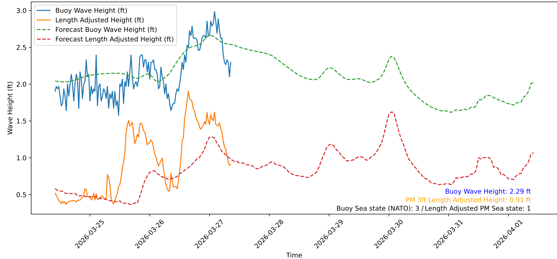
Wave Heights over Time for Red Beach at 2026-03-27 09:30:47
