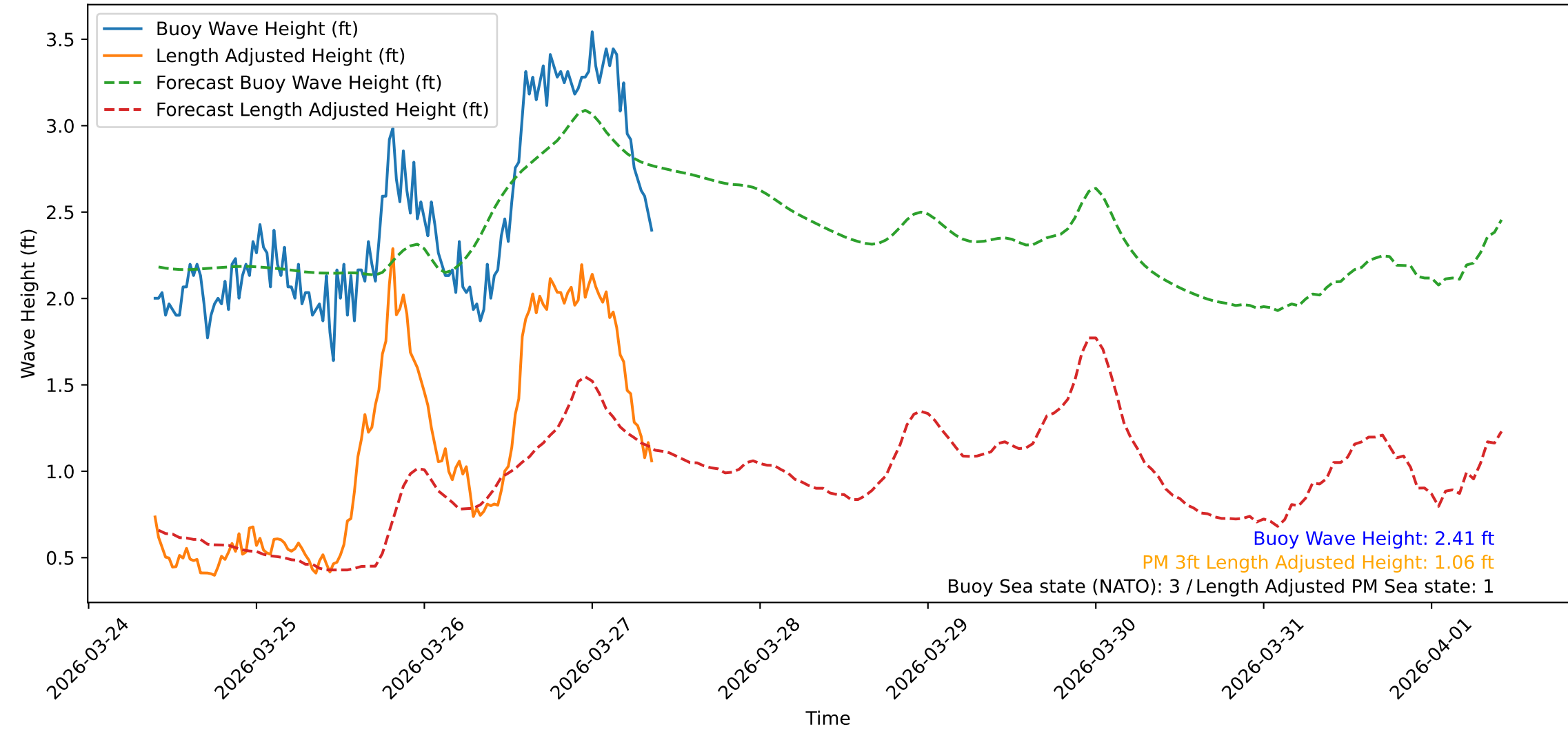
Wave Heights over Time for Green Beach at 2026-03-27 09:31:10
