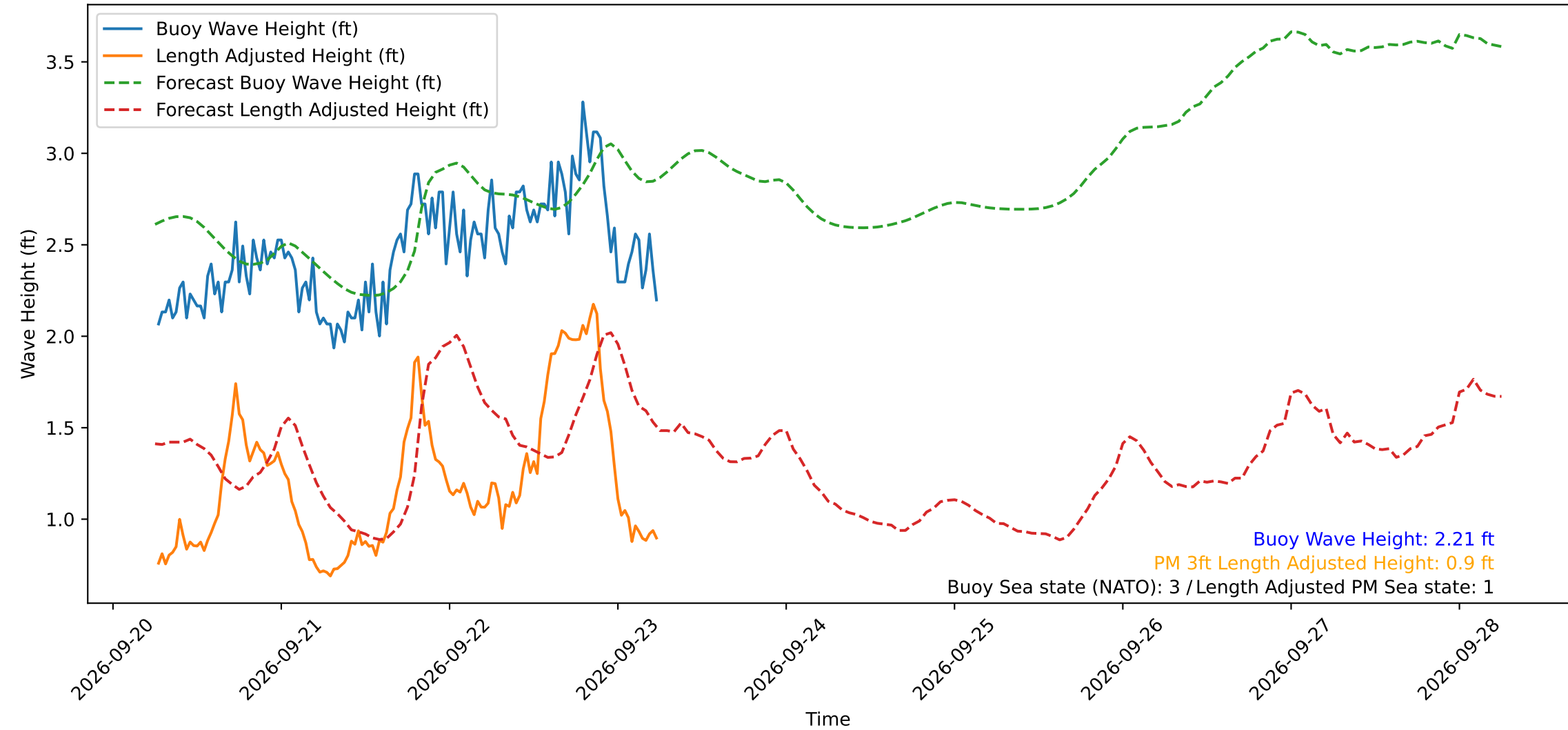
Wave Heights over Time for Red Beach at 2026-09-23 06:10:50
