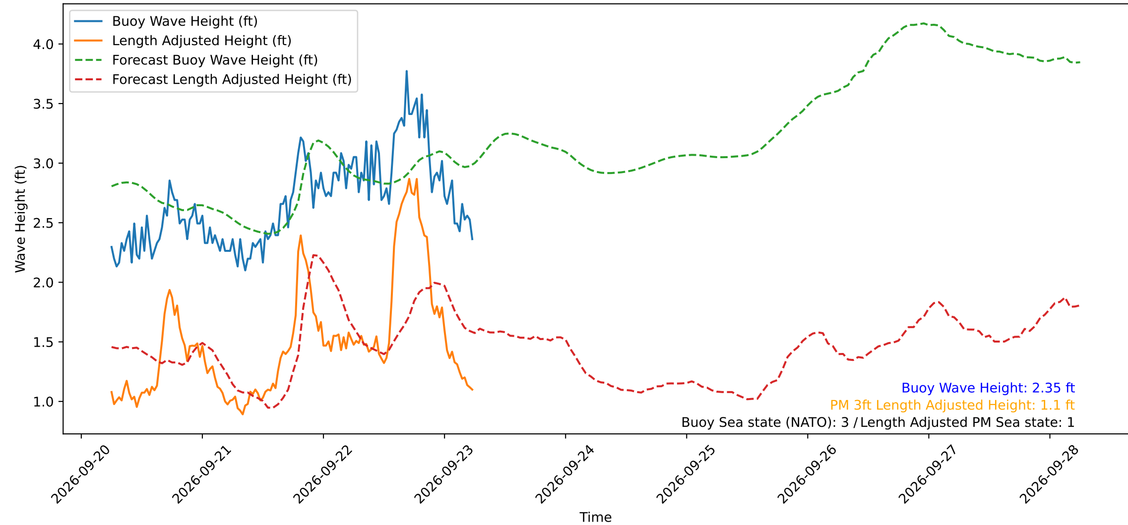
Wave Heights over Time for Oceanside Harbor at 2026-09-23 06:10:30
