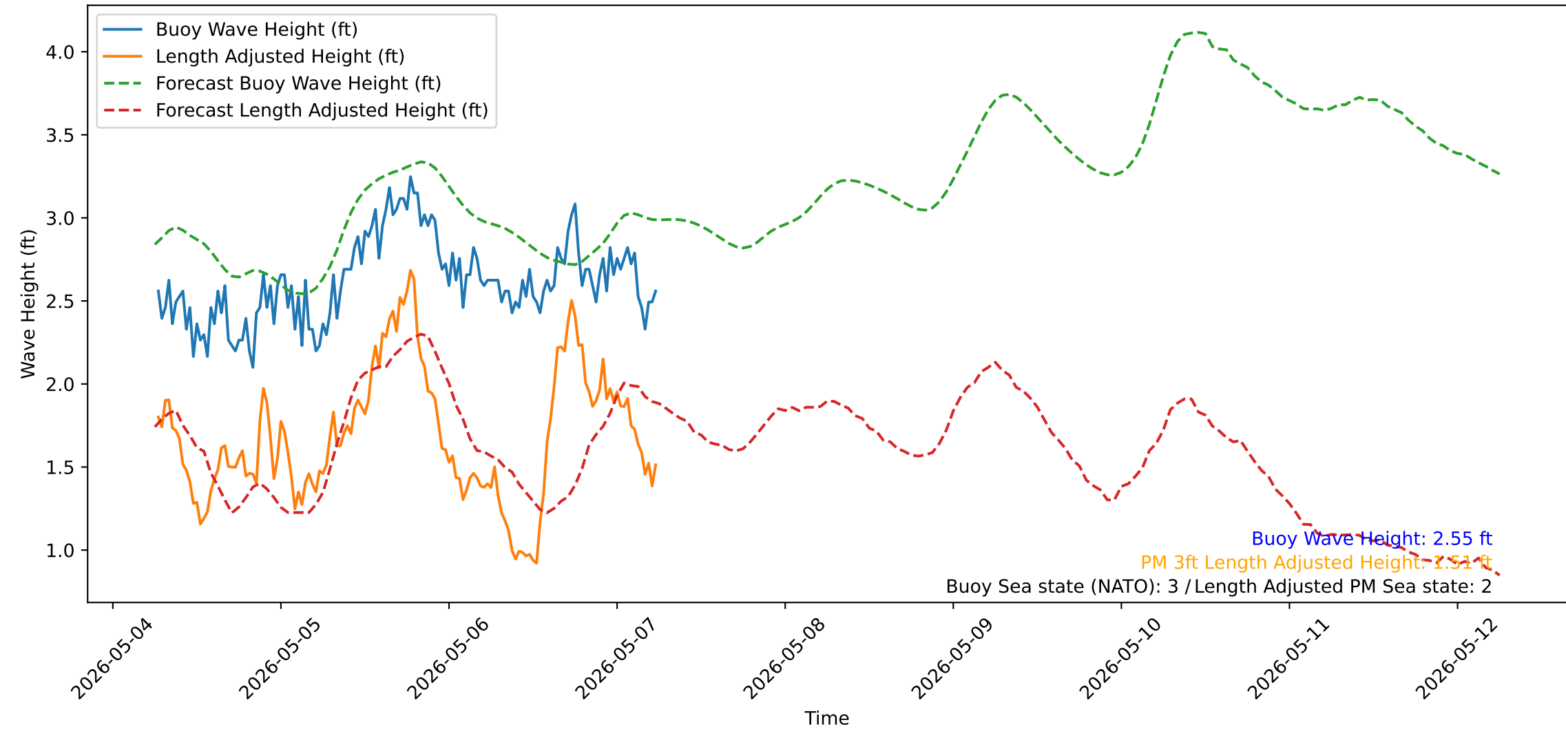
Wave Heights over Time for Oceanside Harbor at 2026-05-07 06:20:31
