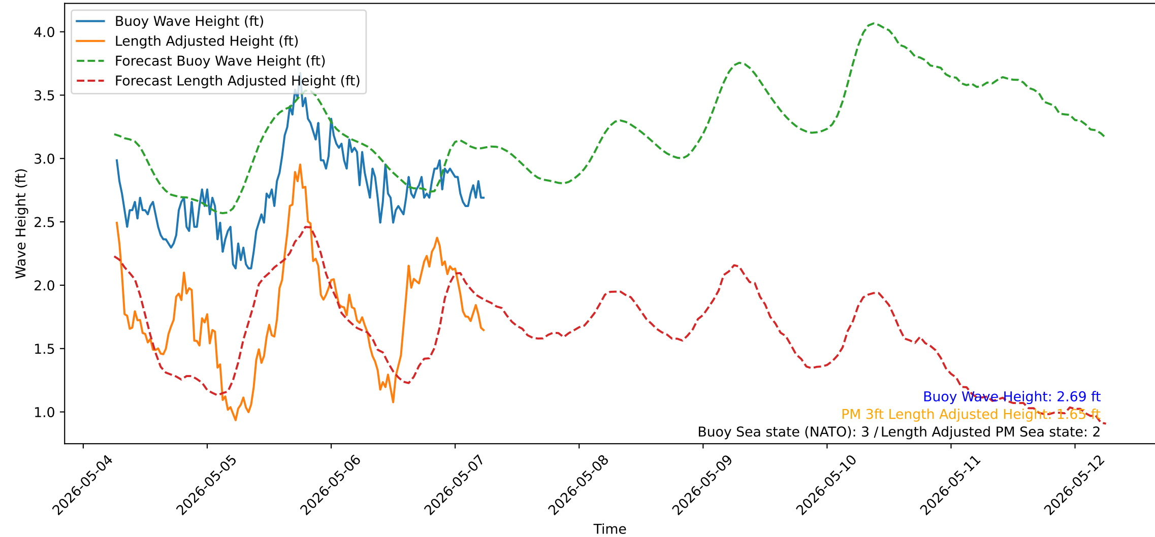
Wave Heights over Time for Green Beach at 2026-05-07 06:21:13
