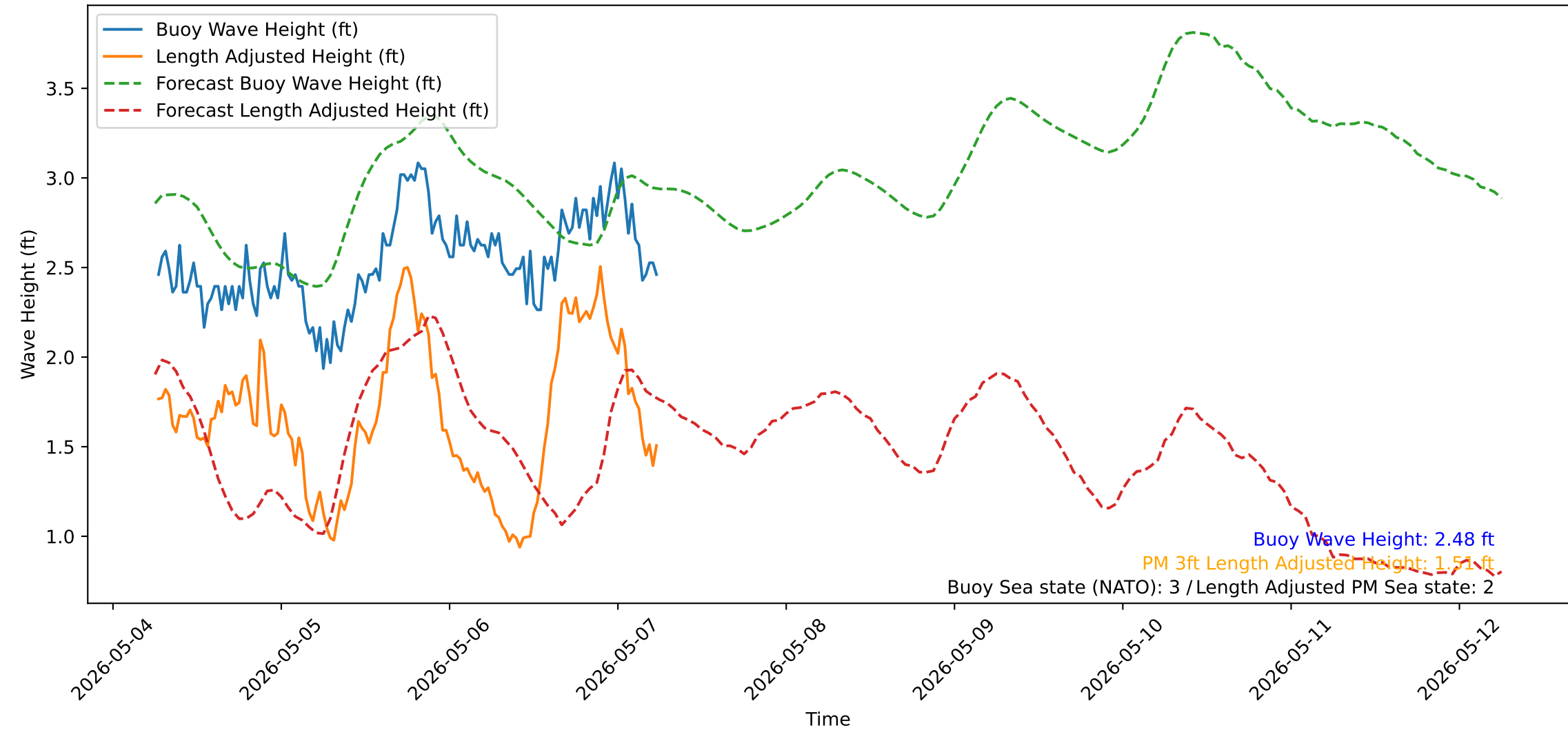
Wave Heights over Time for Red Beach at 2026-05-07 06:20:51
