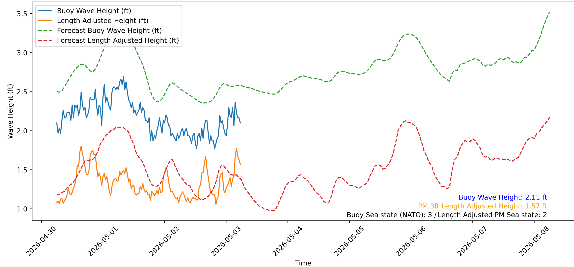
Wave Heights over Time for Oceanside Harbor at 2026-05-03 06:00:31
