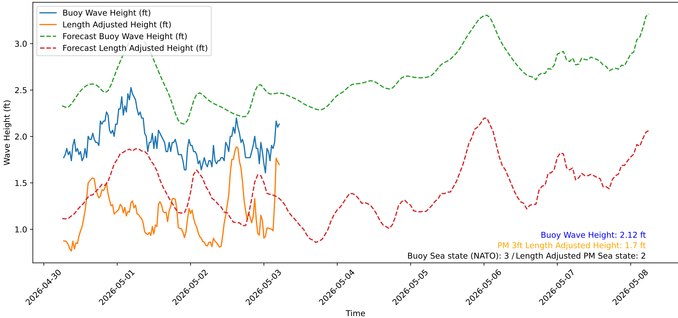
Wave Heights over Time for Red Beach at 2026-05-03 06:00:50
