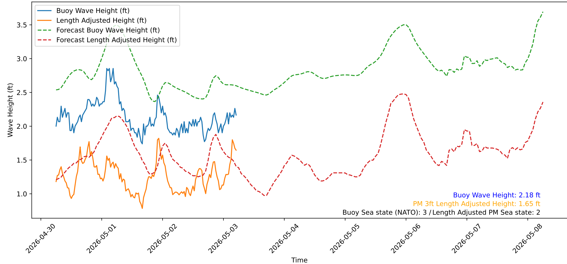
Wave Heights over Time for Green Beach at 2026-05-03 06:01:13
