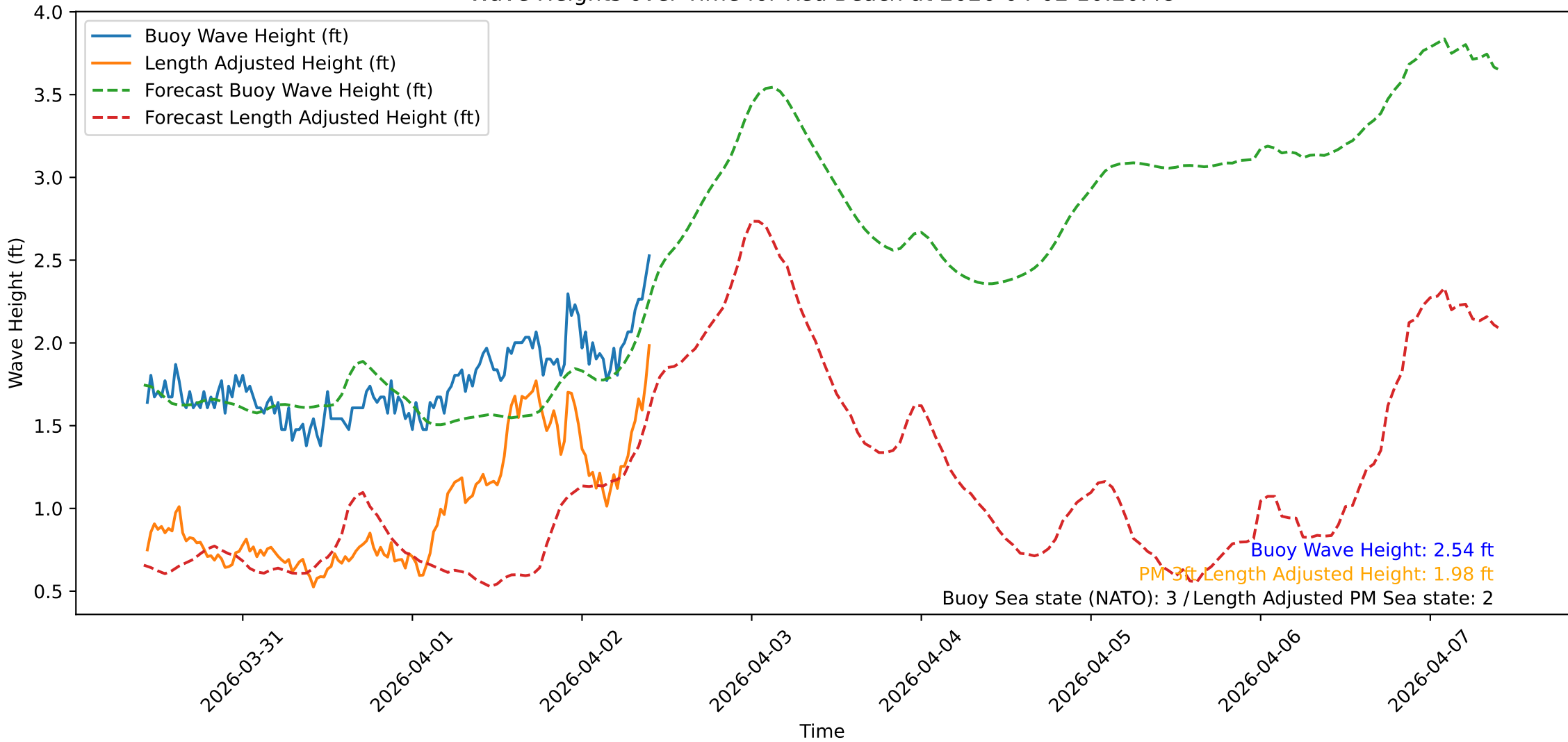
Wave Heights over Time for Red Beach at 2026-04-02 10:20:48
