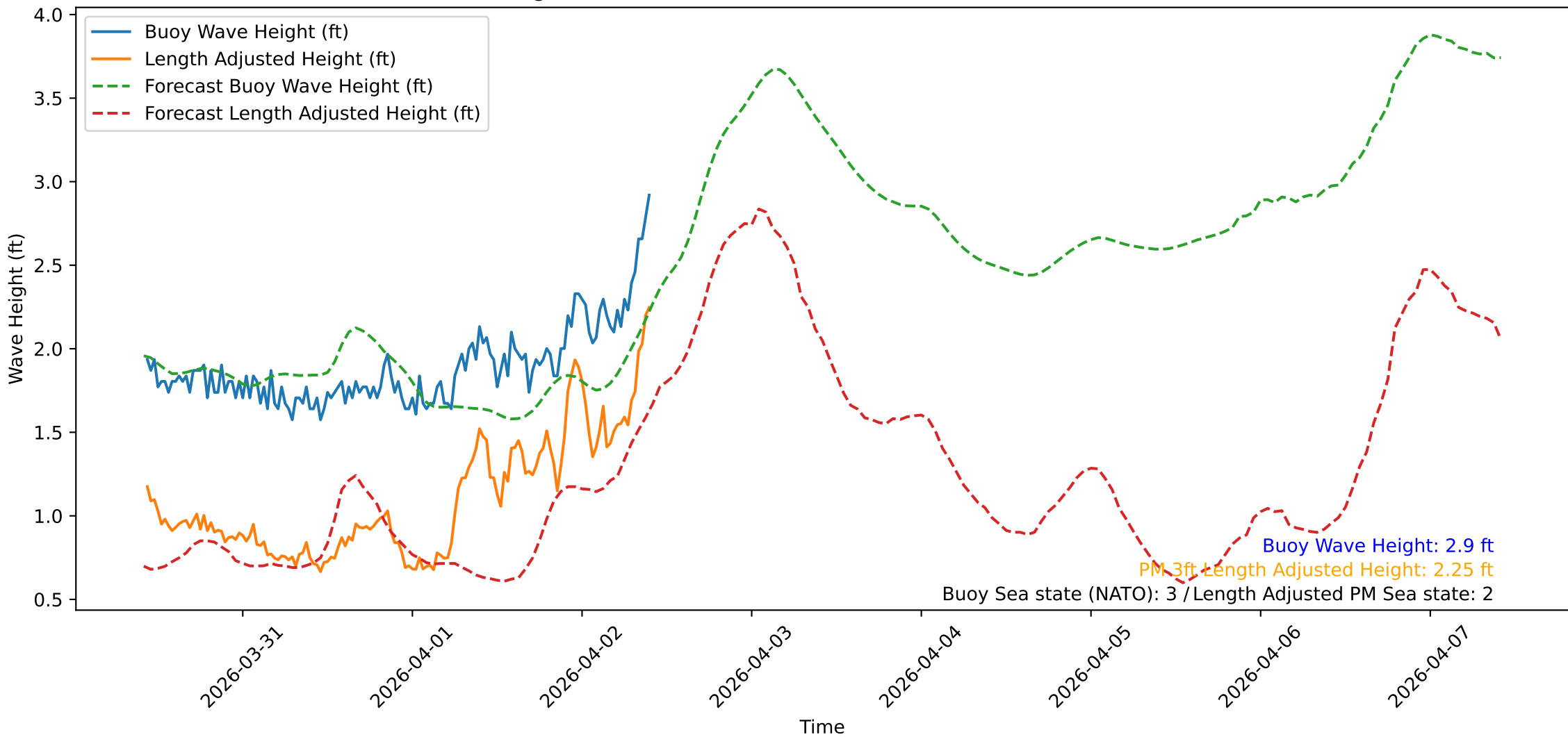
Wave Heights over Time for Oceanside Harbor at 2026-04-02 10:20:31
