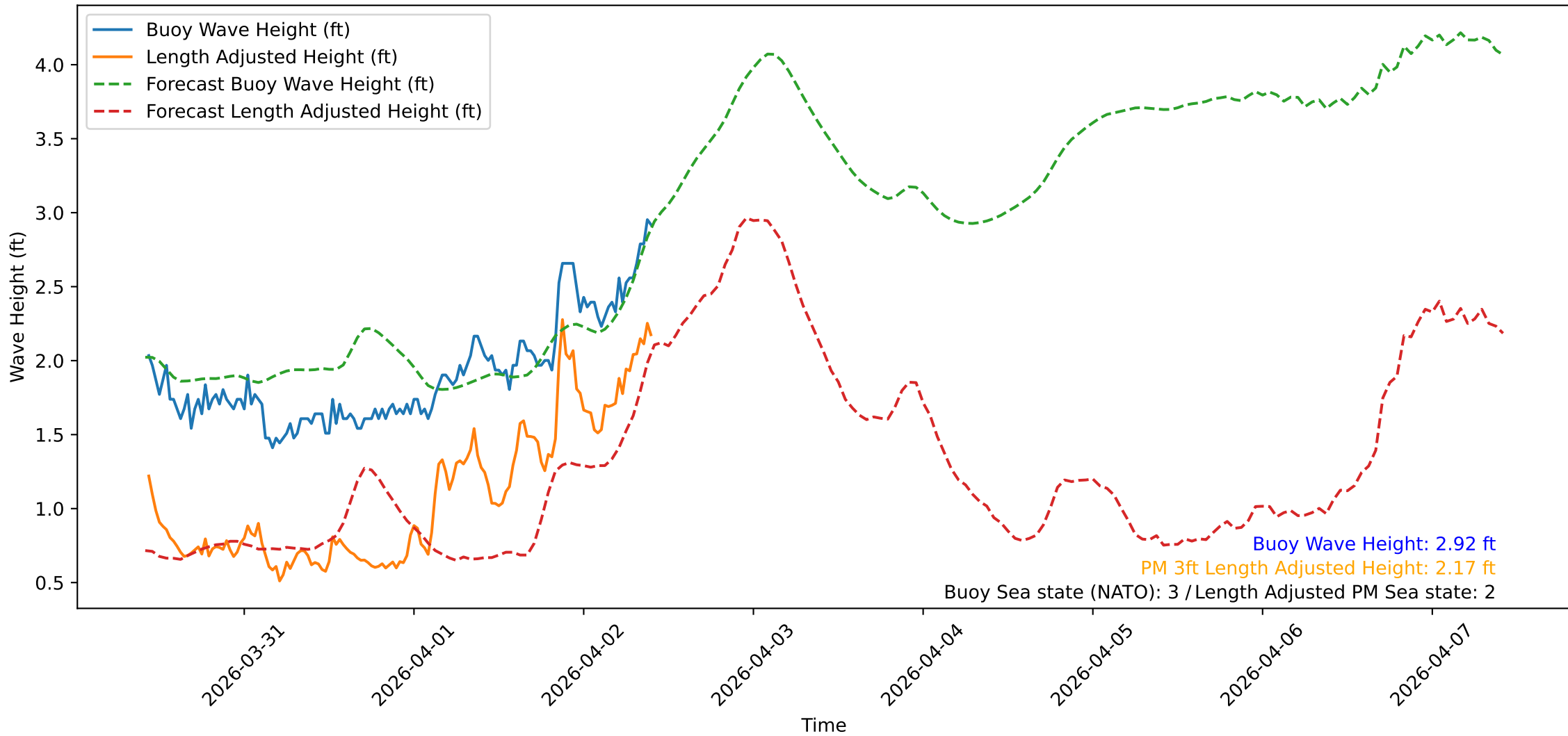
Wave Heights over Time for Green Beach at 2026-04-02 10:21:11
