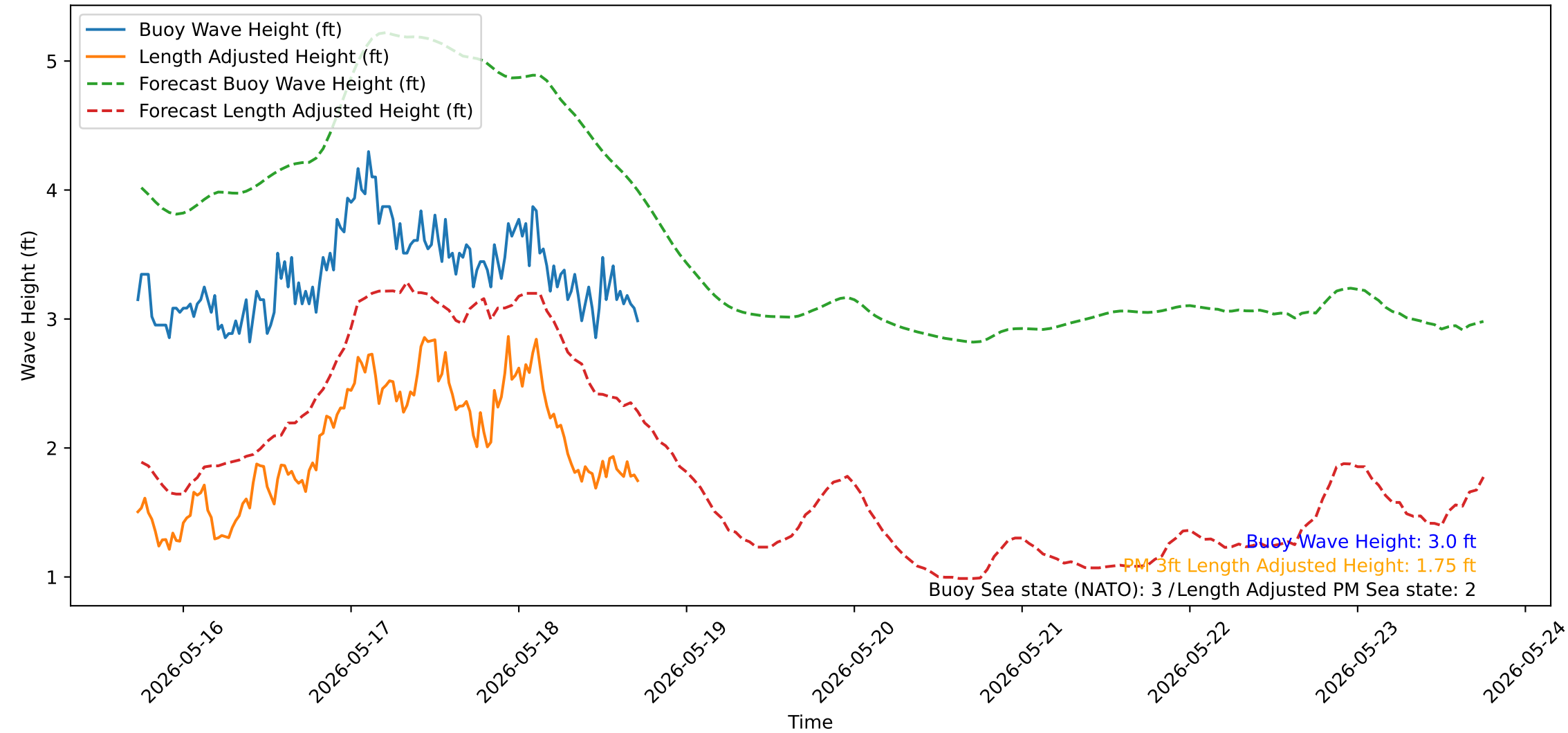
Wave Heights over Time for Oceanside Harbor at 2026-05-18 17:40:31
