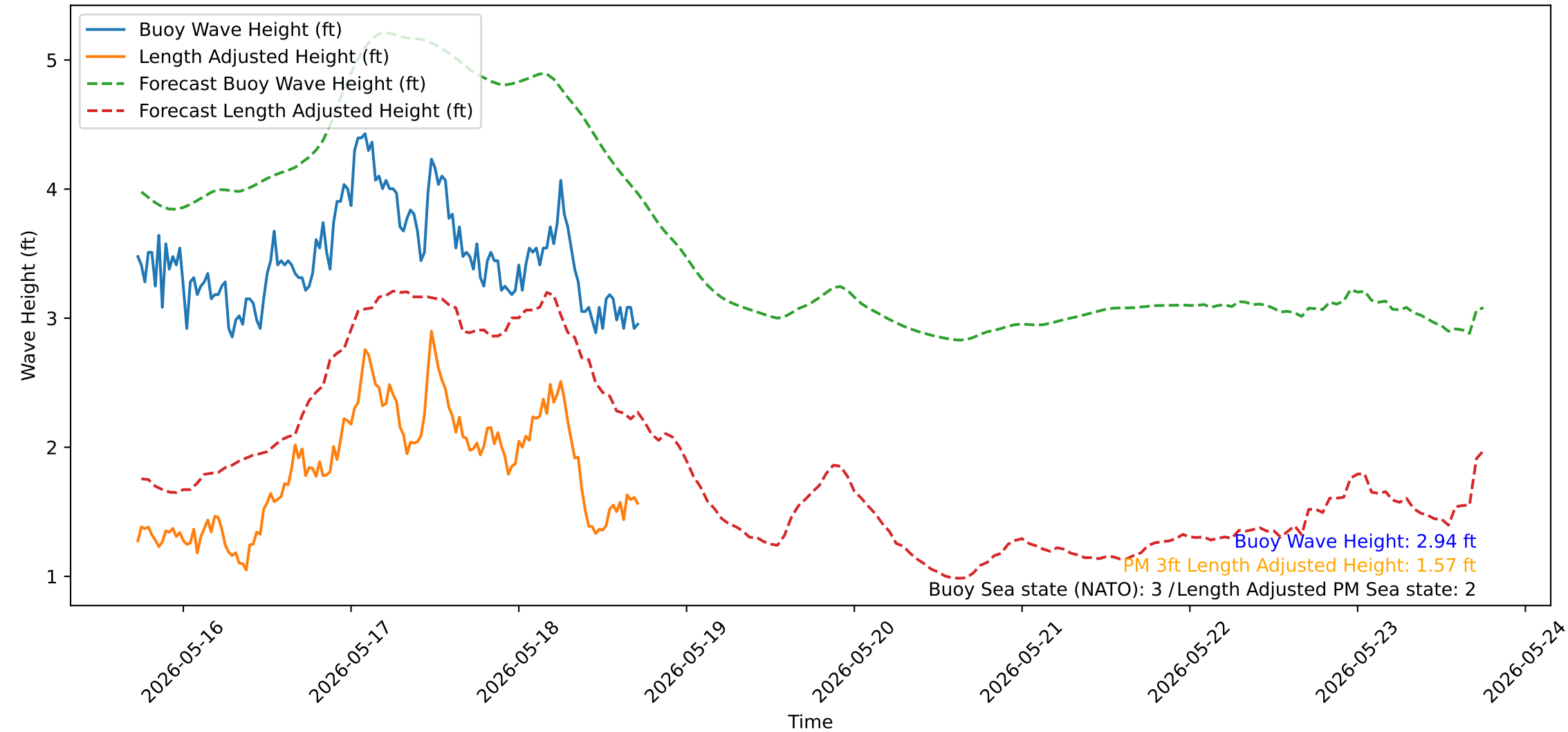
Wave Heights over Time for Green Beach at 2026-05-18 17:41:14
