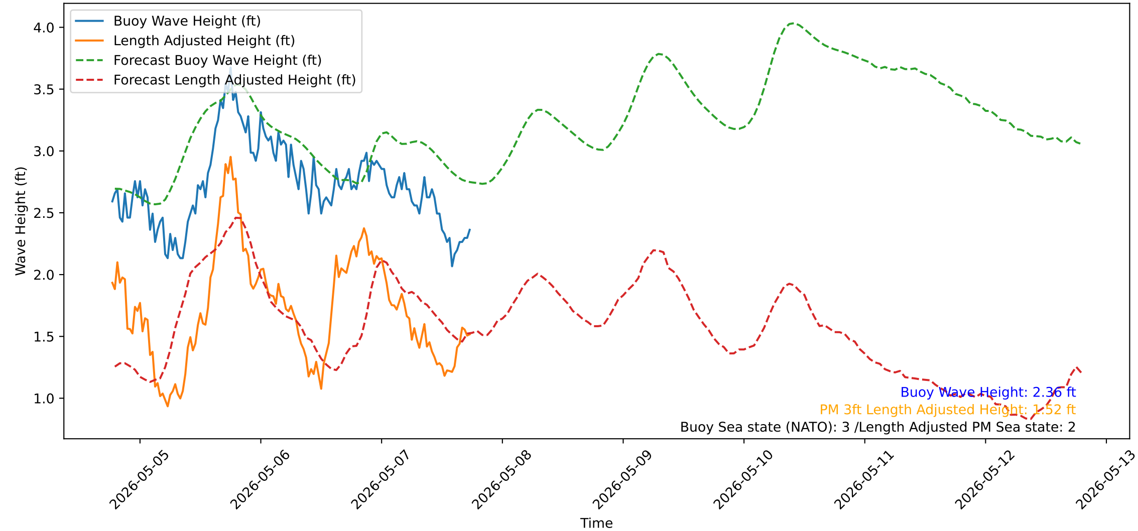
Wave Heights over Time for Green Beach at 2026-05-07 18:31:14
