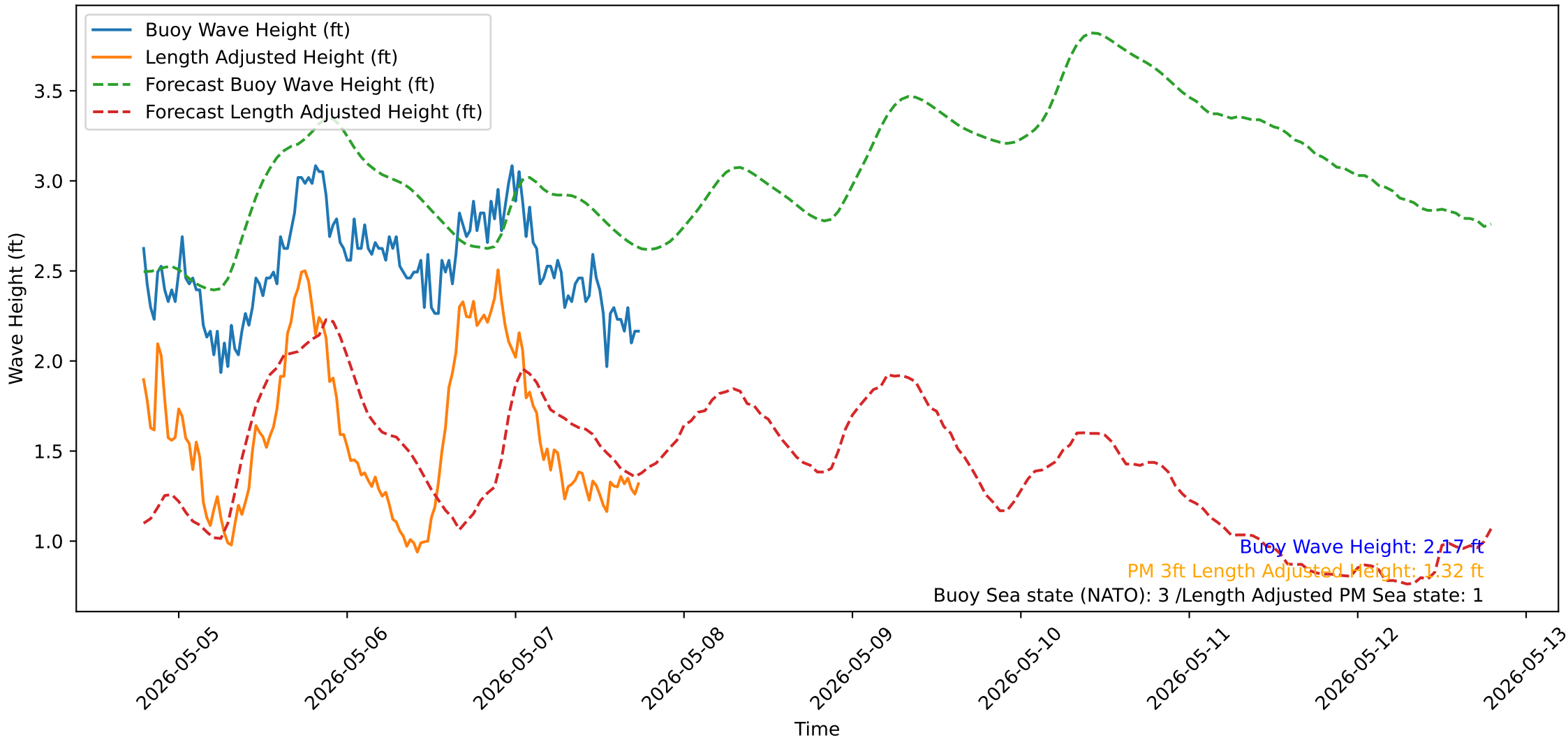
Wave Heights over Time for Red Beach at 2026-05-07 18:30:51
