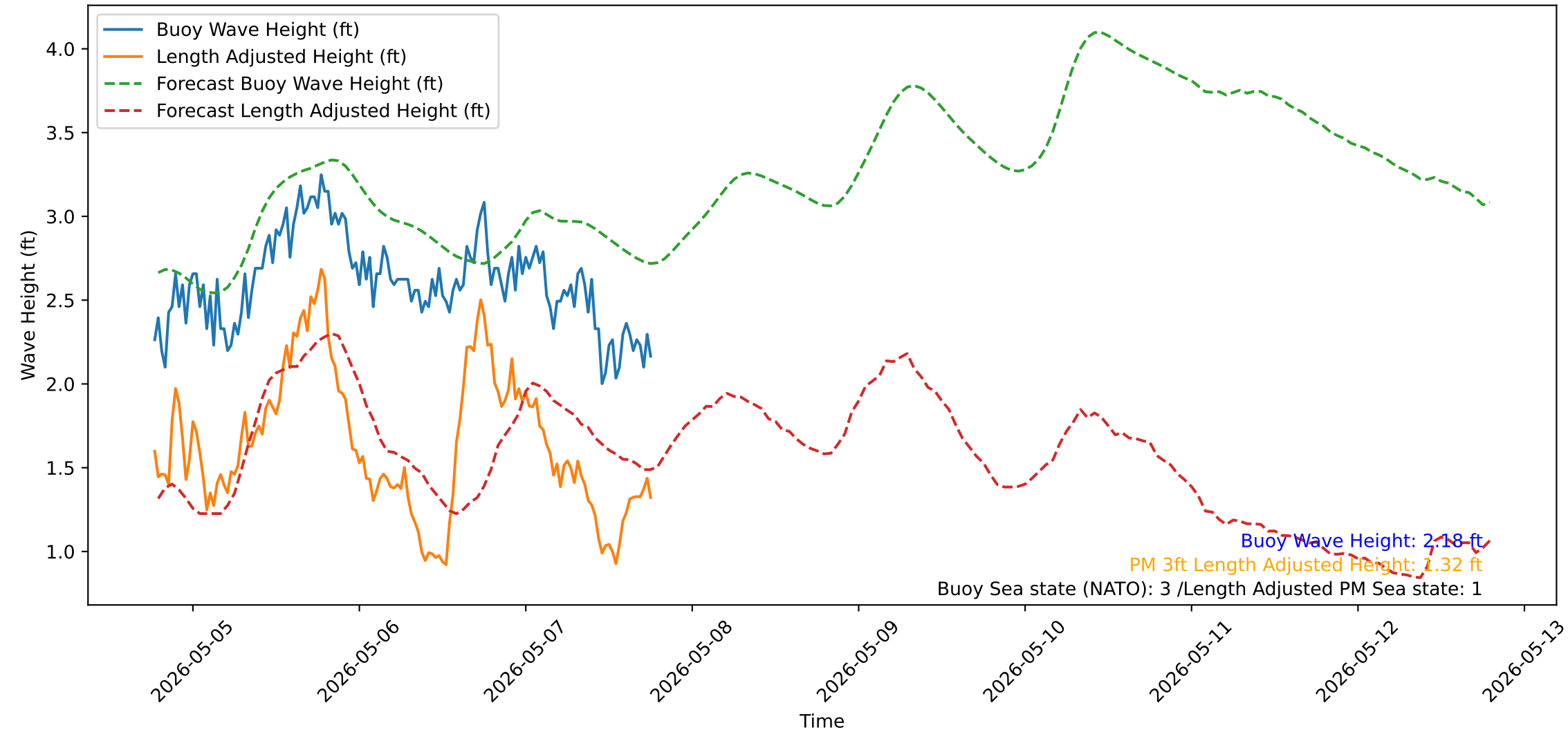
Wave Heights over Time for Oceanside Harbor at 2026-05-07 18:30:32
