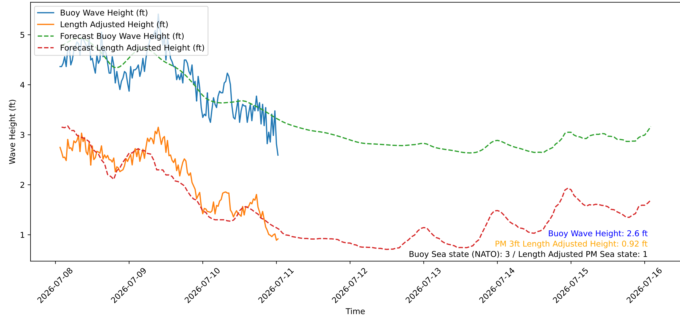
Wave Heights over Time for Oceanside Harbor at 2026-07-11 01:30:27
