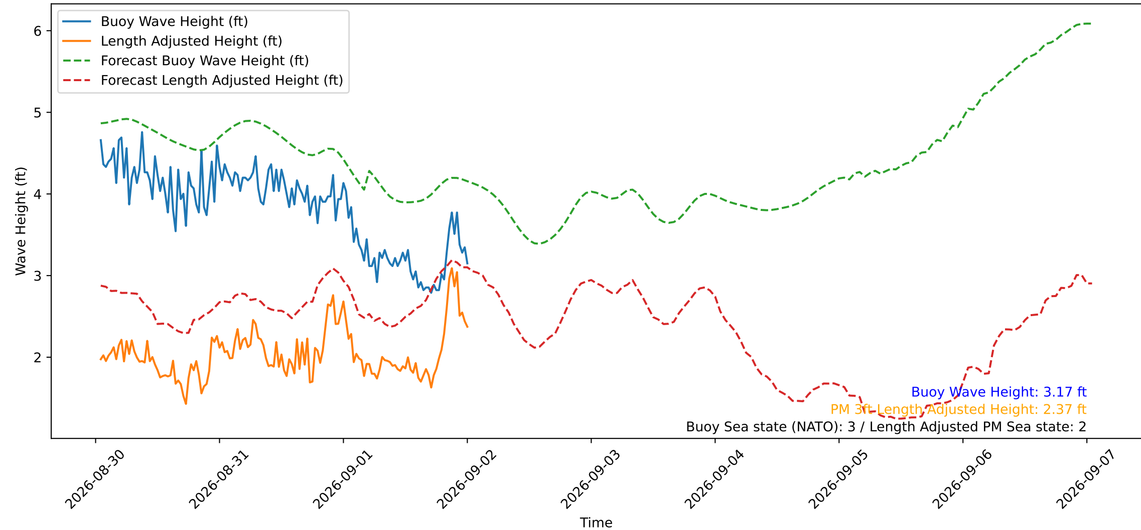
Wave Heights over Time for Green Beach at 2026-09-02 00:41:12
