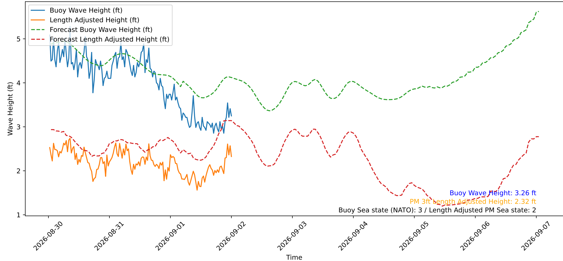
Wave Heights over Time for Oceanside Harbor at 2026-09-02 00:40:30
