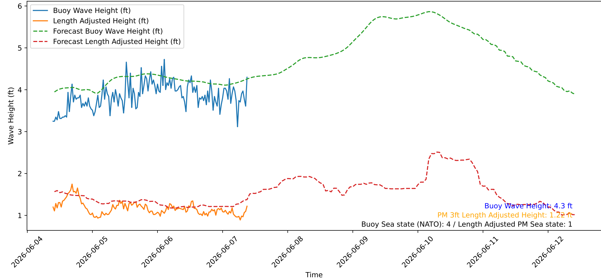
Wave Heights over Time for Green Beach at 2026-06-07 09:41:08
