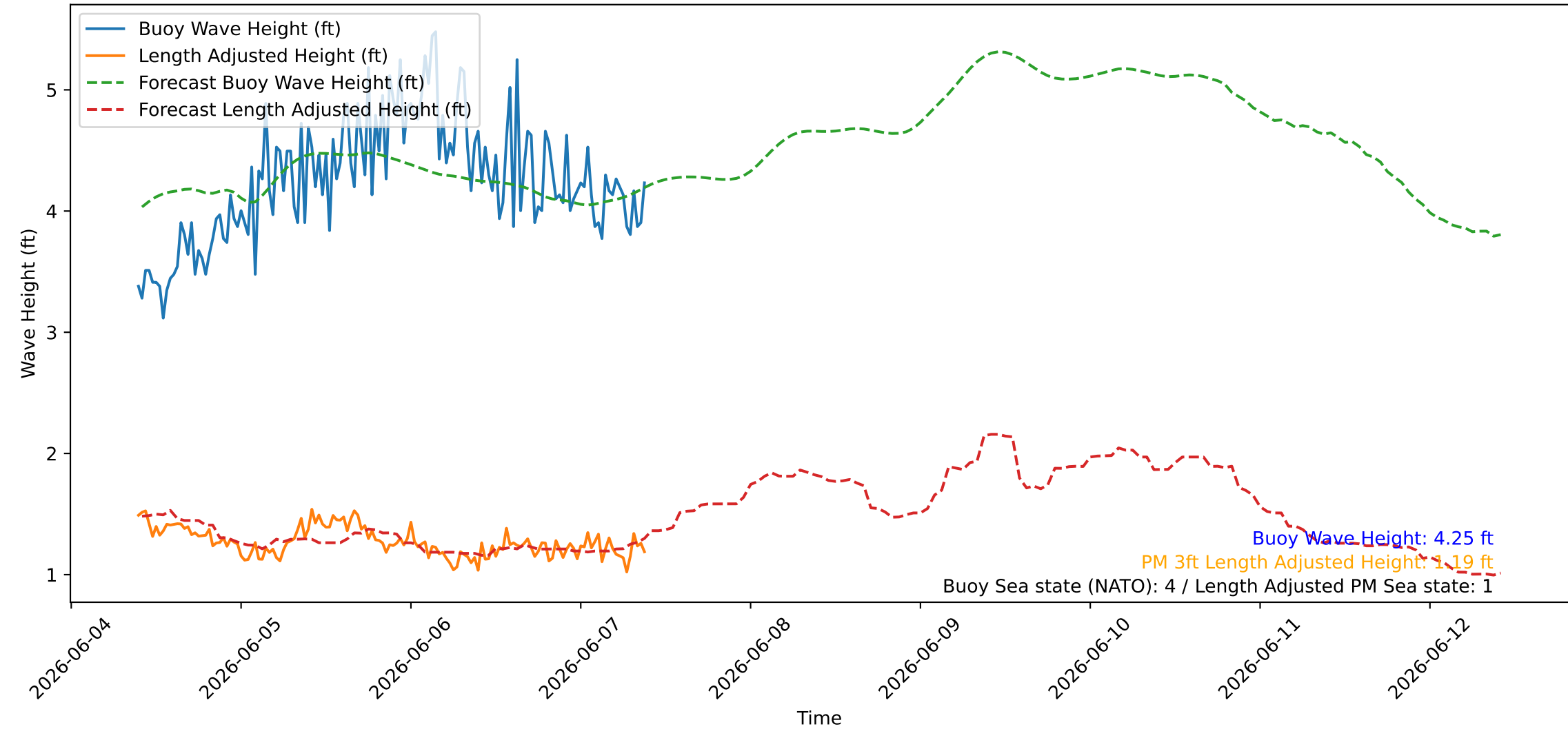
Wave Heights over Time for Oceanside Harbor at 2026-06-07 09:40:26
