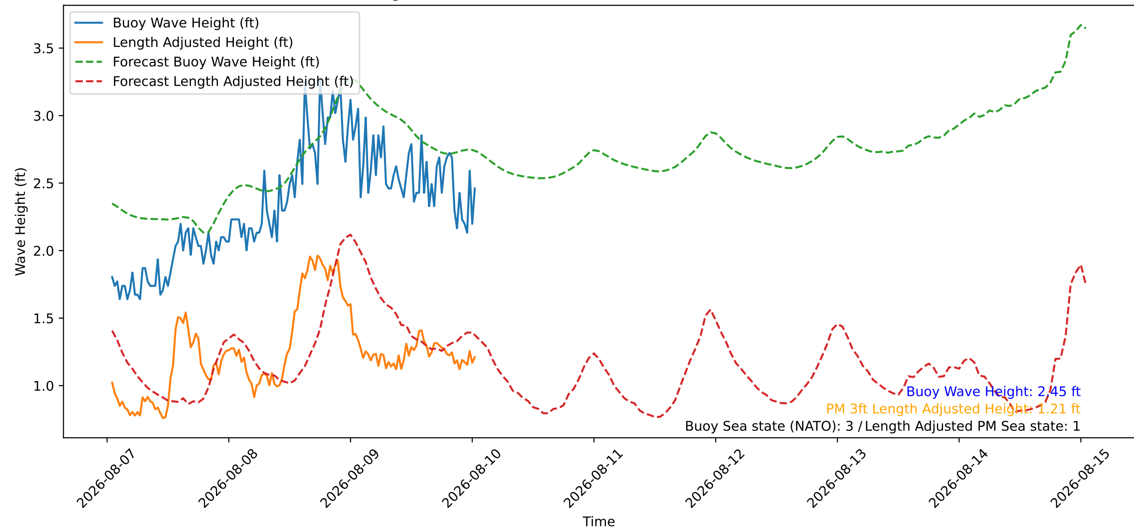
Wave Heights over Time for Oceanside Harbor at 2026-08-10 01:00:26
