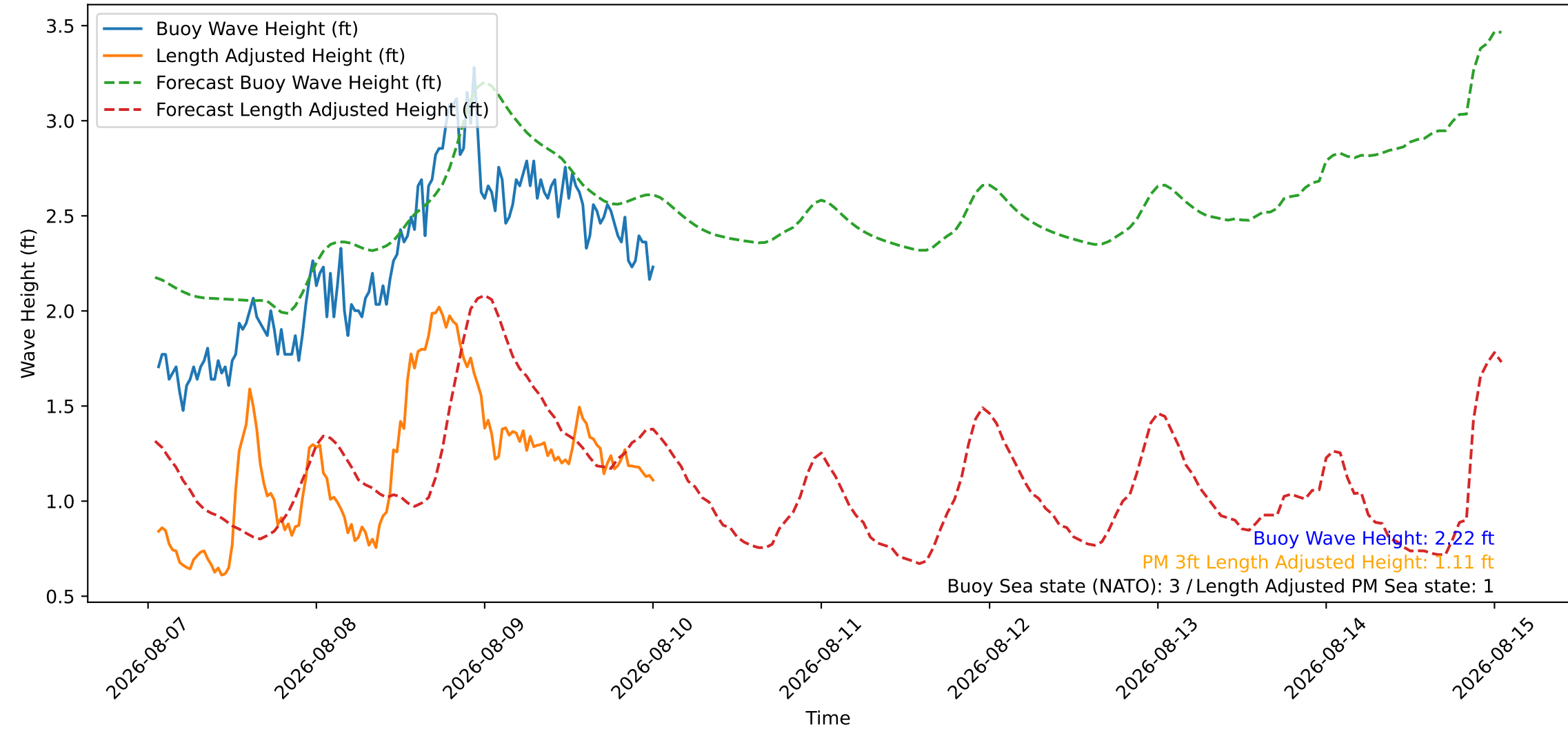
Wave Heights over Time for Red Beach at 2026-08-10 01:00:46
