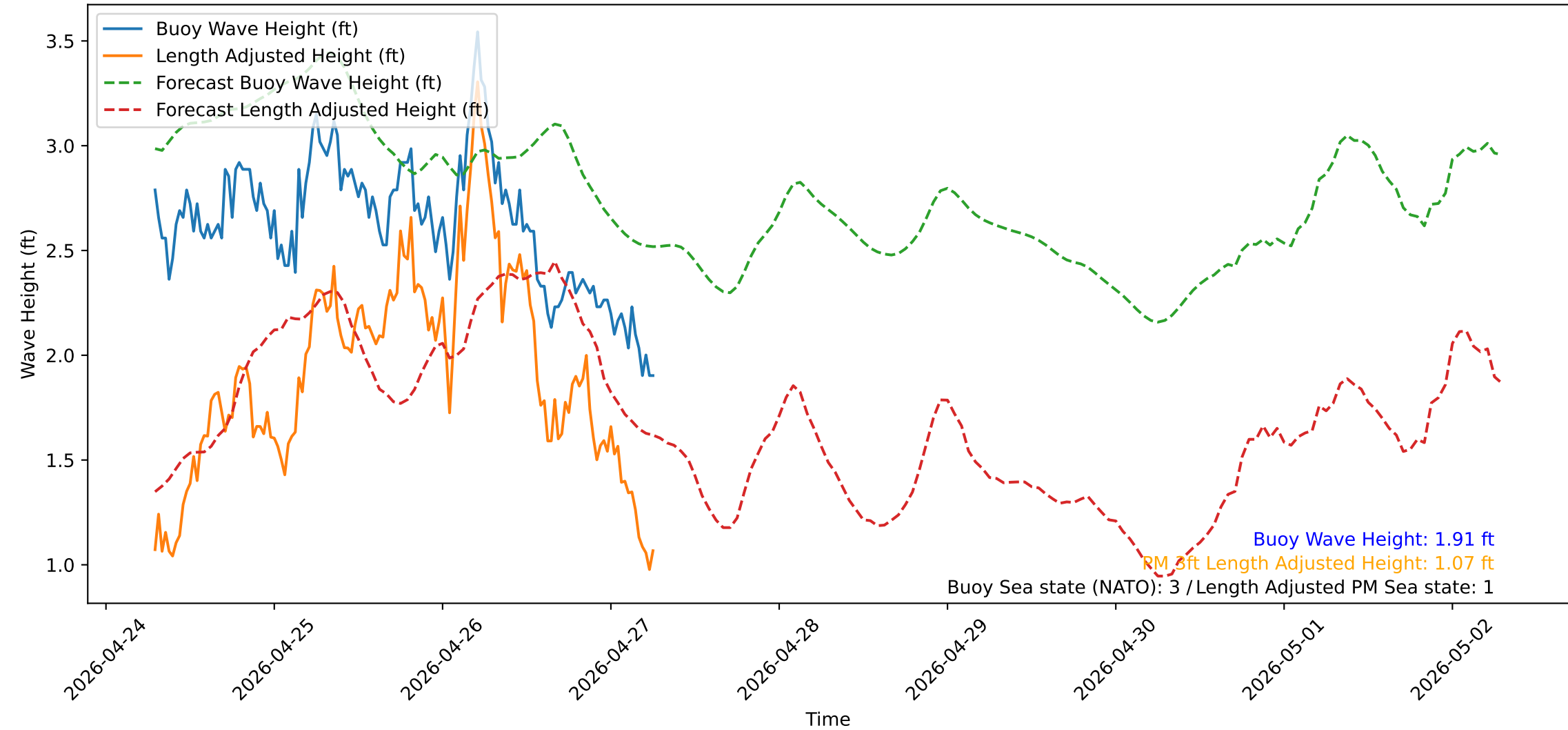
Wave Heights over Time for Red Beach at 2026-04-27 06:40:50
