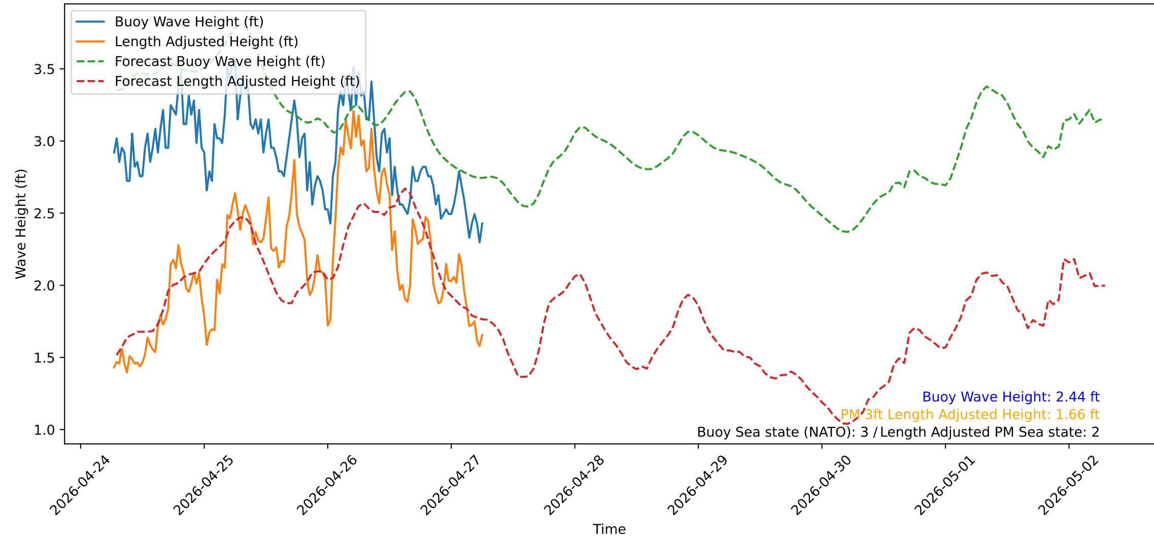
Wave Heights over Time for Green Beach at 2026-04-27 06:41:12
