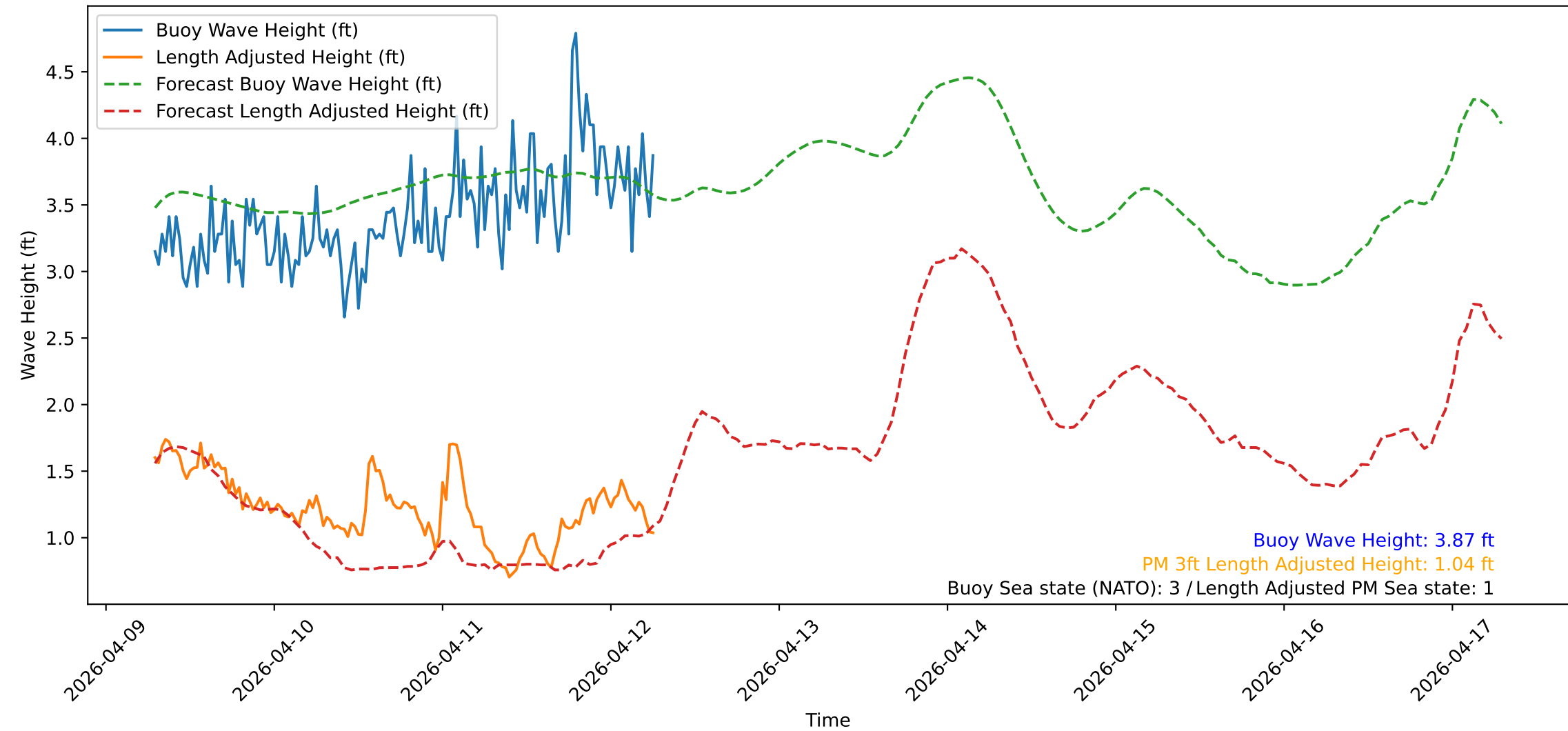
Wave Heights over Time for Oceanside Harbor at 2026-04-12 06:50:31
