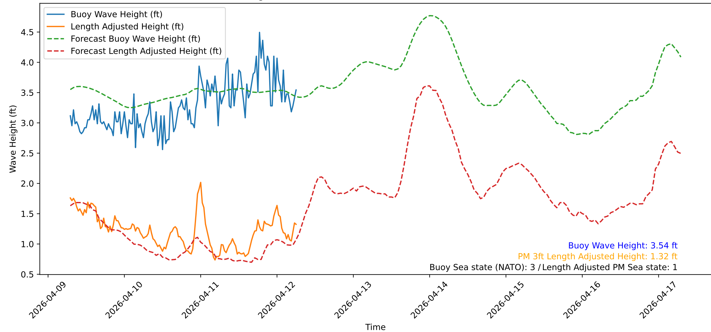
Wave Heights over Time for Green Beach at 2026-04-12 06:51:14
