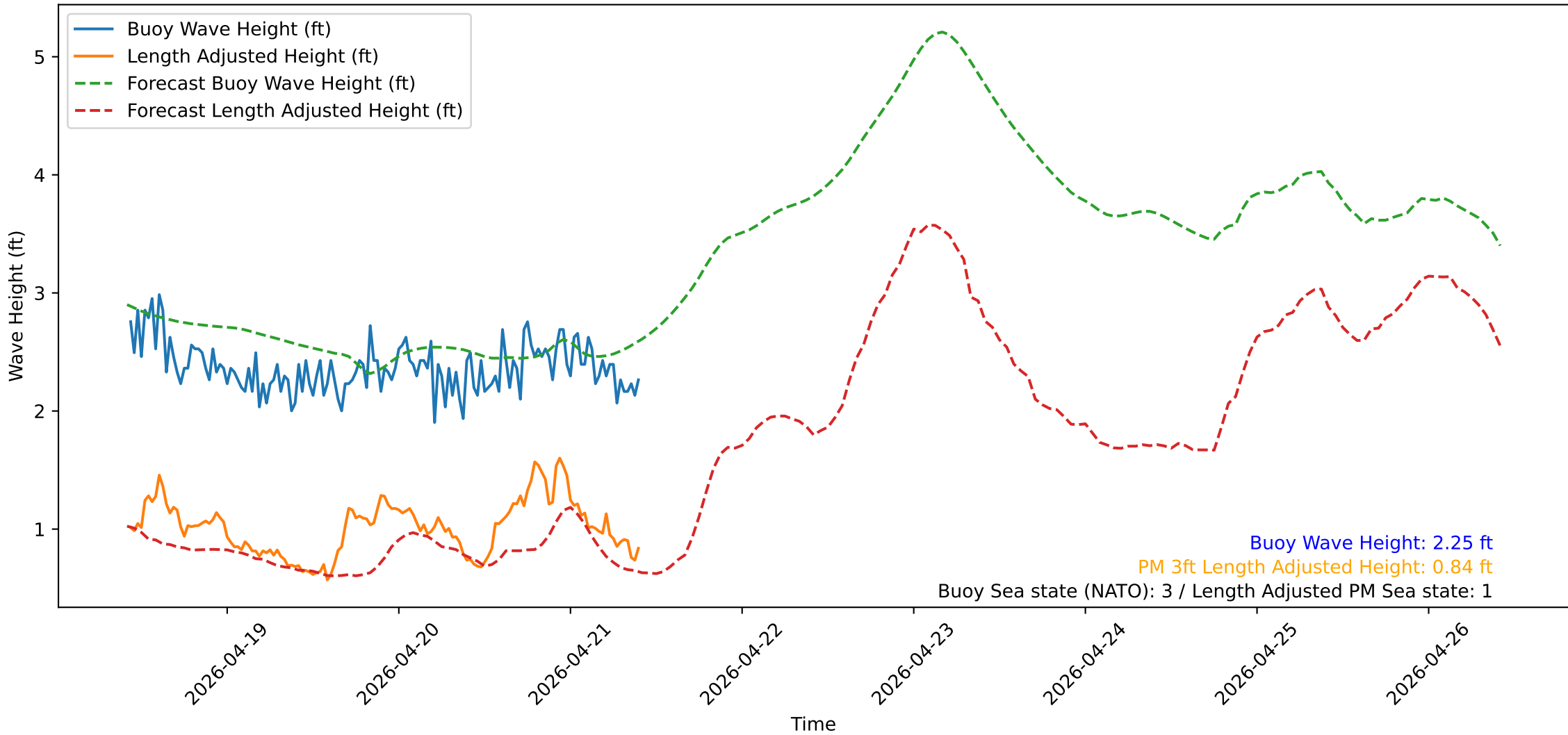
Wave Heights over Time for Oceanside Harbor at 2026-04-21 10:20:32
