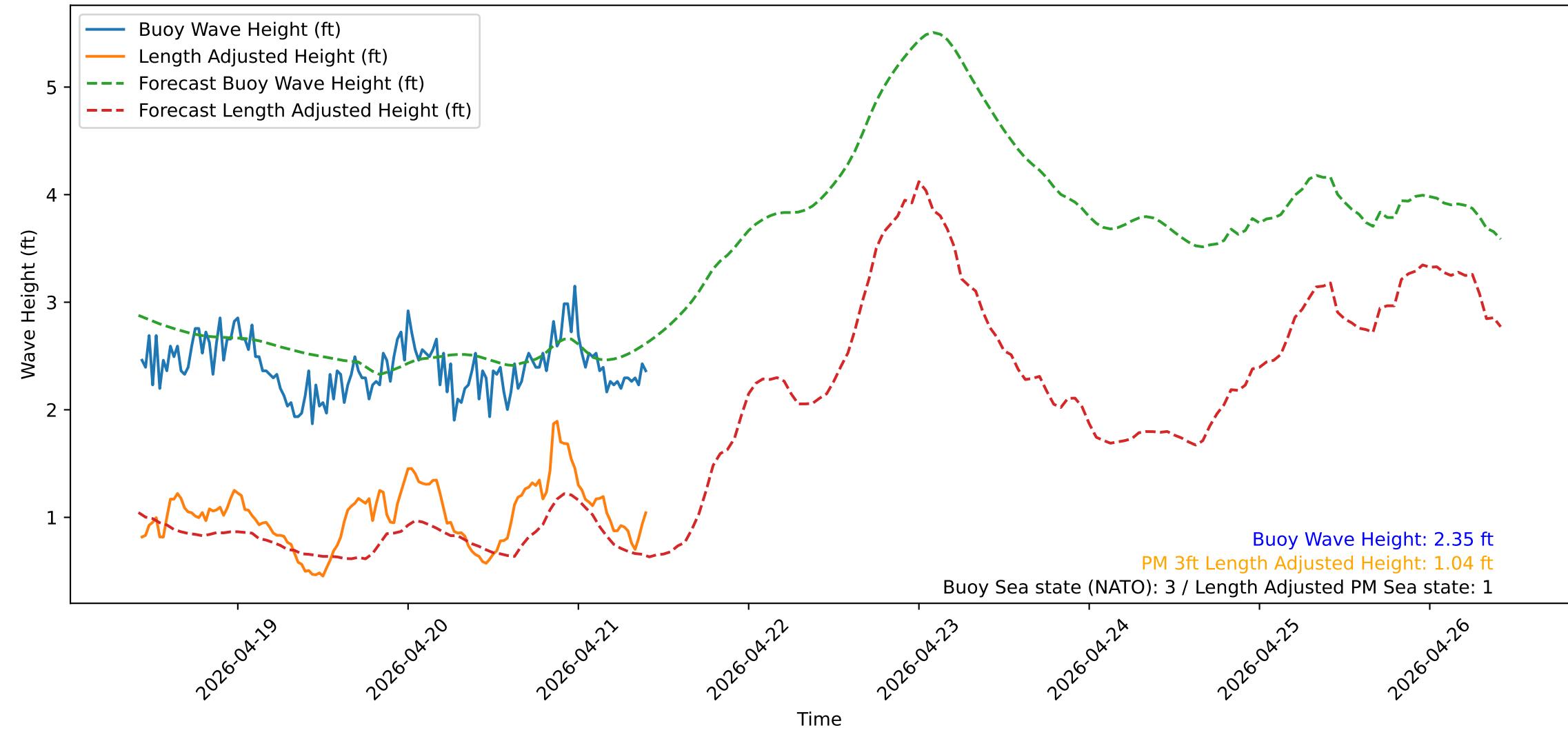
Wave Heights over Time for Green Beach at 2026-04-21 10:21:15
