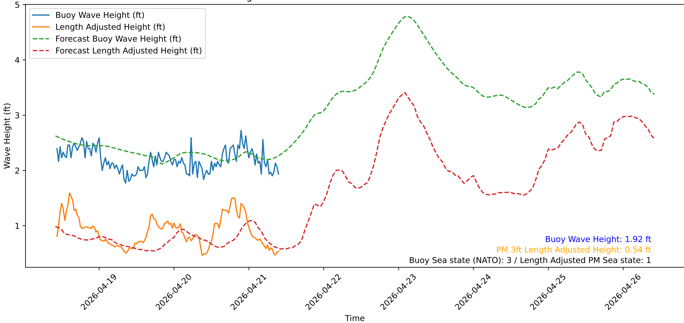
Wave Heights over Time for Red Beach at 2026-04-21 10:20:52
