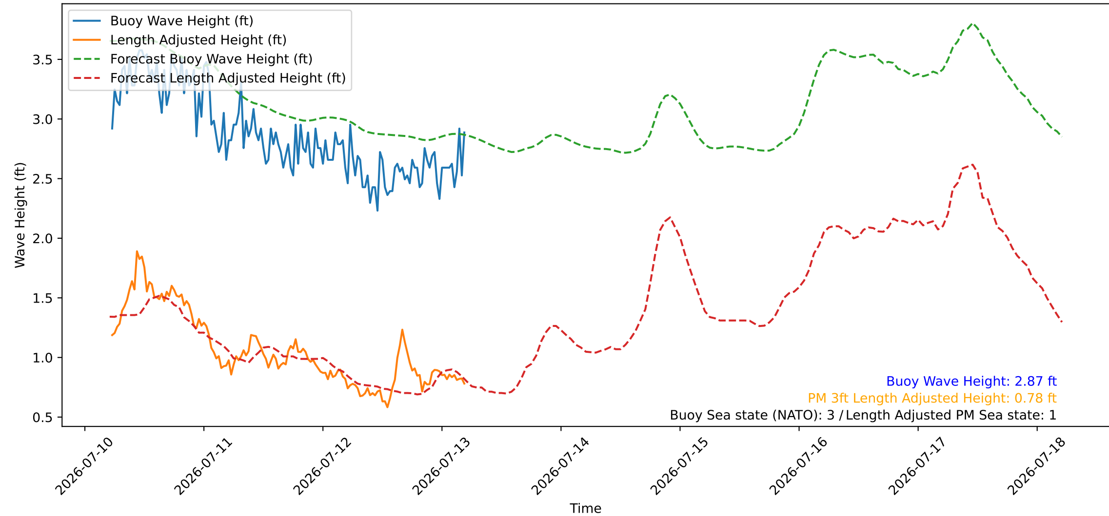
Wave Heights over Time for Green Beach at 2026-07-13 05:21:07
