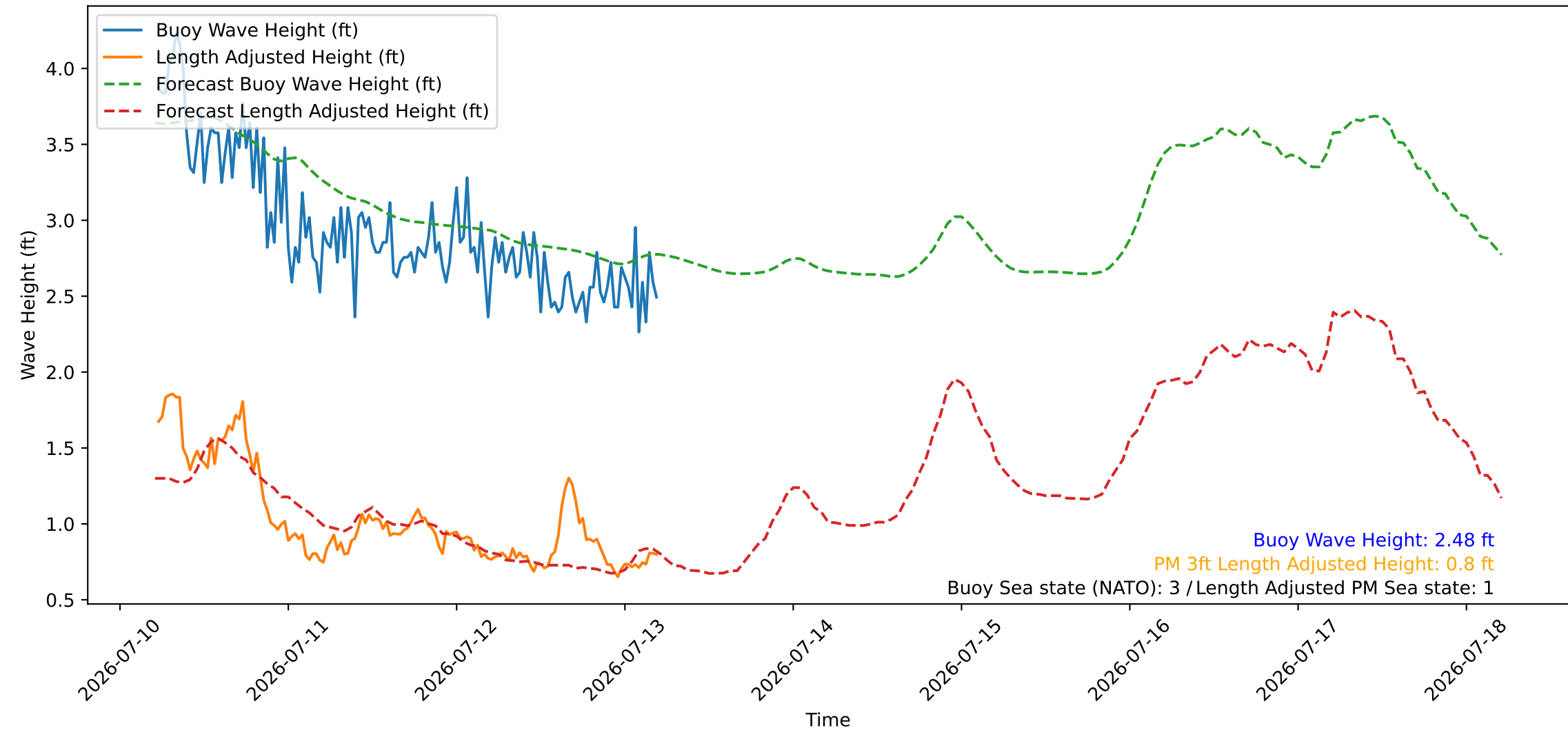
Wave Heights over Time for Oceanside Harbor at 2026-07-13 05:20:25
