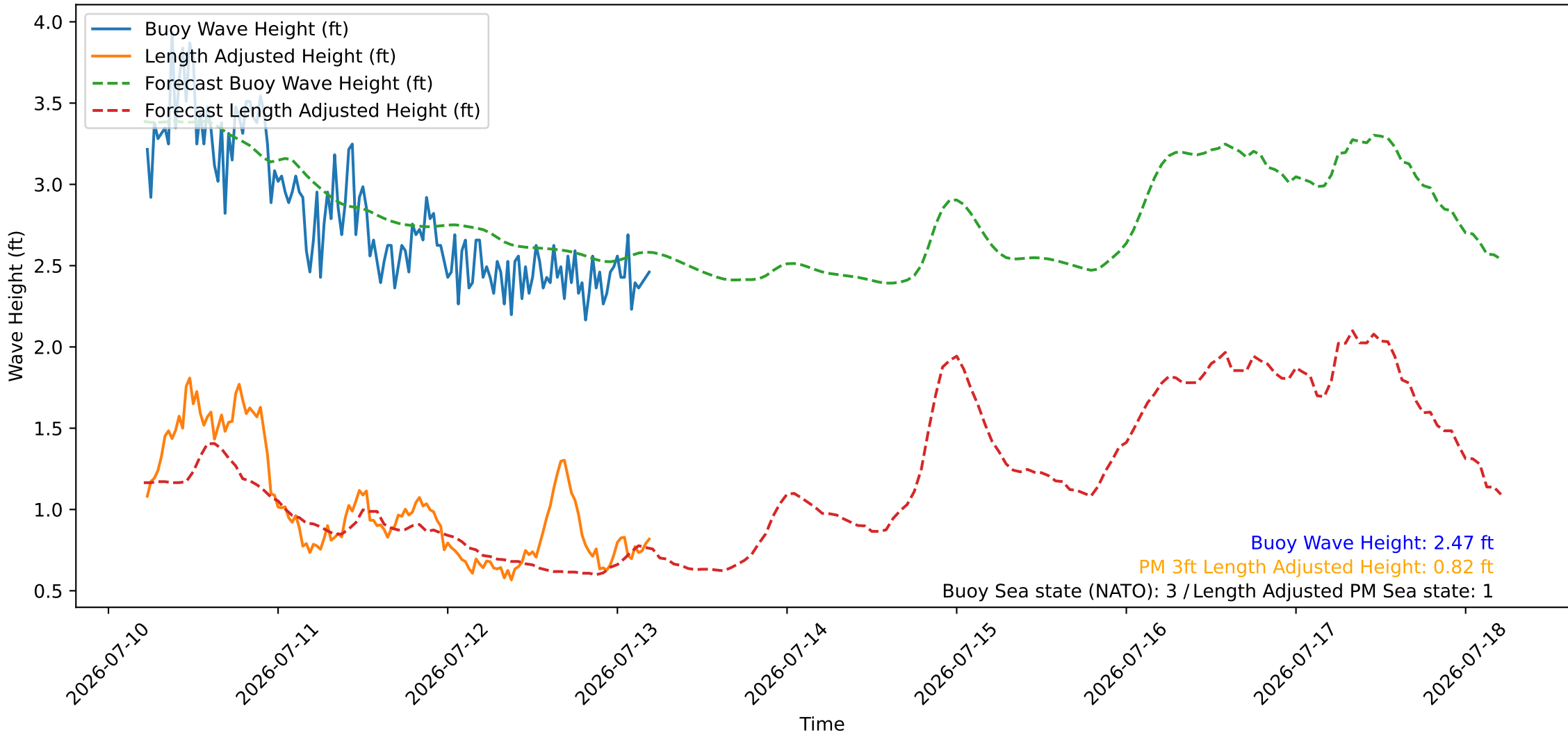
Wave Heights over Time for Red Beach at 2026-07-13 05:20:46
