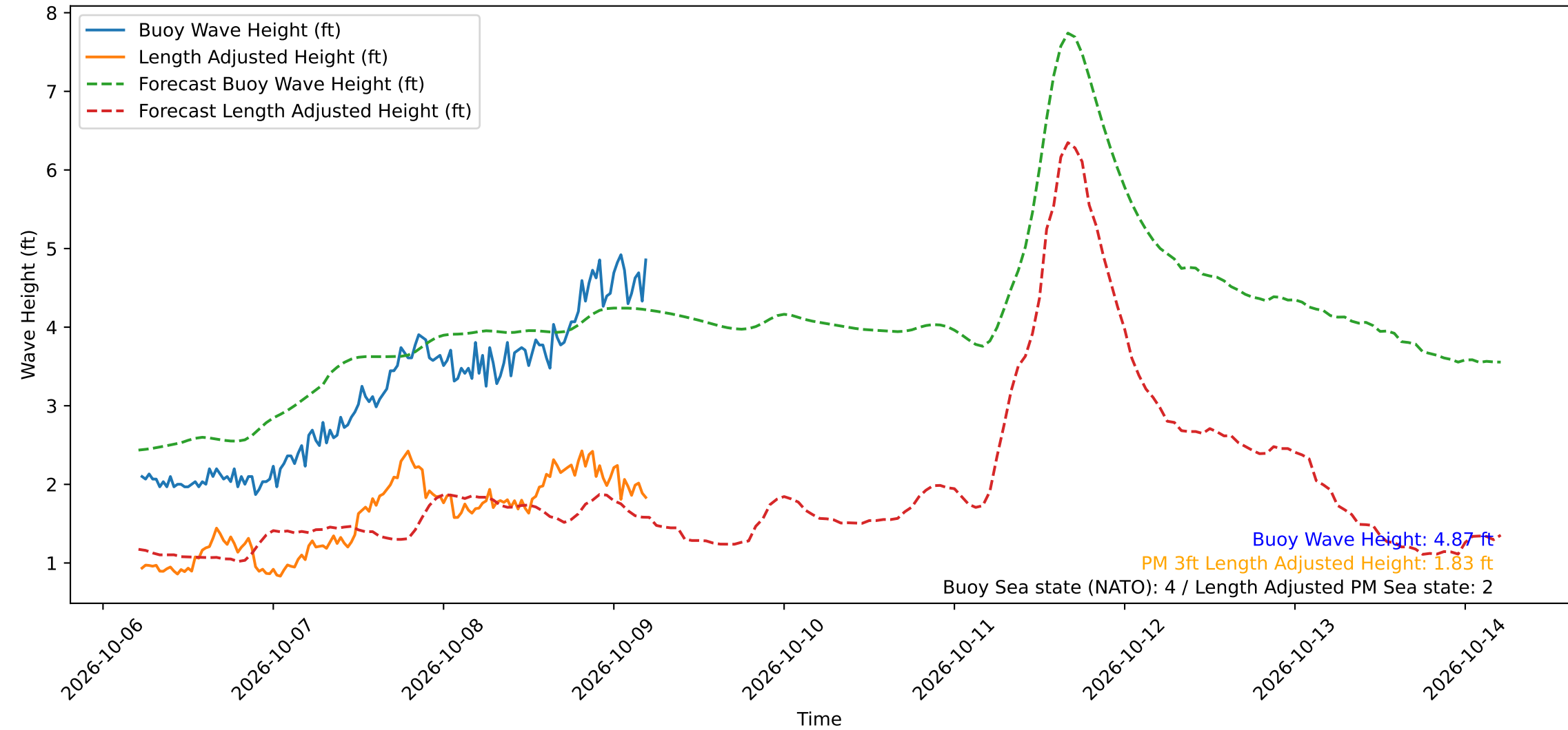
Wave Heights over Time for Red Beach at 2026-10-09 05:20:50
