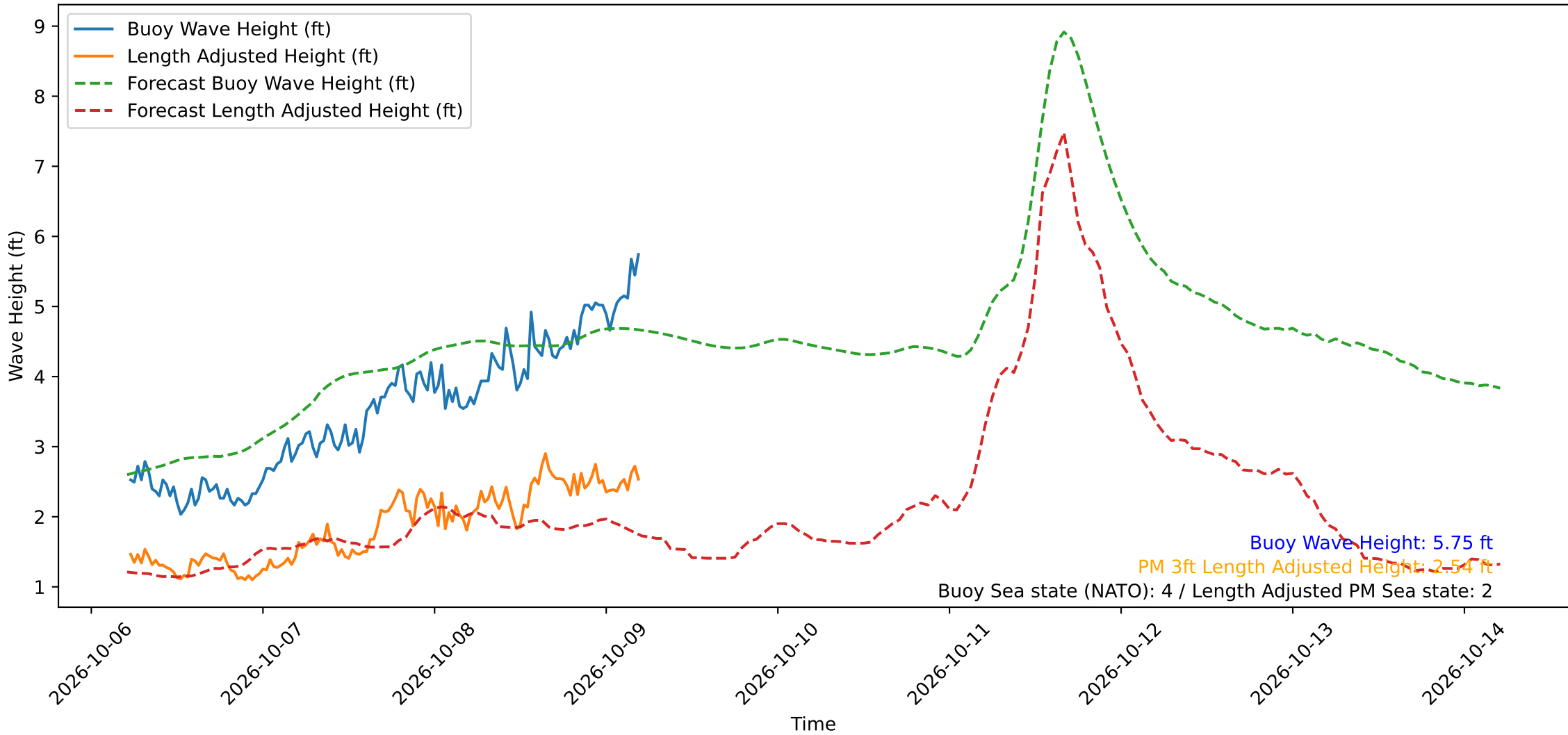
Wave Heights over Time for Oceanside Harbor at 2026-10-09 05:20:30
