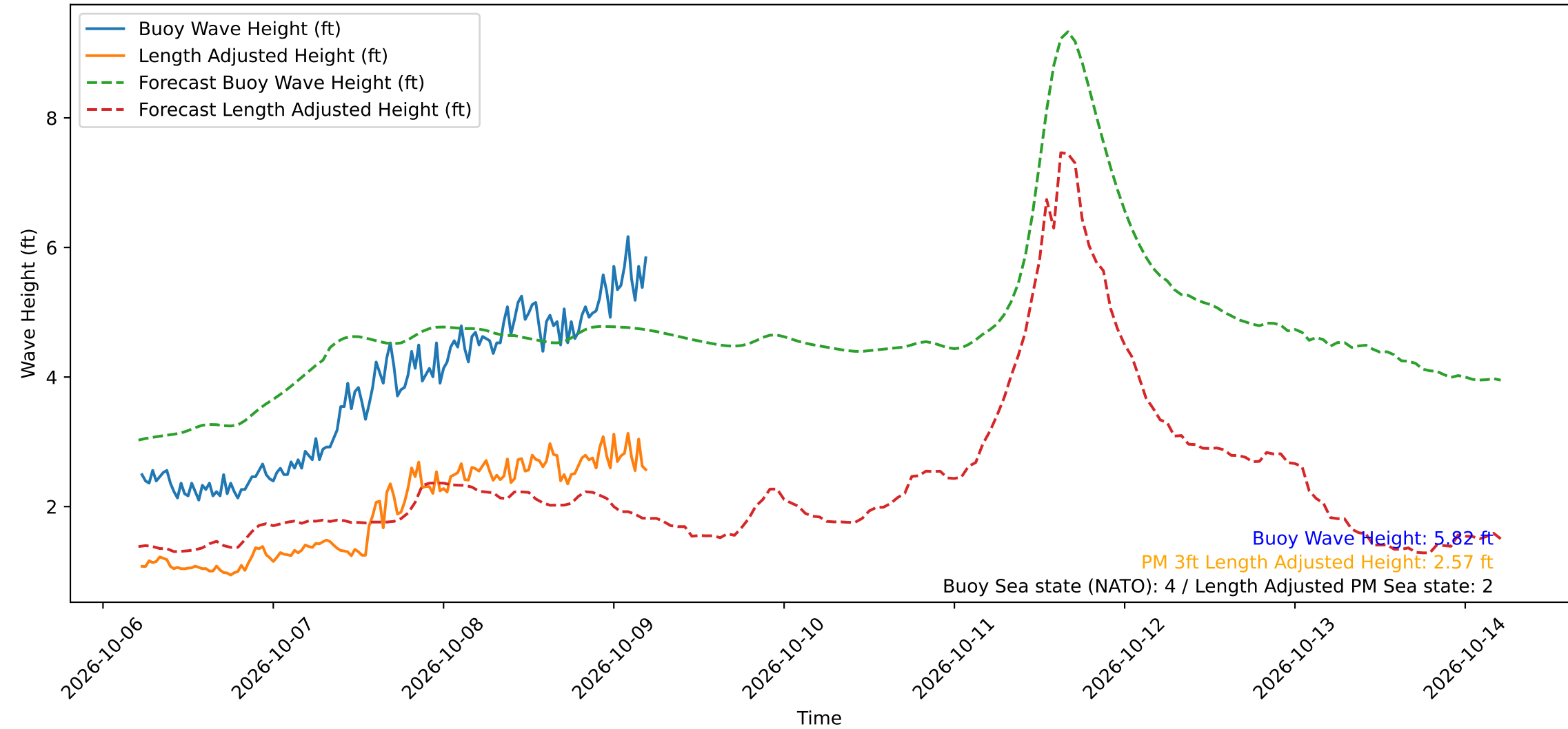
Wave Heights over Time for Green Beach at 2026-10-09 05:21:14
