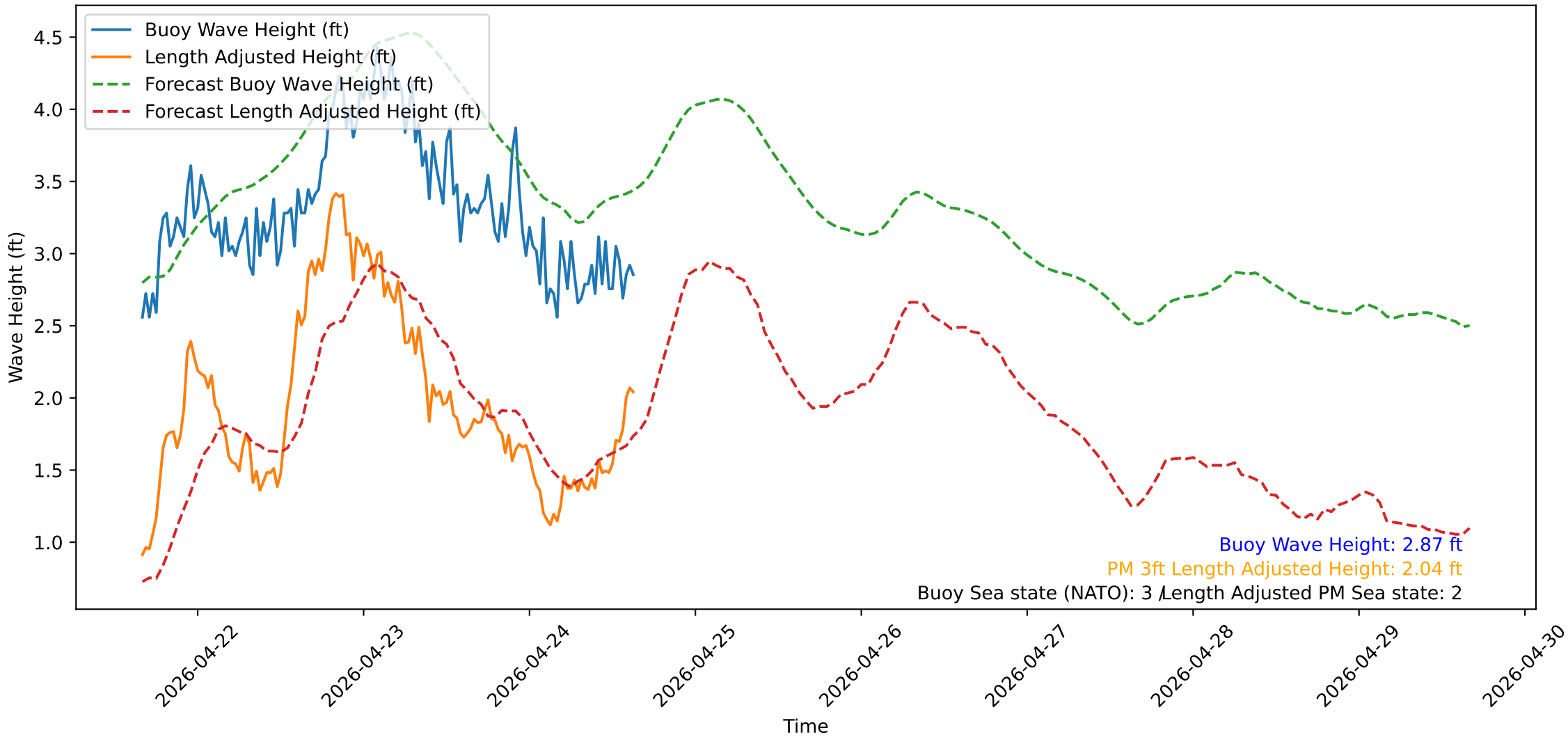
Wave Heights over Time for Oceanside Harbor at 2026-04-24 16:00:31
