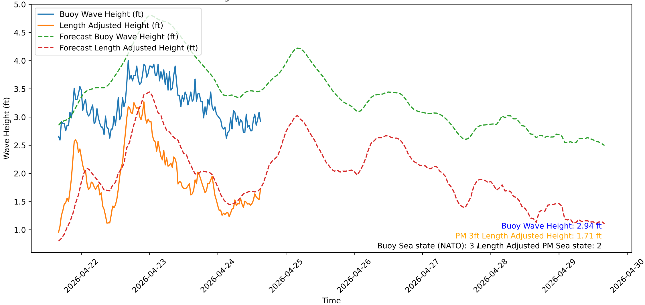
Wave Heights over Time for Green Beach at 2026-04-24 16:01:13
