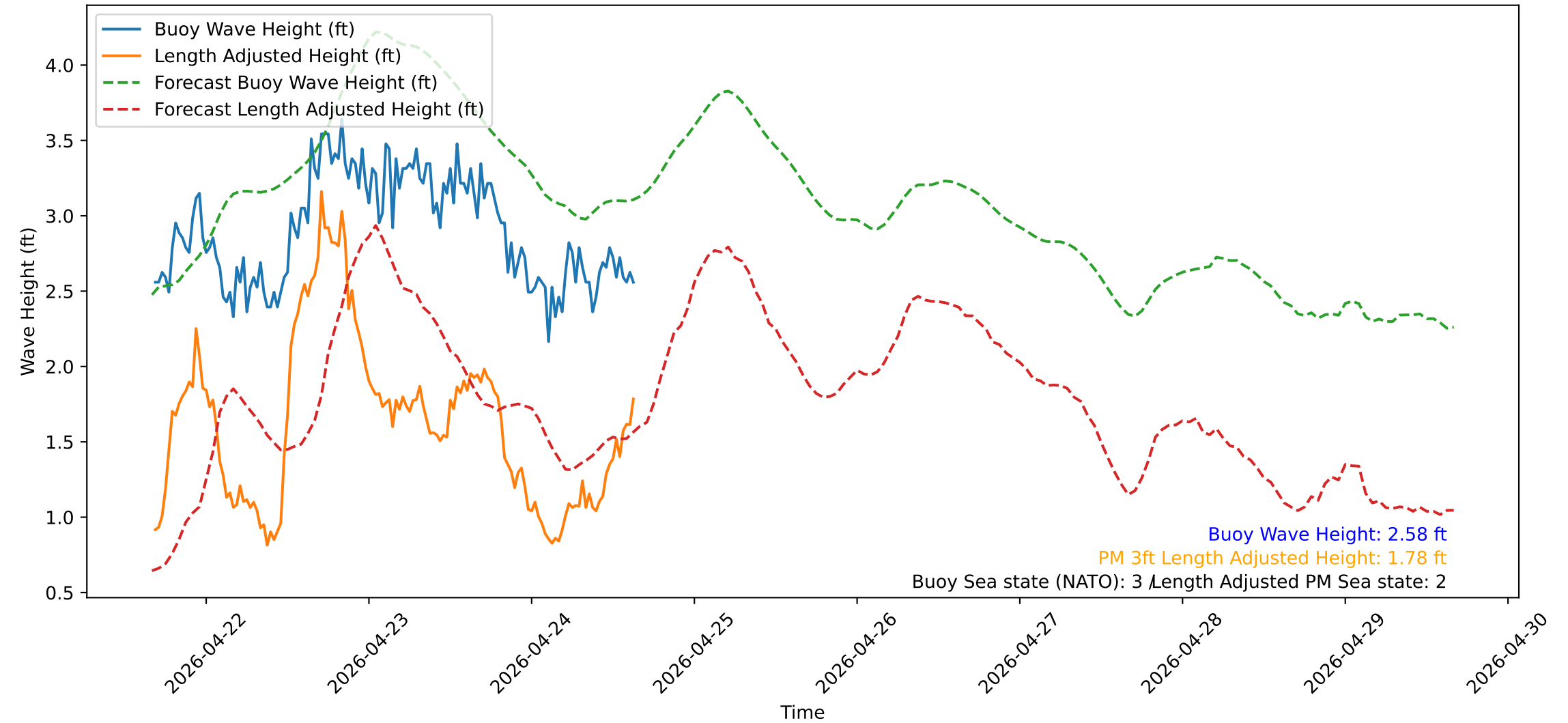
Wave Heights over Time for Red Beach at 2026-04-24 16:00:51
