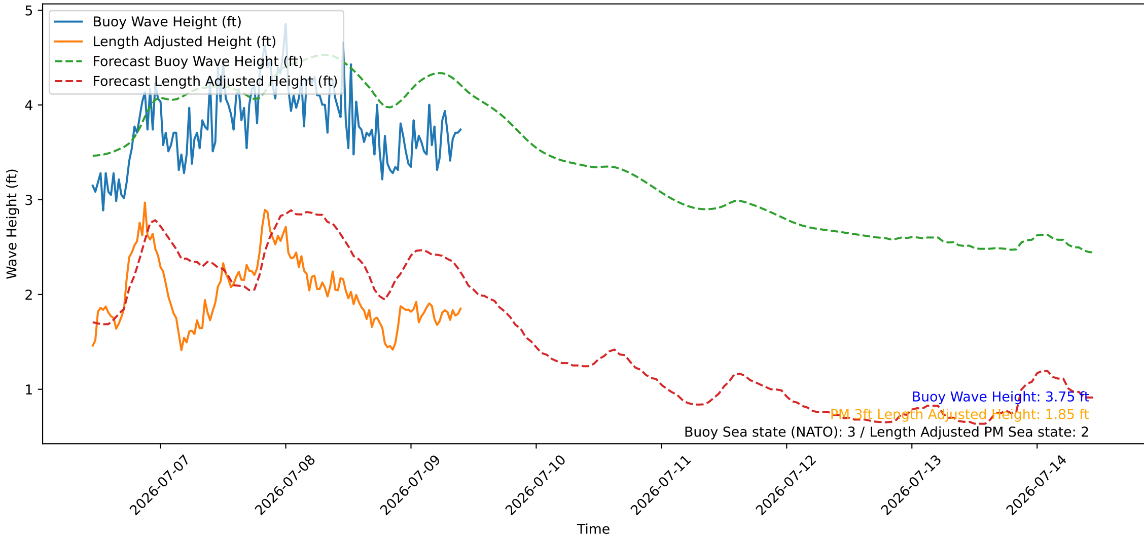
Wave Heights over Time for Red Beach at 2026-07-09 10:40:46
