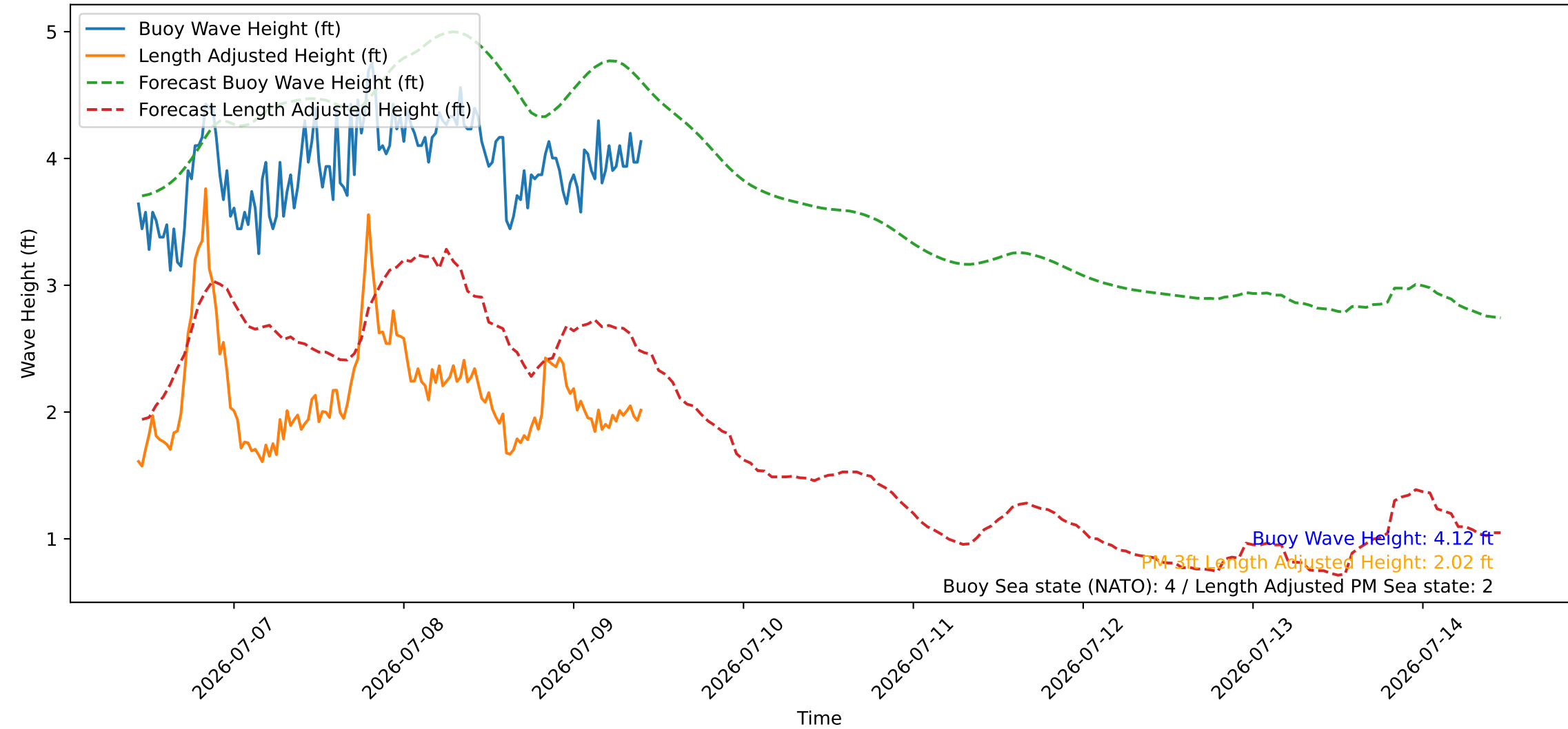
Wave Heights over Time for Green Beach at 2026-07-09 10:41:08
