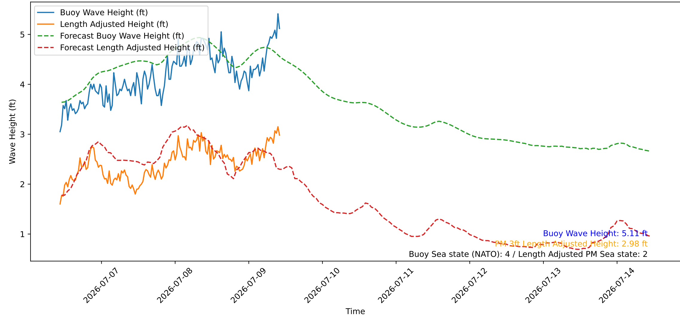
Wave Heights over Time for Oceanside Harbor at 2026-07-09 10:40:26
