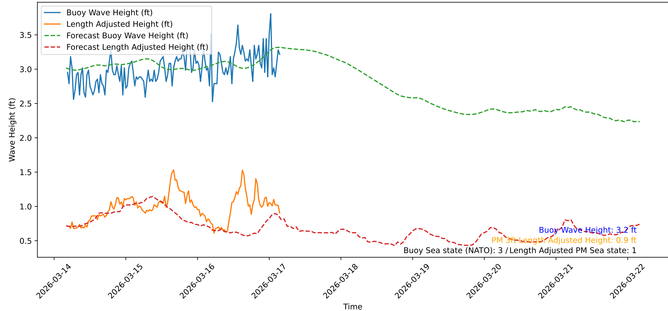
Wave Heights over Time for Red Beach at 2026-03-17 04:11:08
