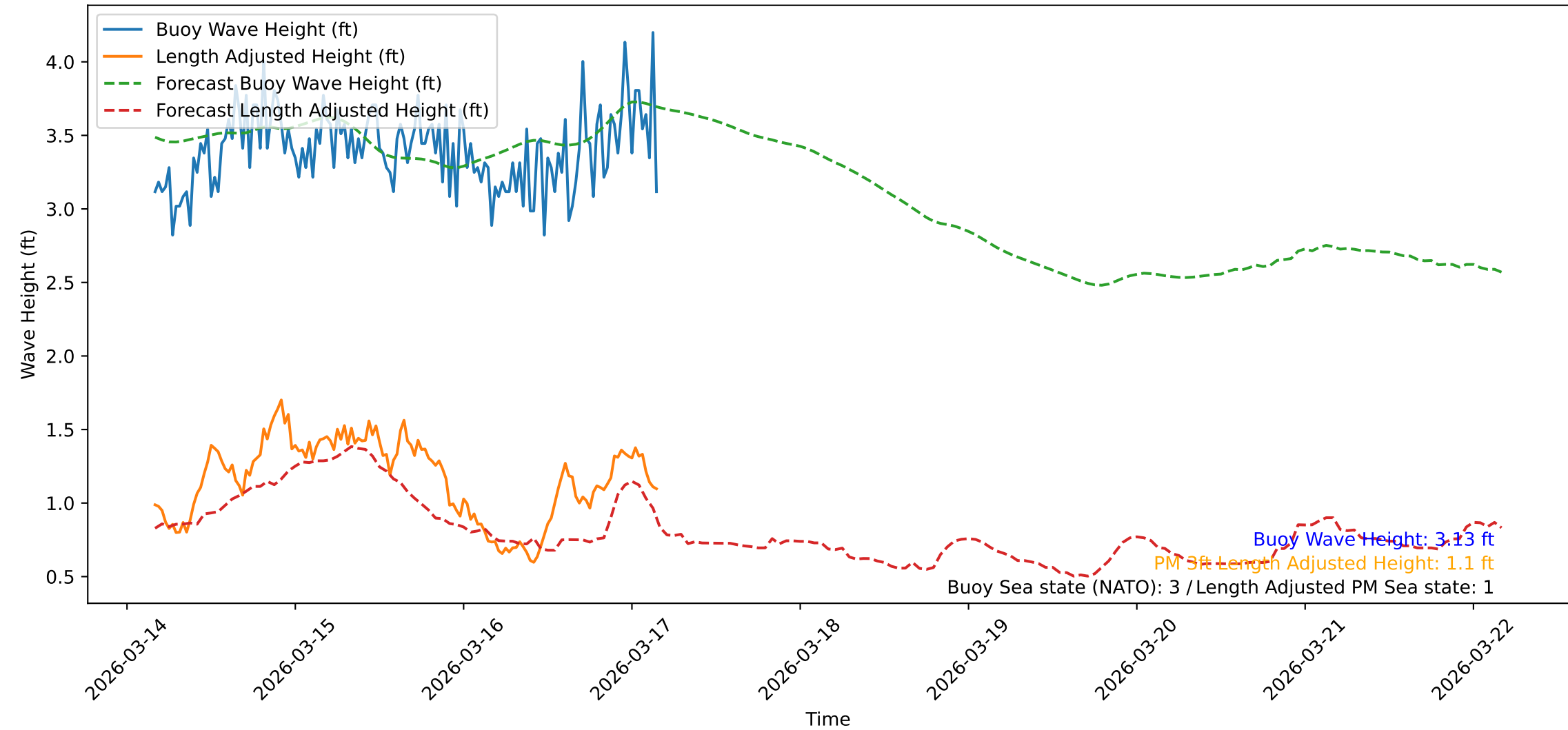
Wave Heights over Time for Green Beach at 2026-03-17 04:11:46
