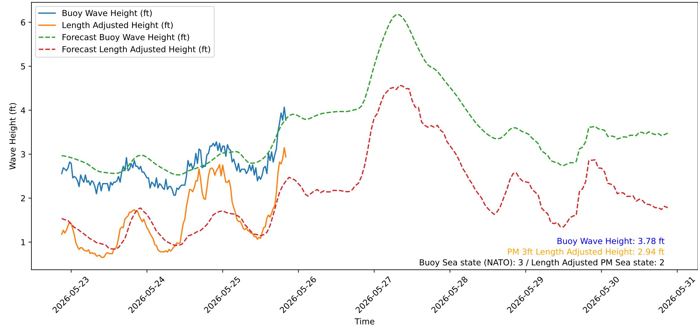
Wave Heights over Time for Green Beach at 2026-05-25 20:51:12
