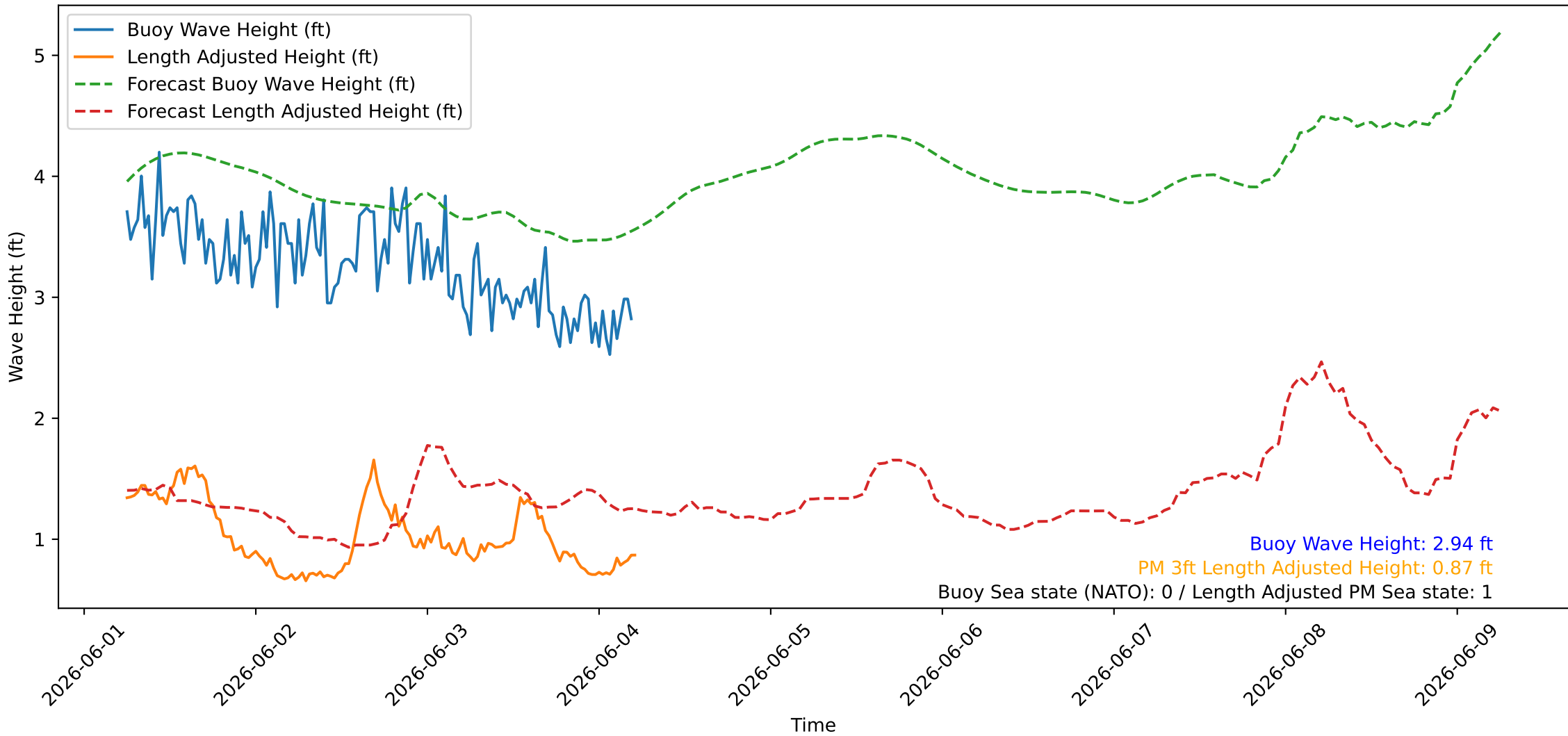
Wave Heights over Time for Red Beach at 2026-06-04 05:40:46
