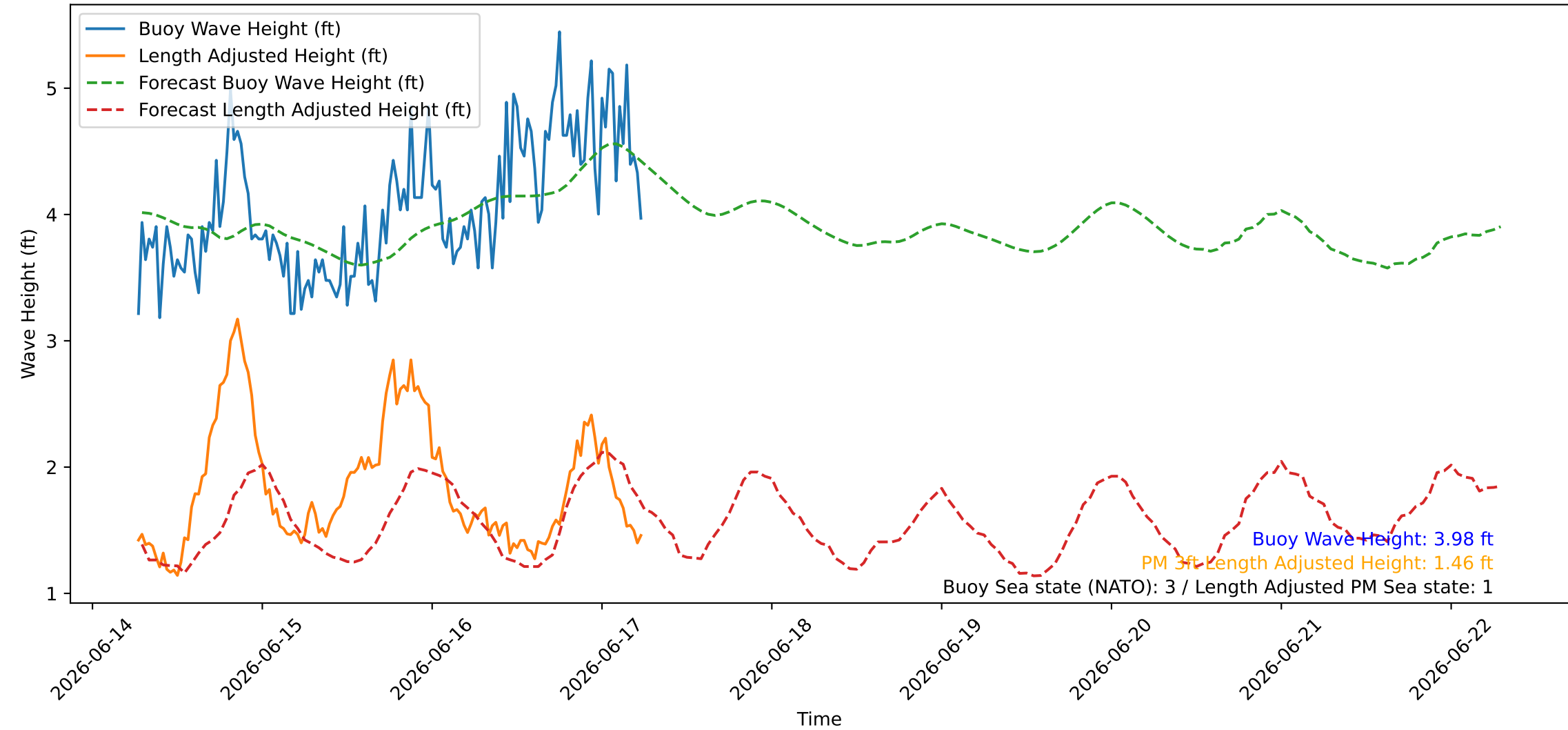
Wave Heights over Time for Oceanside Harbor at 2026-06-17 06:30:26
