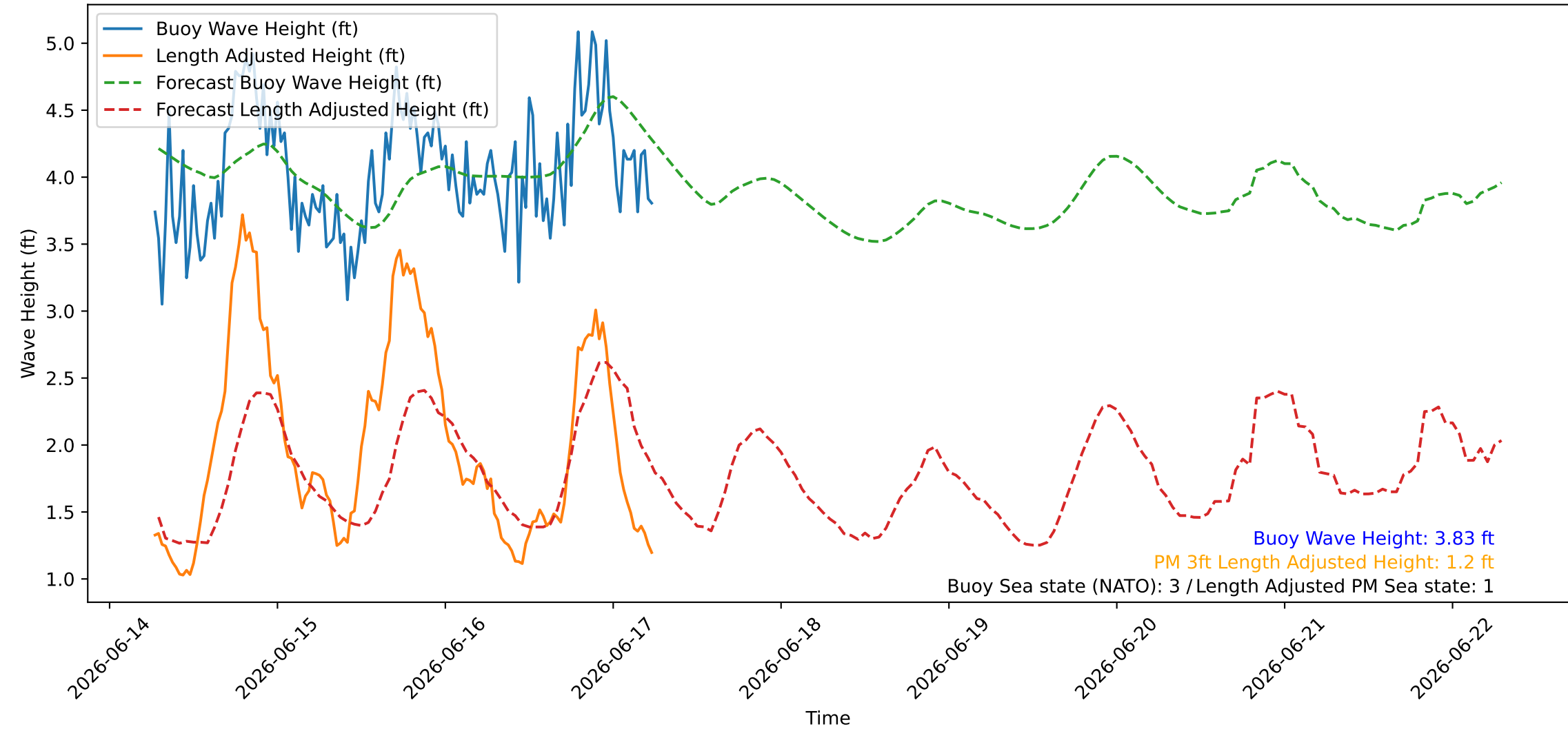
Wave Heights over Time for Green Beach at 2026-06-17 06:31:08
