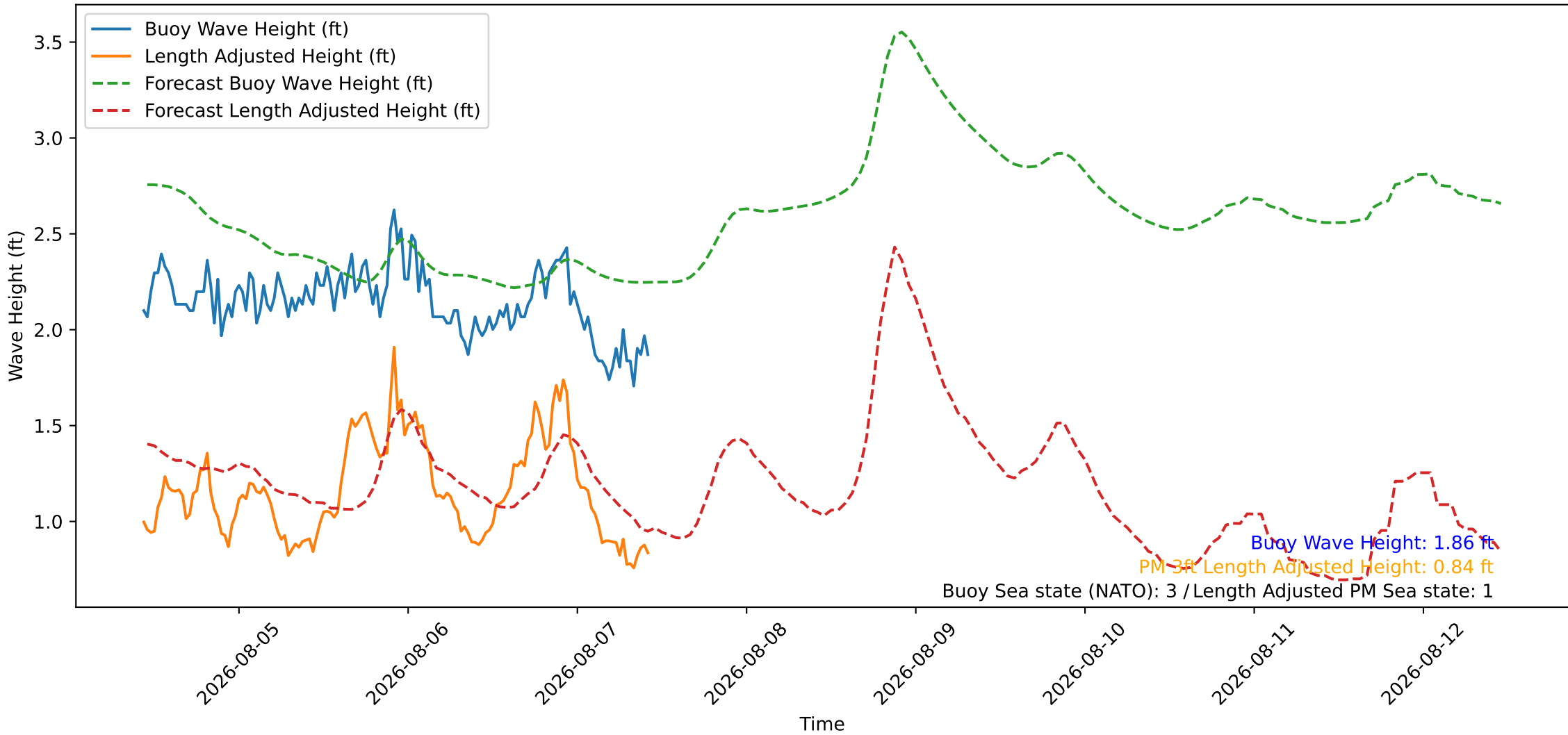
Wave Heights over Time for Green Beach at 2026-08-07 10:41:08
