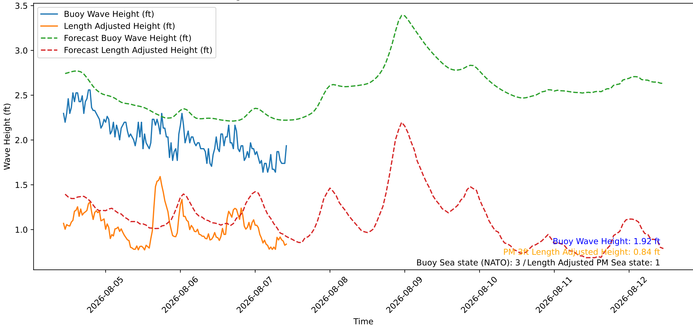
Wave Heights over Time for Oceanside Harbor at 2026-08-07 10:40:26
