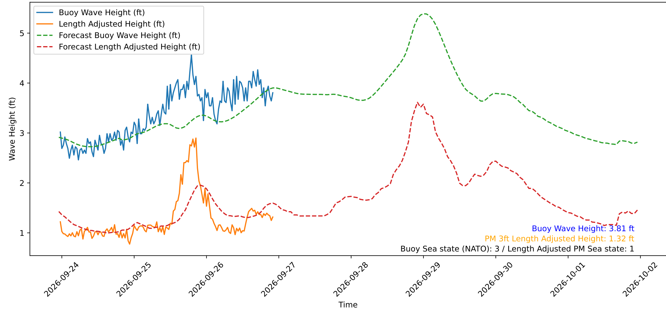
Wave Heights over Time for Green Beach at 2026-09-26 23:01:13
