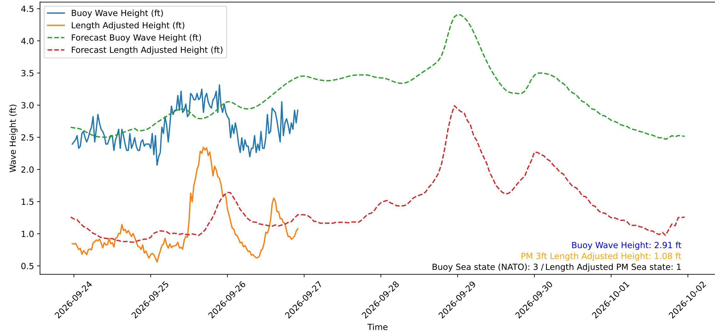
Wave Heights over Time for Red Beach at 2026-09-26 23:00:50
