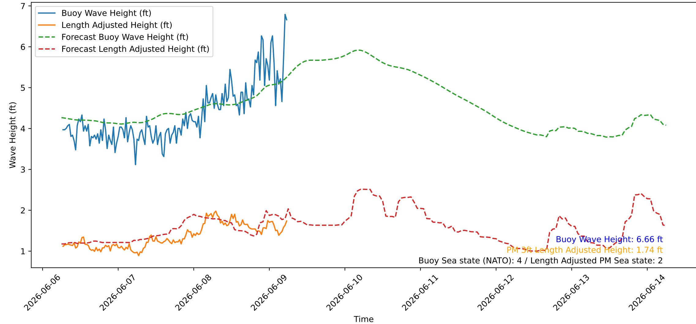
Wave Heights over Time for Green Beach at 2026-06-09 06:21:10
