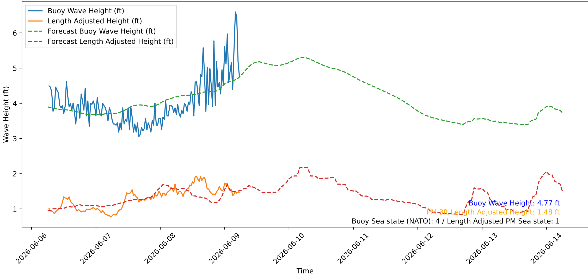
Wave Heights over Time for Red Beach at 2026-06-09 06:20:48
