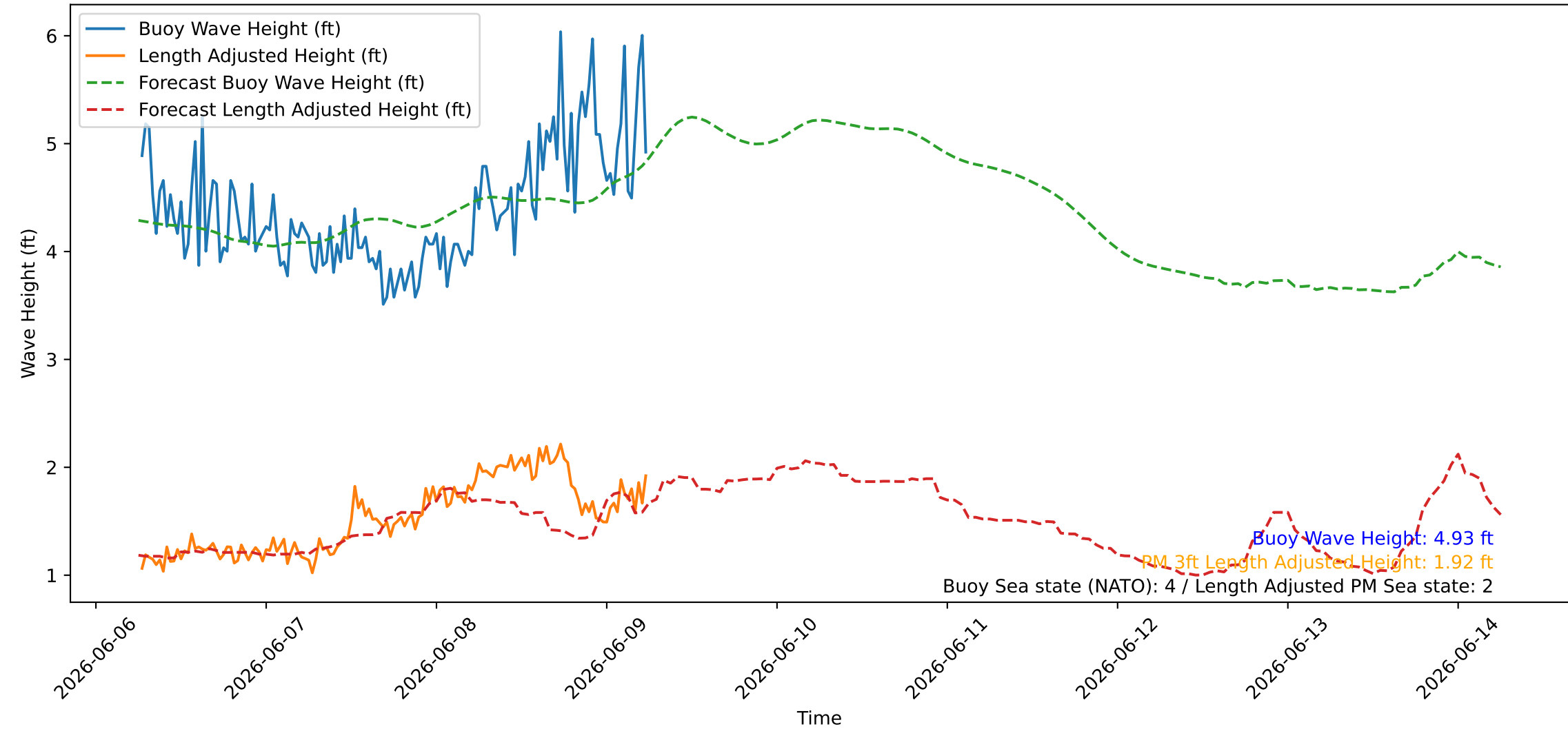
Wave Heights over Time for Oceanside Harbor at 2026-06-09 06:20:27
