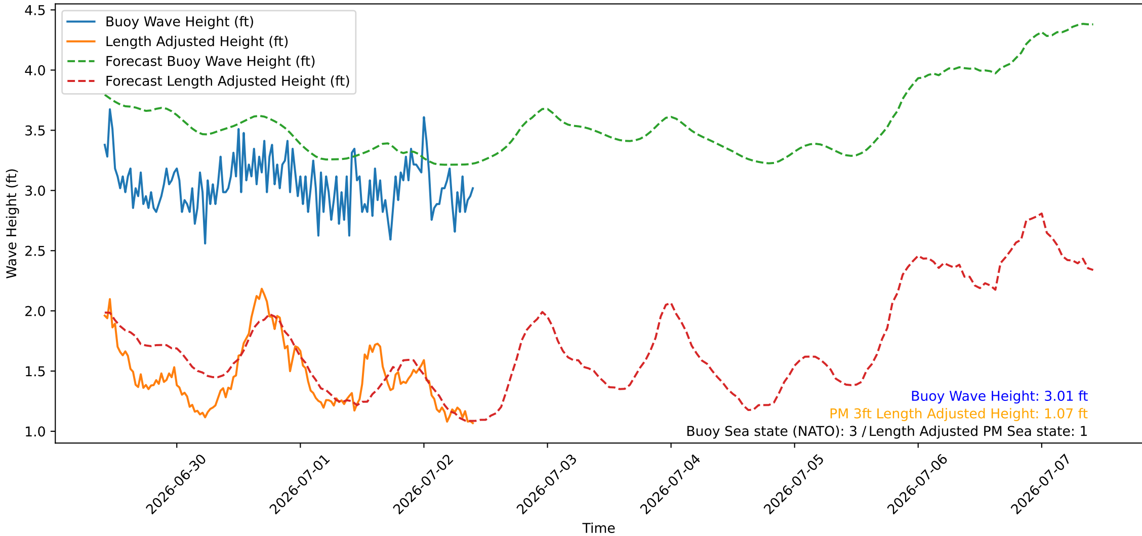
Wave Heights over Time for Oceanside Harbor at 2026-07-02 10:10:26
