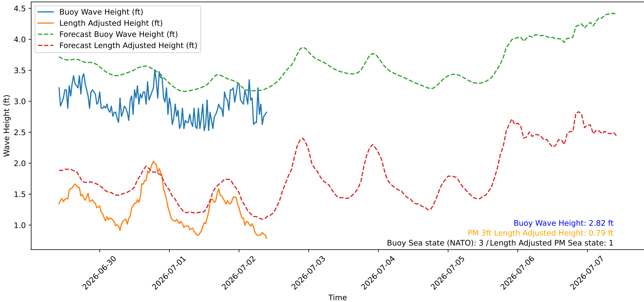
Wave Heights over Time for Green Beach at 2026-07-02 10:11:07
