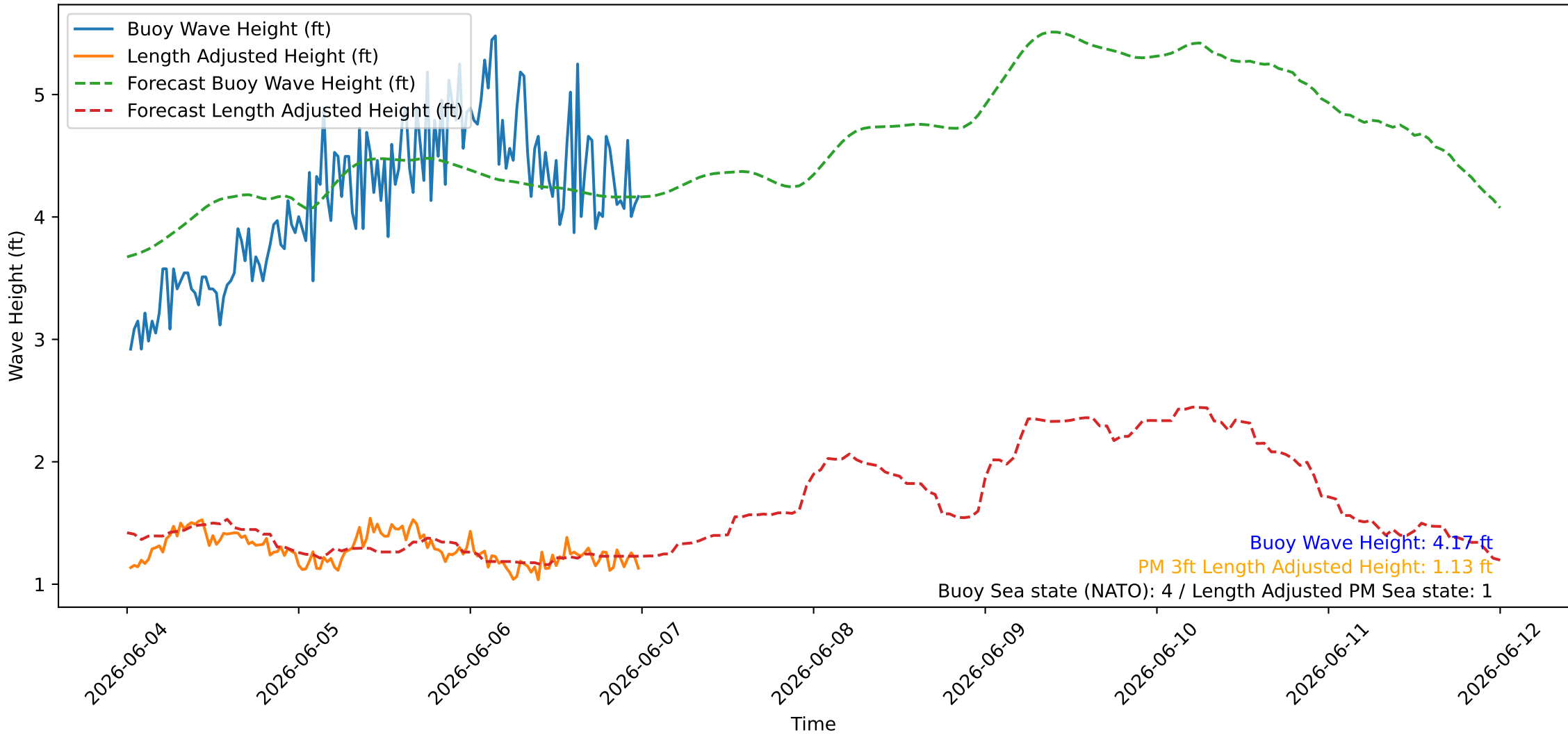
Wave Heights over Time for Oceanside Harbor at 2026-06-07 00:20:26
