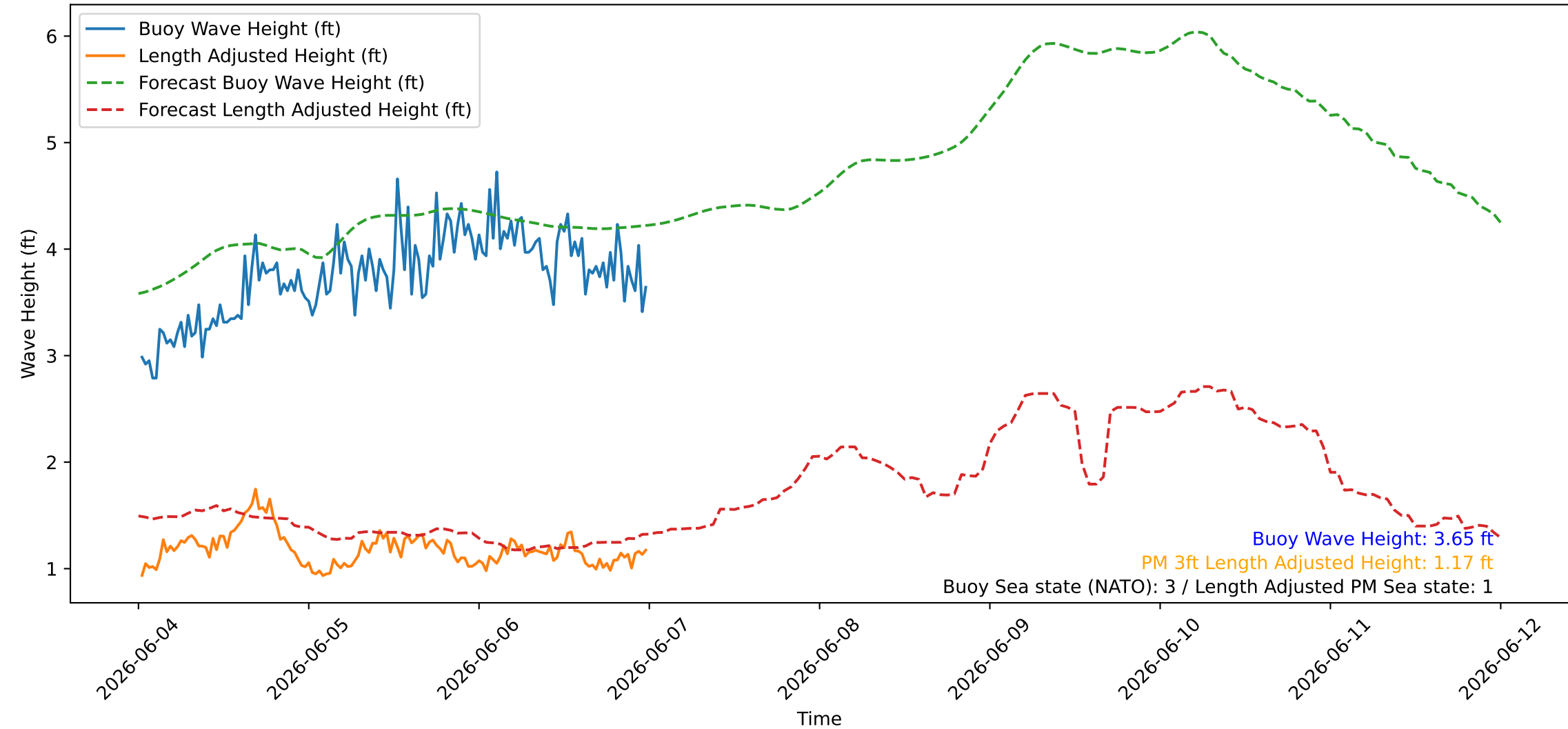
Wave Heights over Time for Green Beach at 2026-06-07 00:21:09
