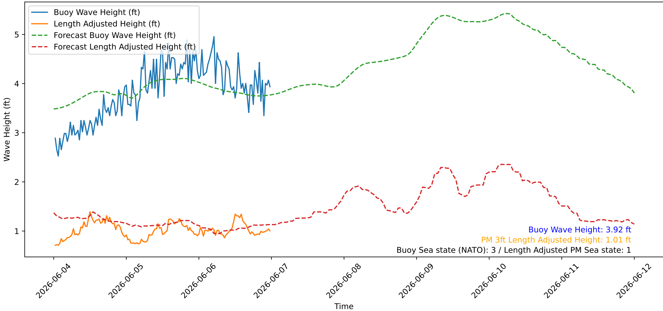
Wave Heights over Time for Red Beach at 2026-06-07 00:20:46
