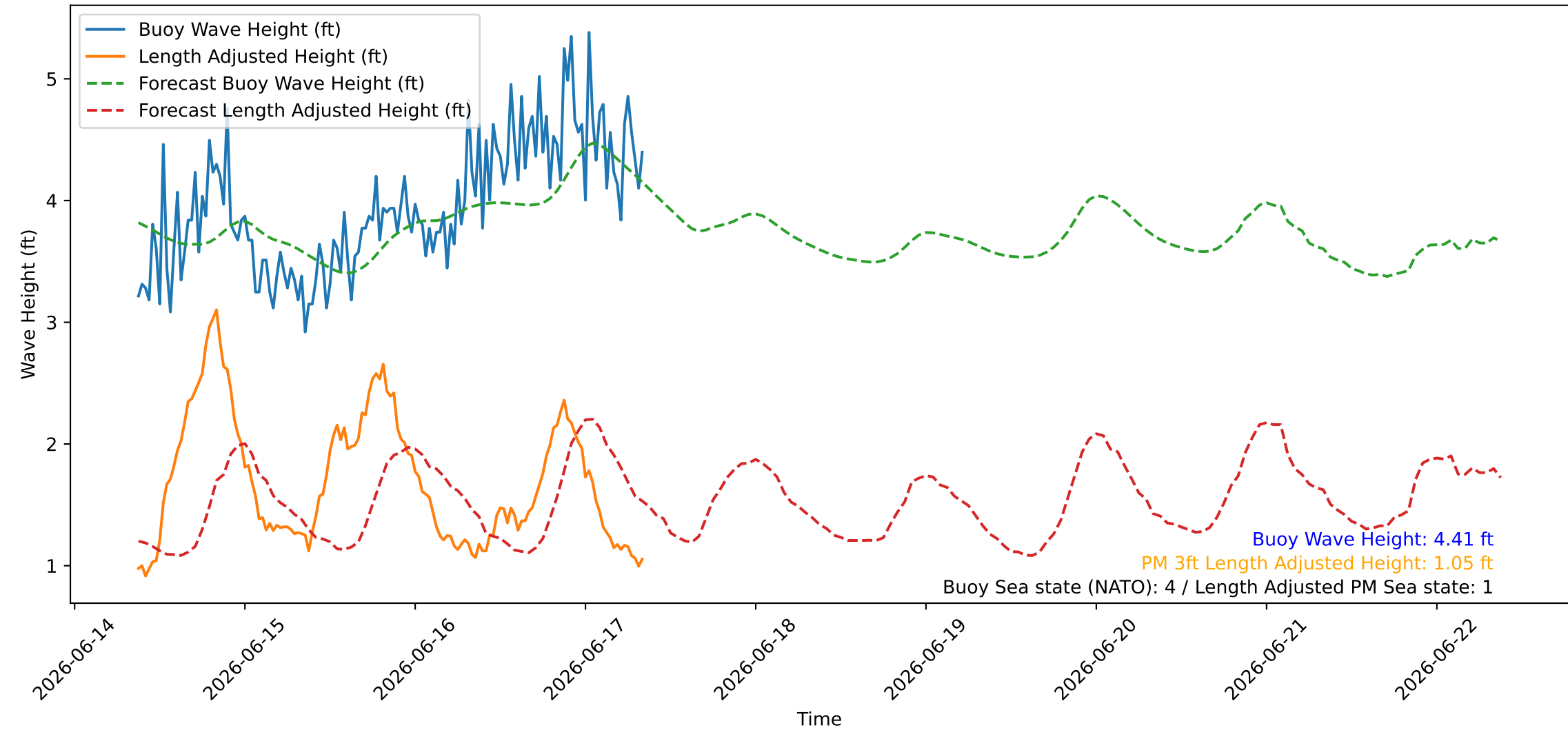
Wave Heights over Time for Red Beach at 2026-06-17 08:50:48
