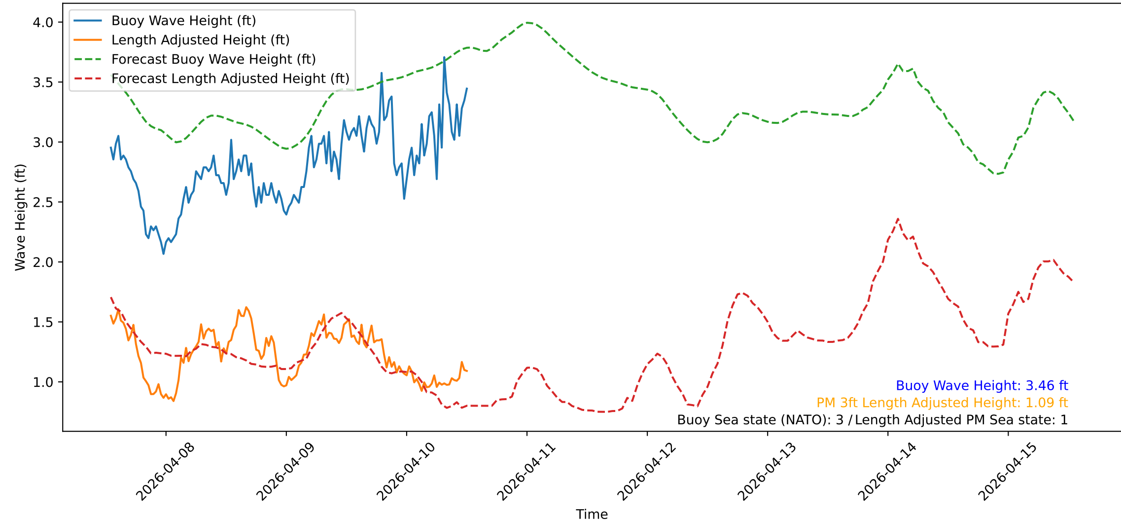
Wave Heights over Time for Red Beach at 2026-04-10 12:50:51
