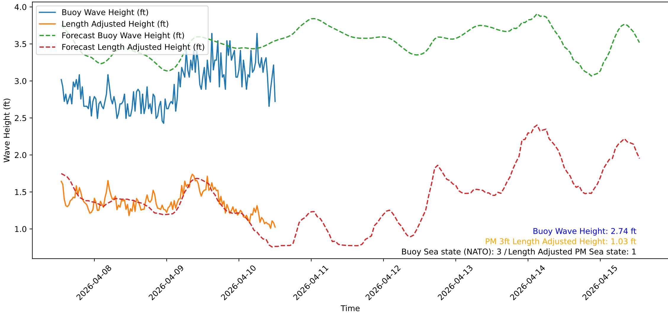
Wave Heights over Time for Oceanside Harbor at 2026-04-10 12:50:31
