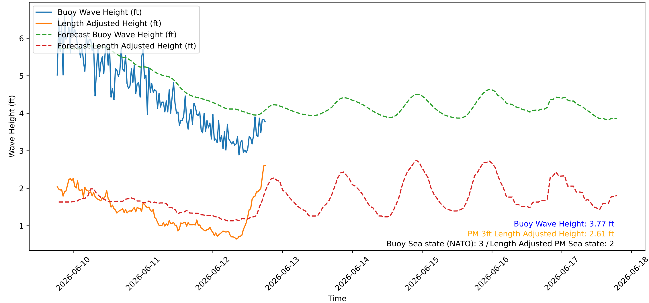
Wave Heights over Time for Green Beach at 2026-06-12 18:41:08
