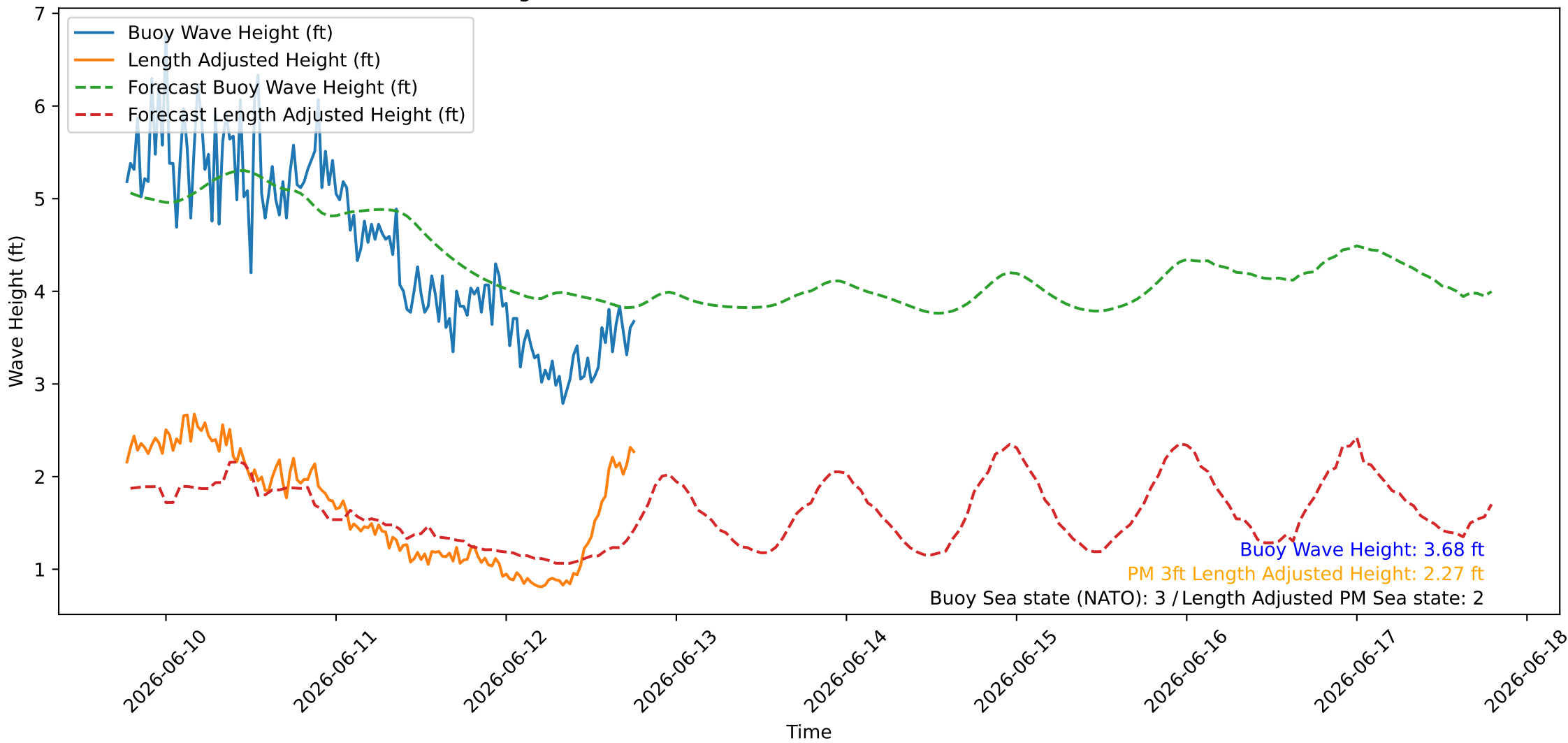
Wave Heights over Time for Oceanside Harbor at 2026-06-12 18:40:26
