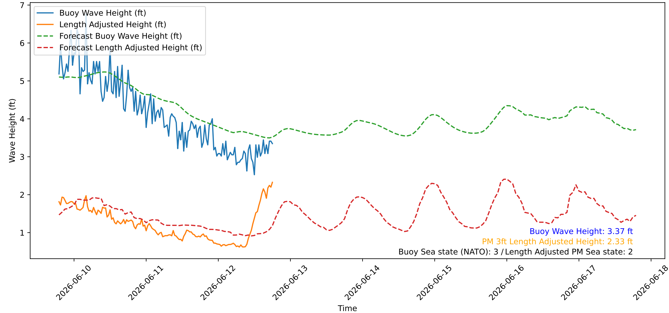
Wave Heights over Time for Red Beach at 2026-06-12 18:40:45
