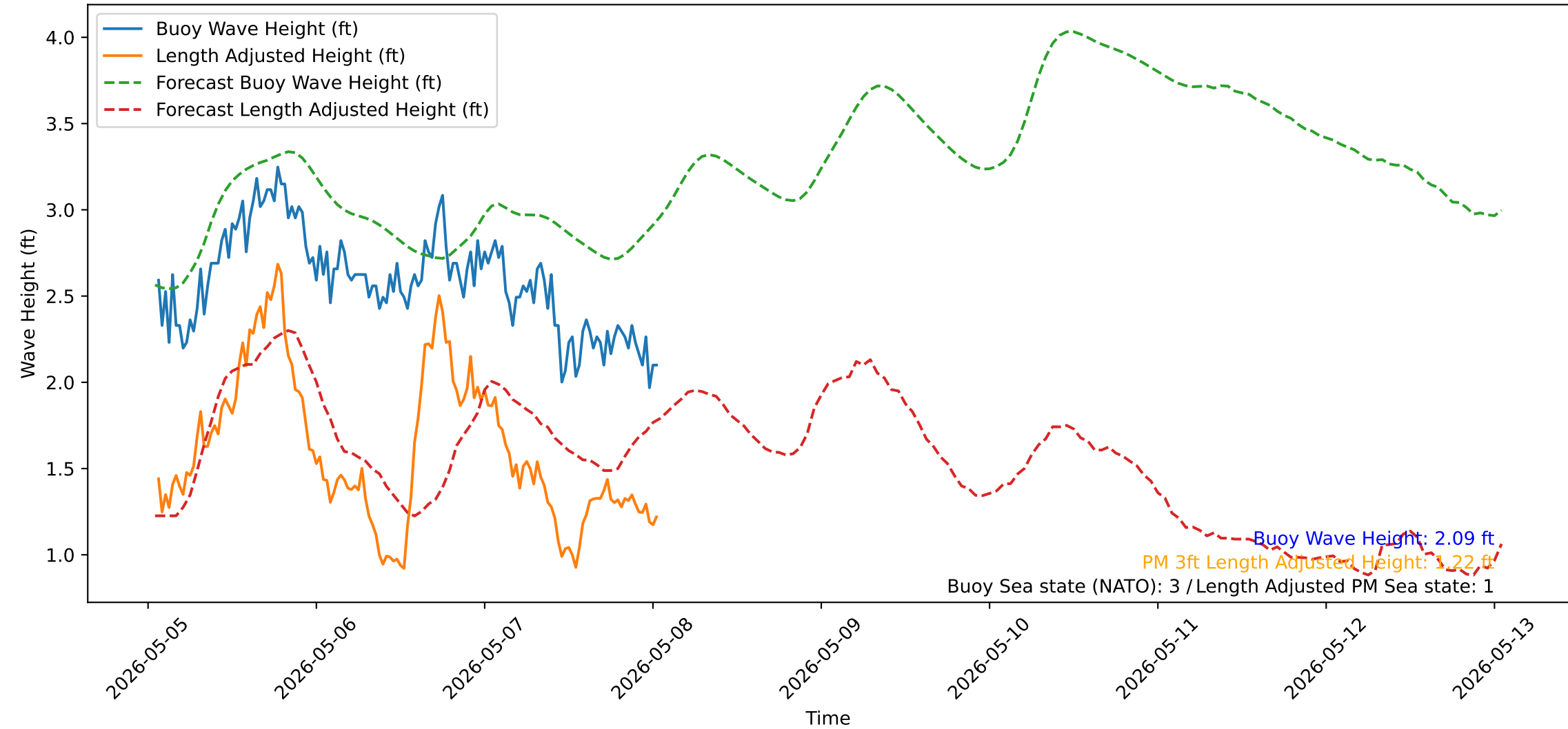
Wave Heights over Time for Oceanside Harbor at 2026-05-08 01:20:31
