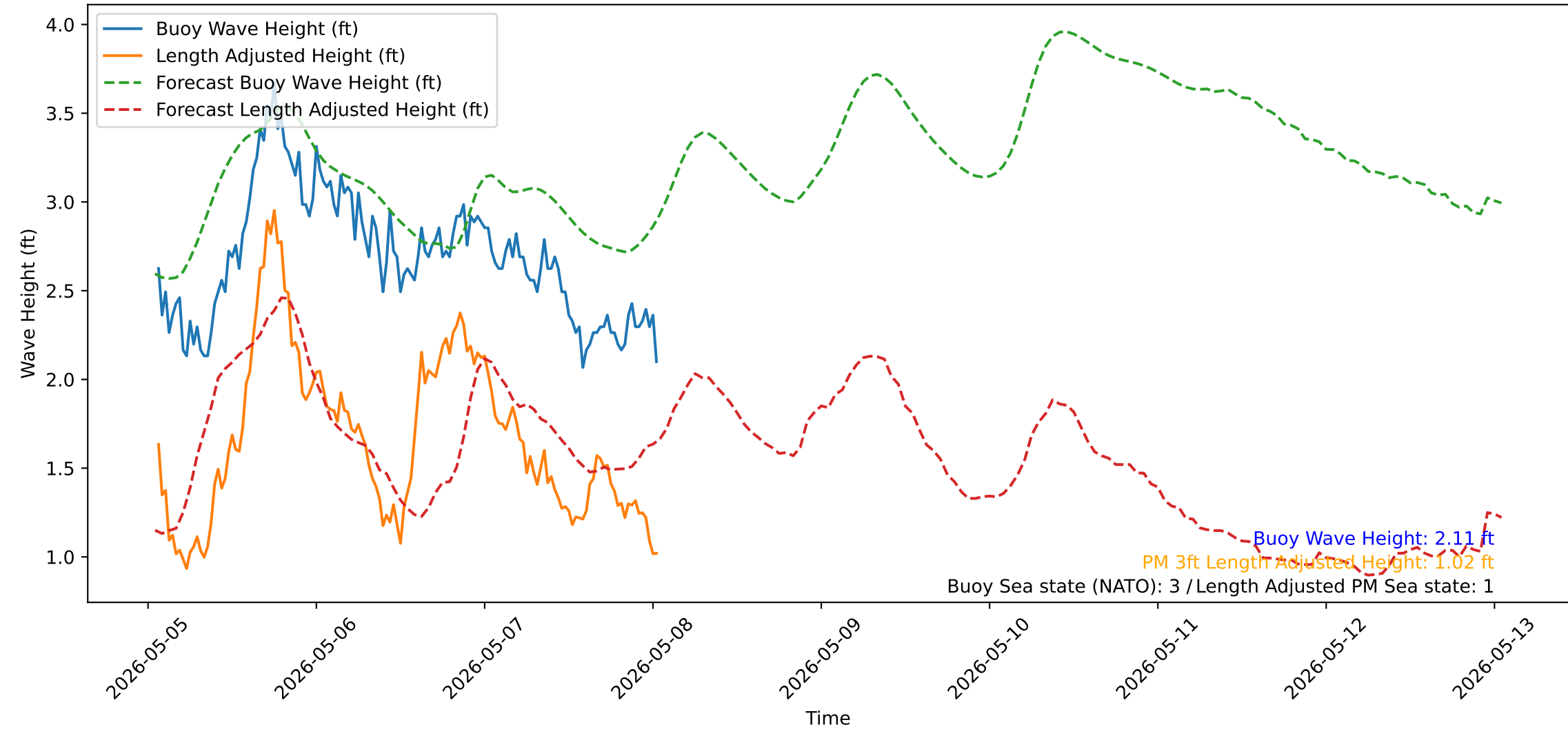
Wave Heights over Time for Green Beach at 2026-05-08 01:21:14
