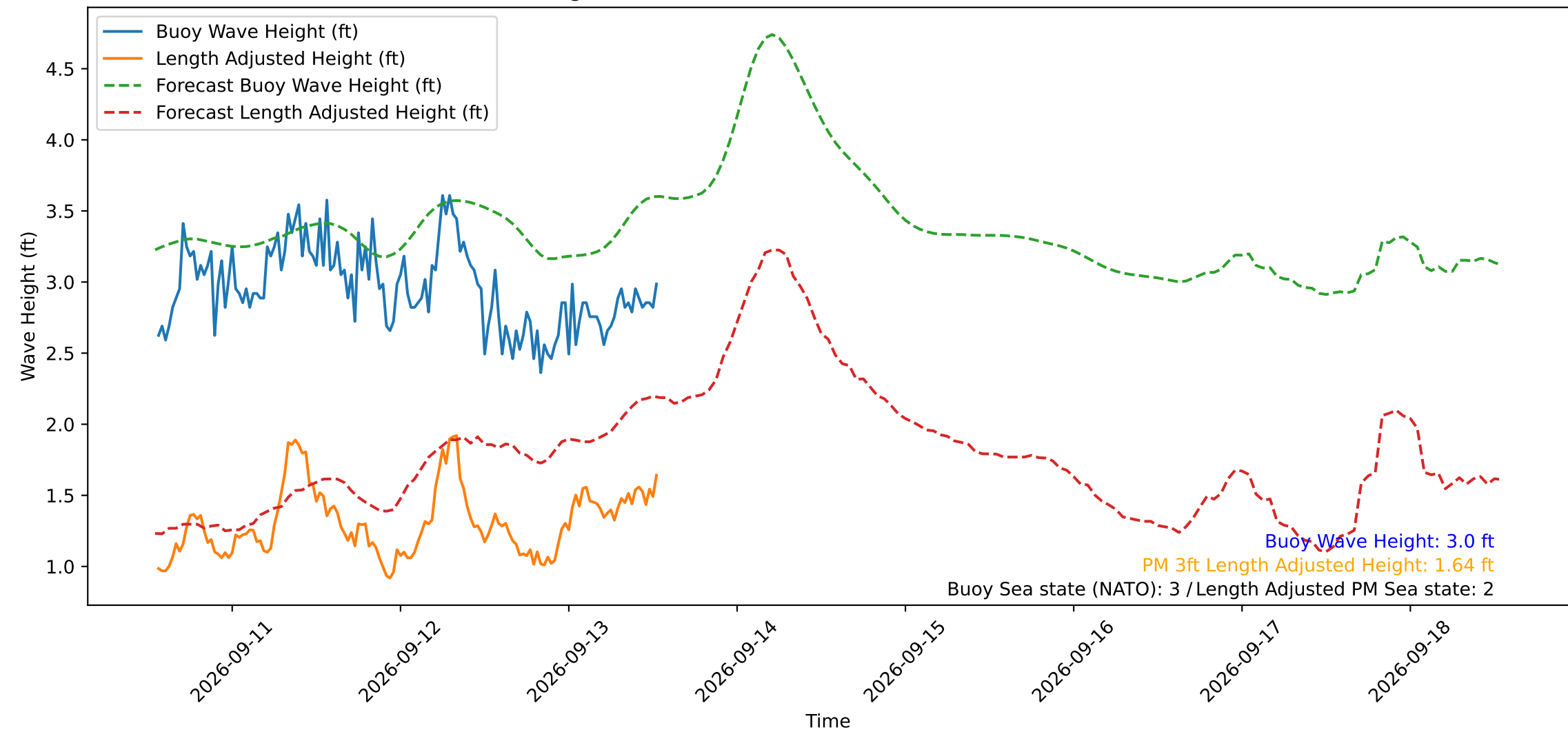
Wave Heights over Time for Green Beach at 2026-09-13 13:21:14
