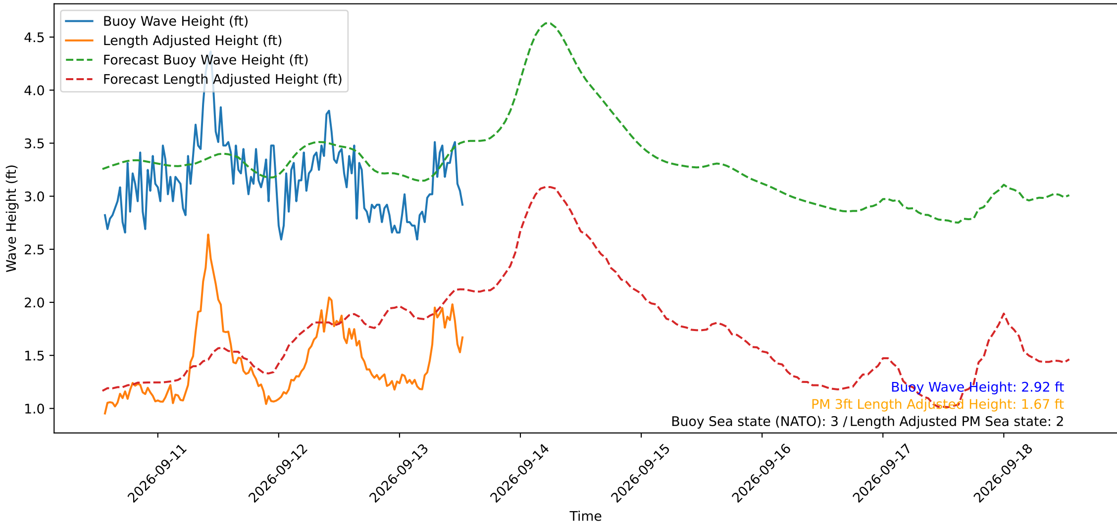
Wave Heights over Time for Oceanside Harbor at 2026-09-13 13:20:29
