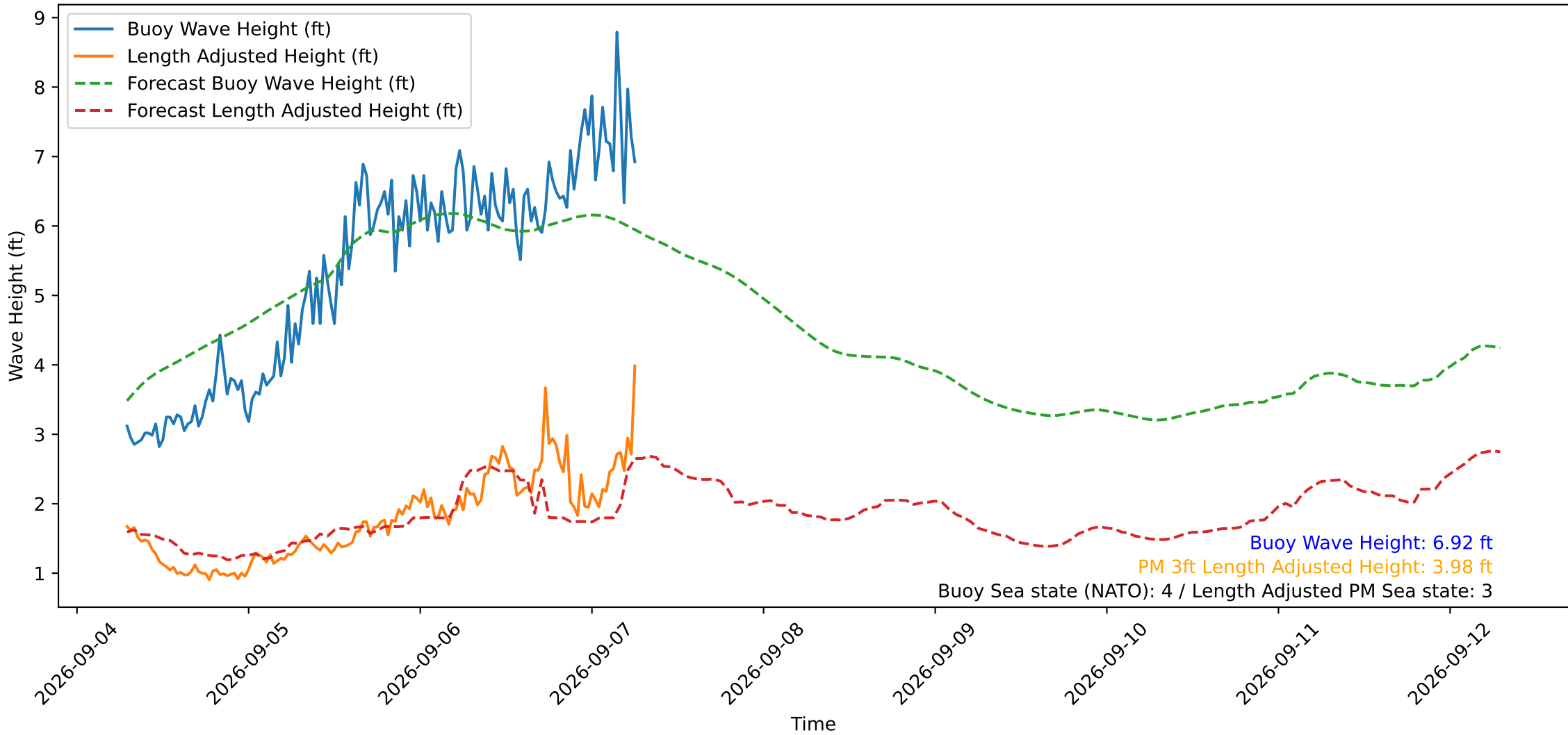
Wave Heights over Time for Green Beach at 2026-09-07 06:41:11
