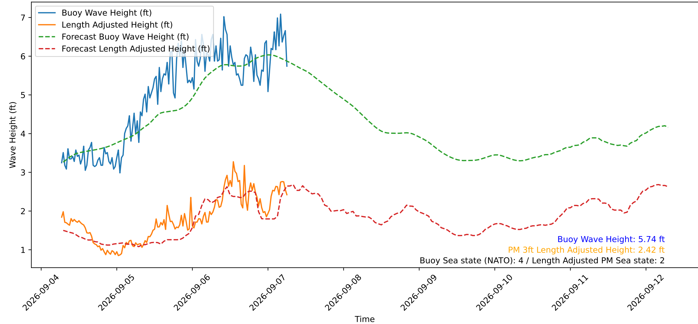
Wave Heights over Time for Oceanside Harbor at 2026-09-07 06:40:29
