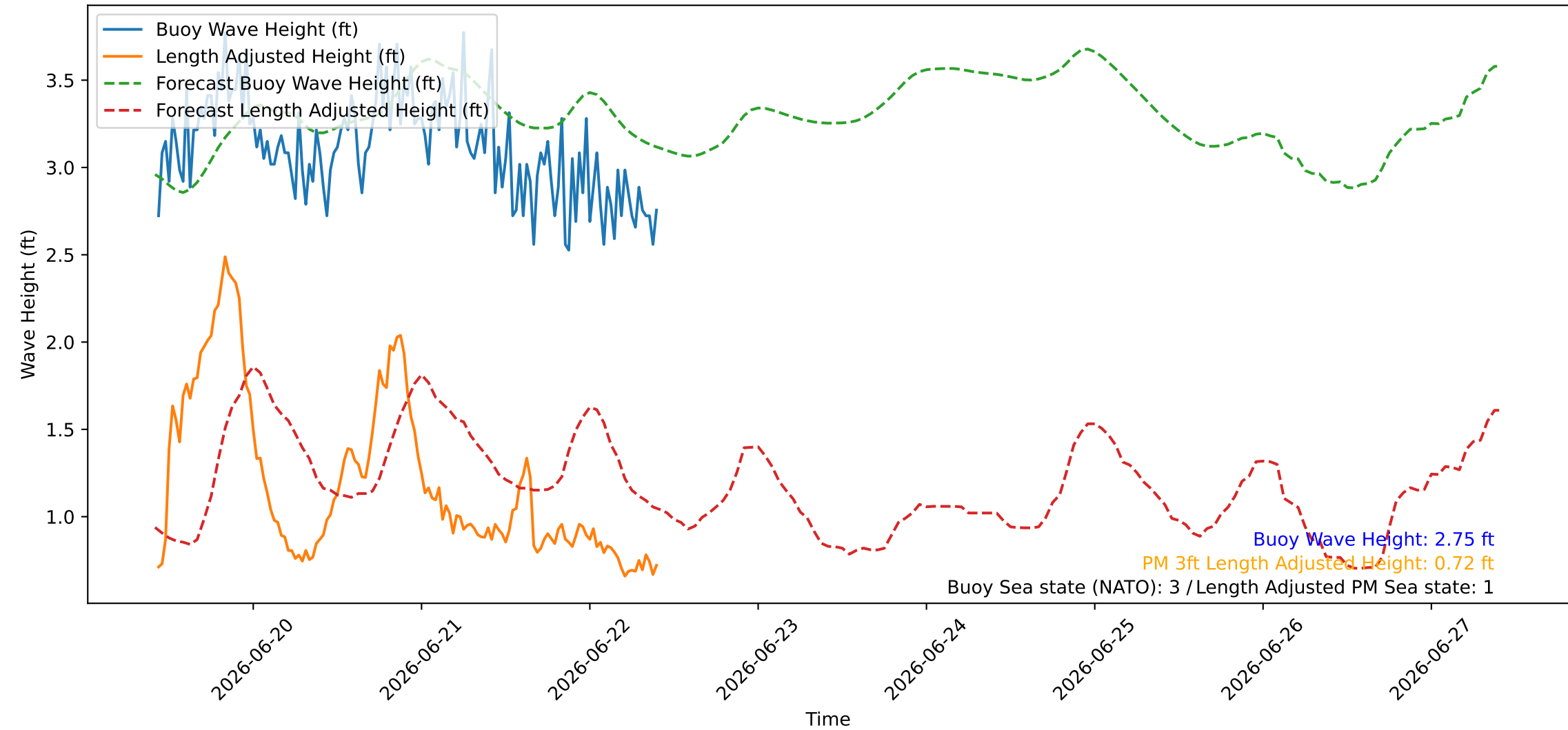
Wave Heights over Time for Red Beach at 2026-06-22 10:10:45
