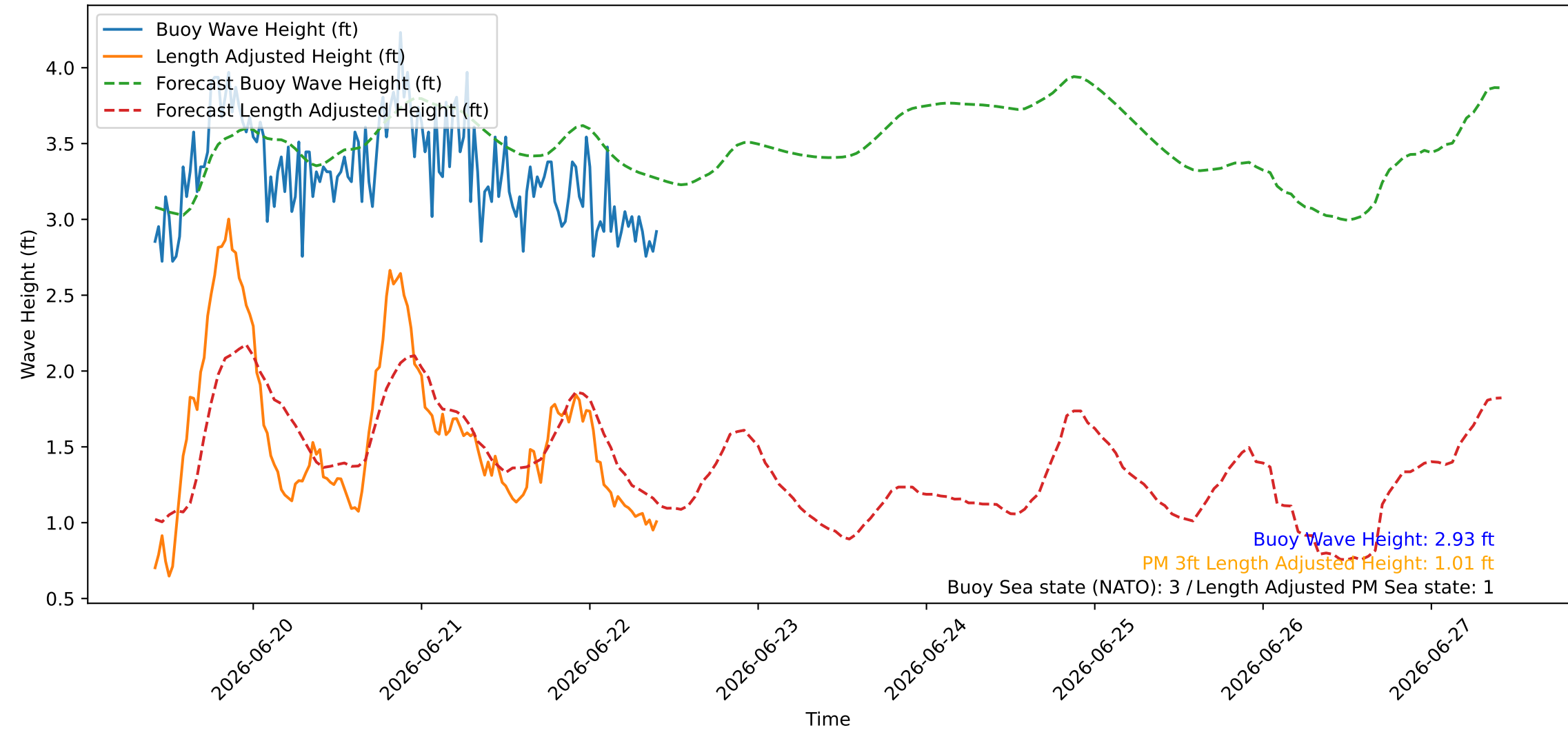
Wave Heights over Time for Green Beach at 2026-06-22 10:11:08
