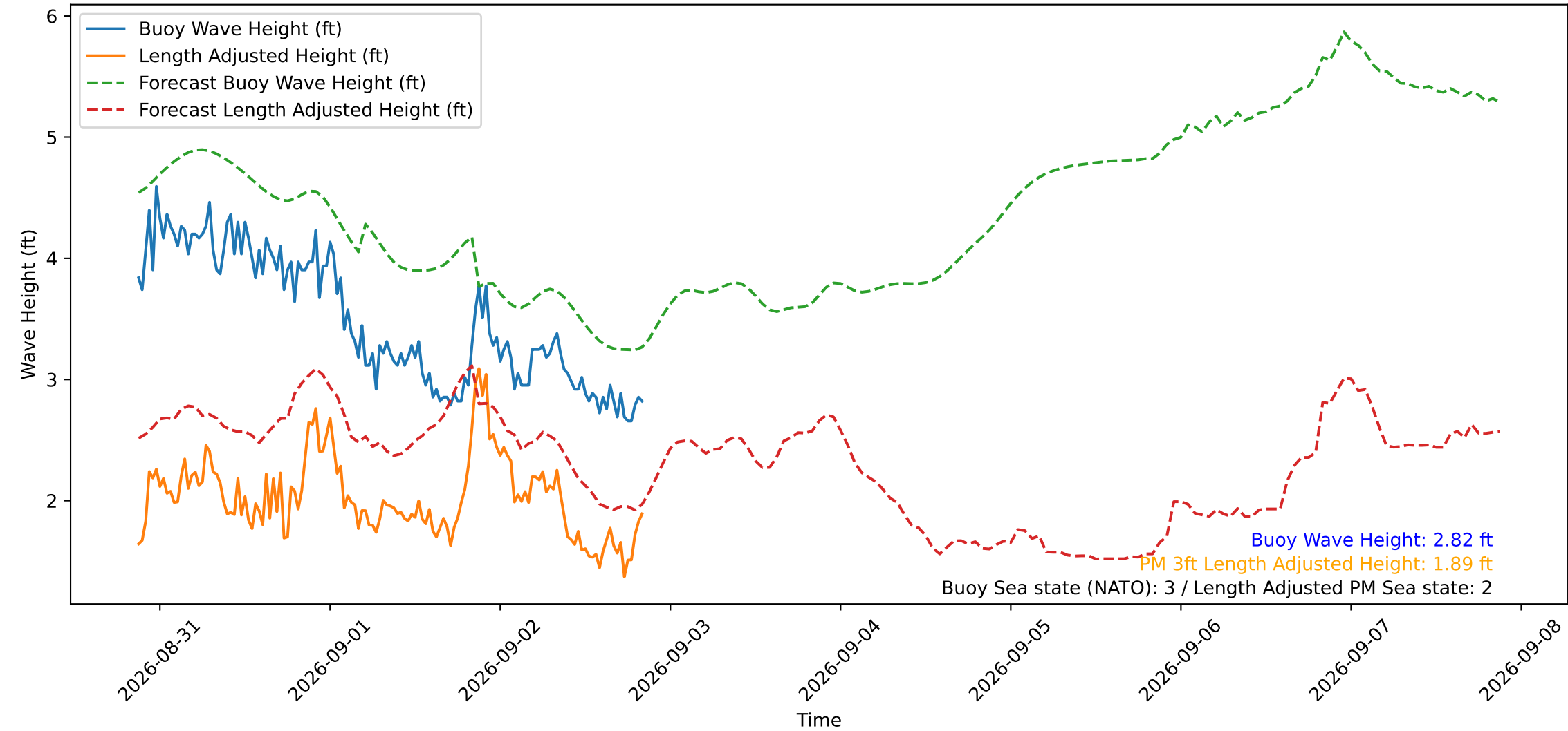
Wave Heights over Time for Green Beach at 2026-09-02 20:41:13
