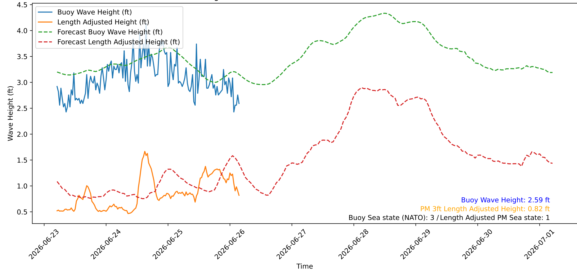
Wave Heights over Time for Red Beach at 2026-06-26 04:30:45
