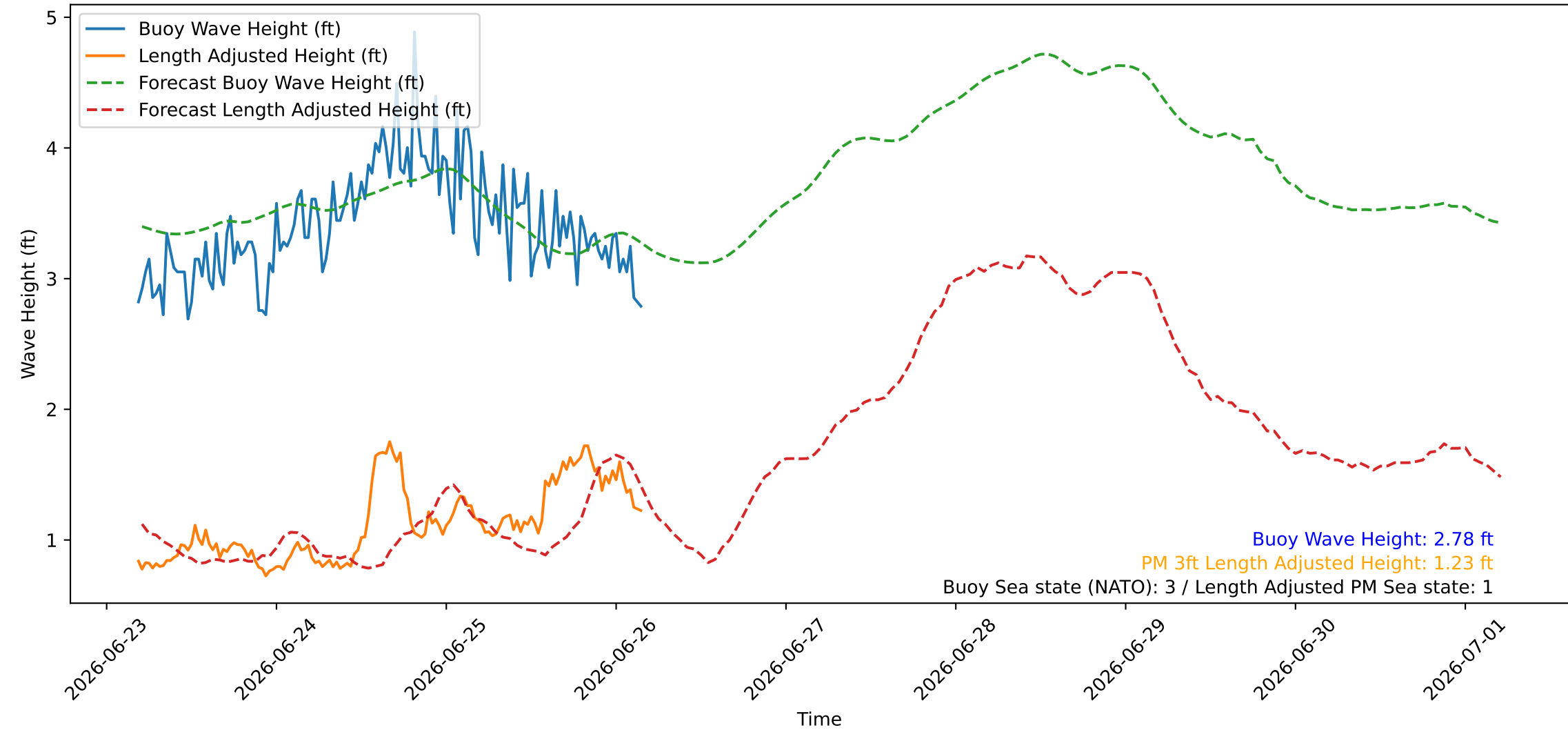
Wave Heights over Time for Oceanside Harbor at 2026-06-26 04:30:26
