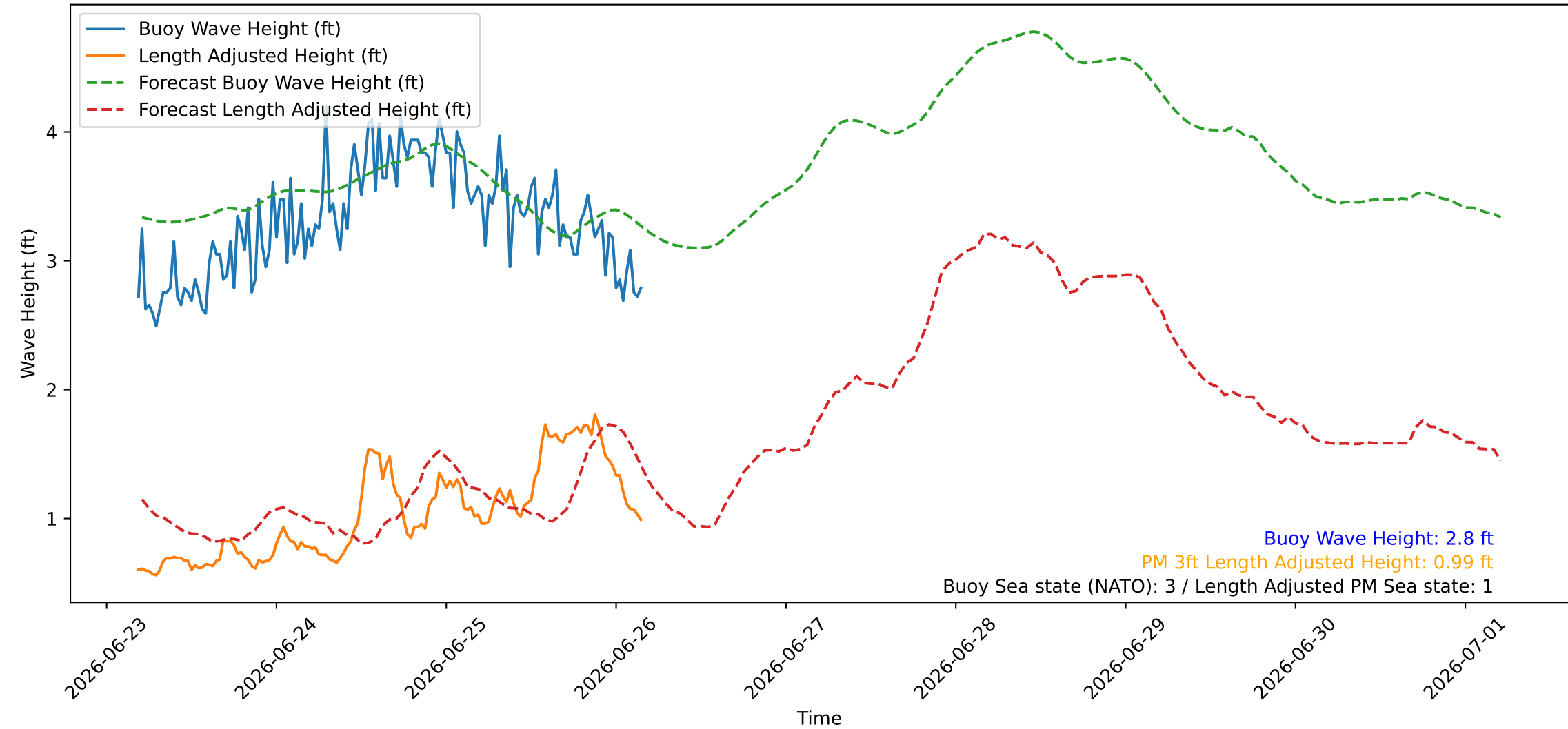
Wave Heights over Time for Green Beach at 2026-06-26 04:31:08
