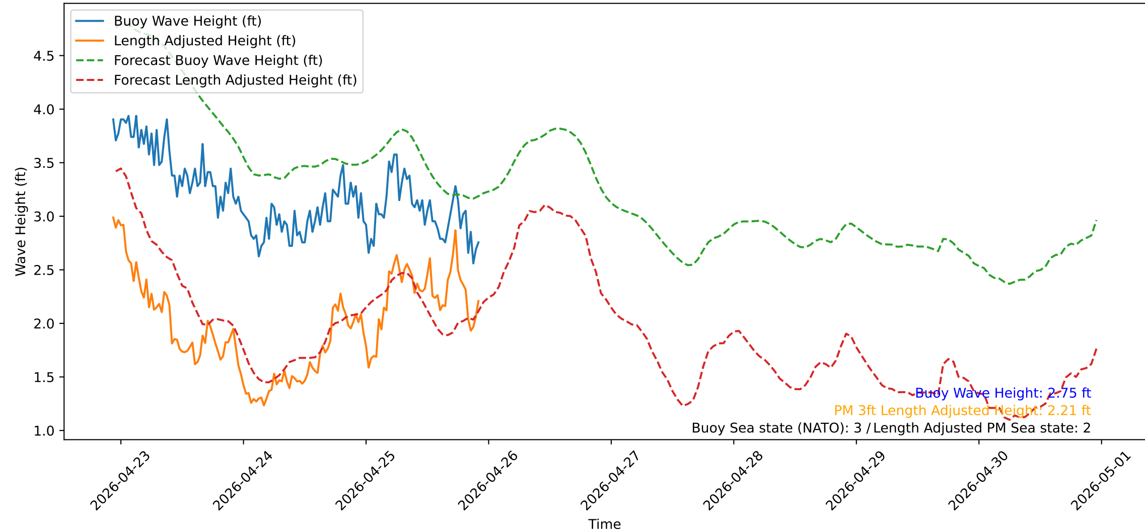
Wave Heights over Time for Green Beach at 2026-04-25 22:41:13
