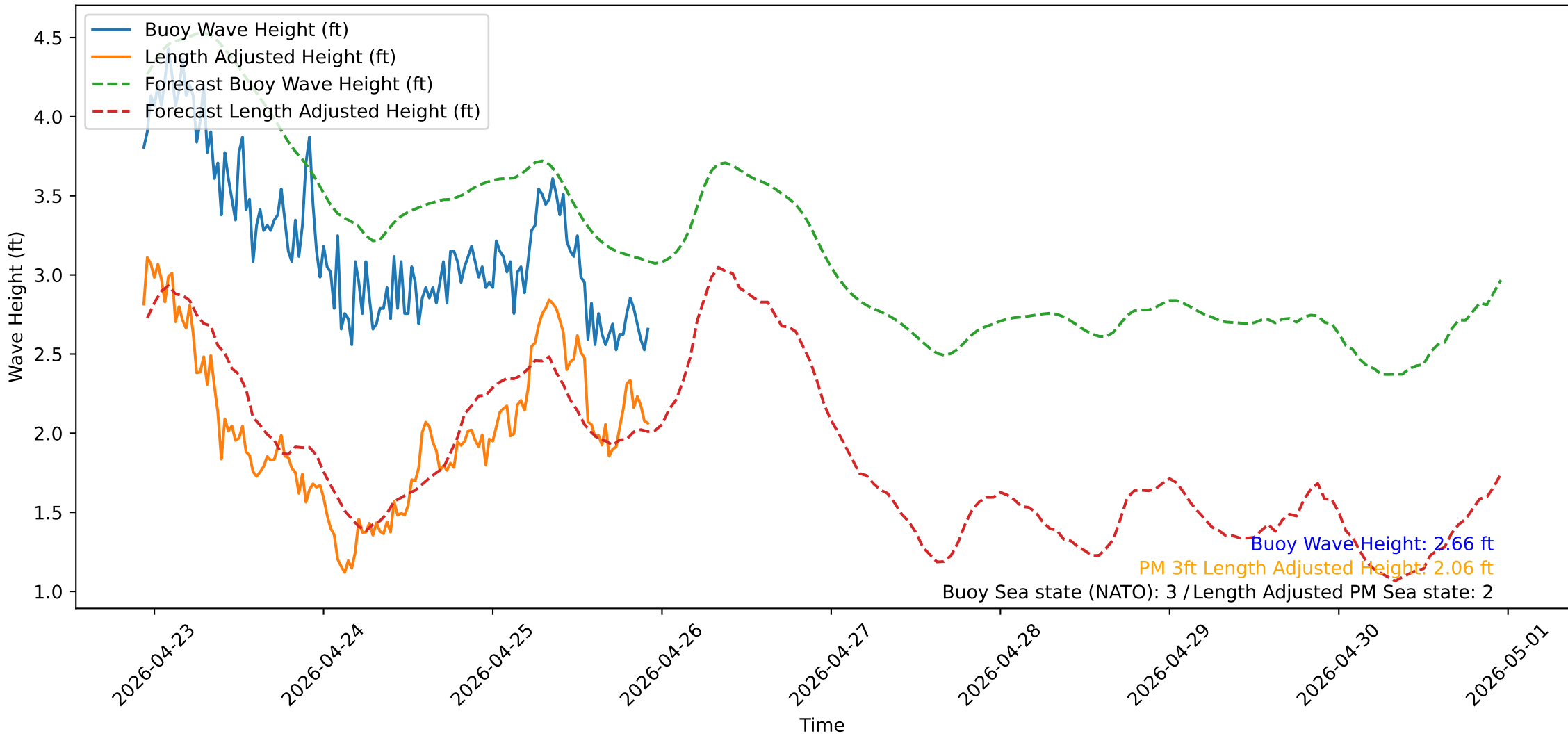
Wave Heights over Time for Oceanside Harbor at 2026-04-25 22:40:31
