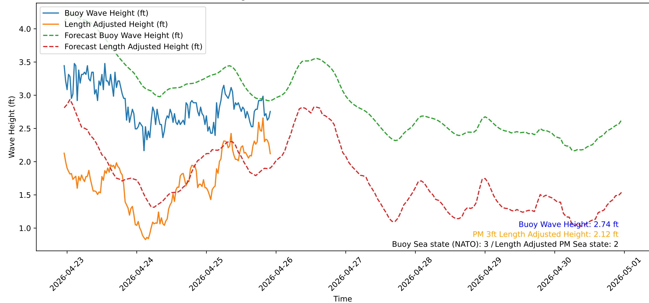
Wave Heights over Time for Red Beach at 2026-04-25 22:40:51
