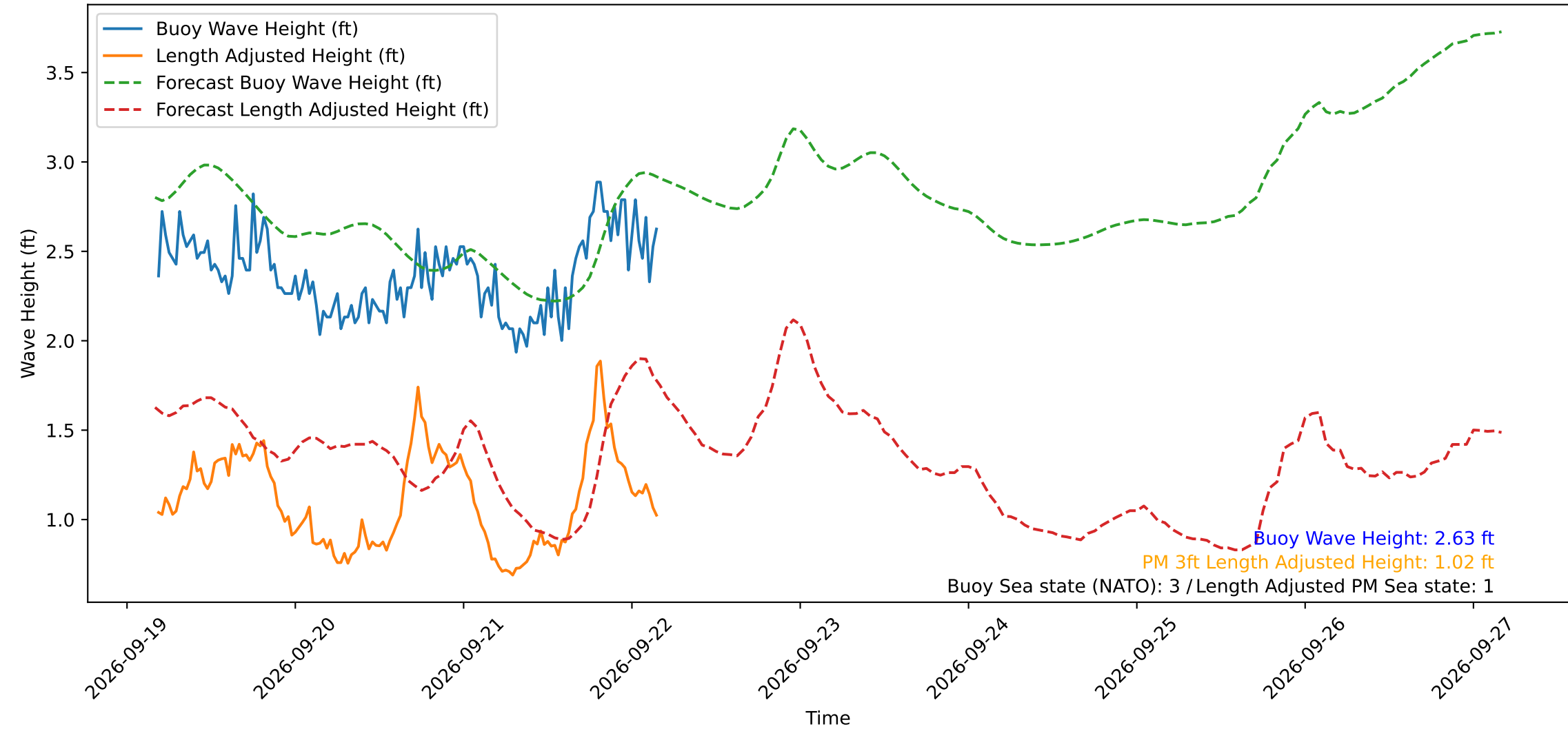
Wave Heights over Time for Red Beach at 2026-09-22 04:20:50
