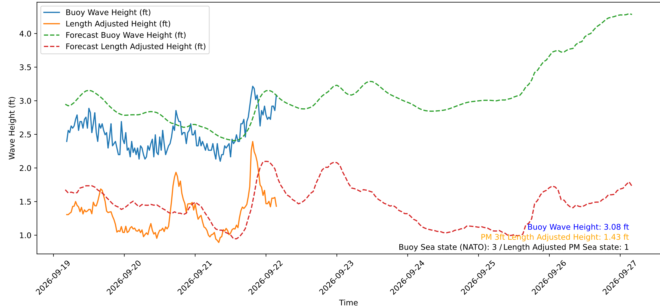
Wave Heights over Time for Oceanside Harbor at 2026-09-22 04:20:30
