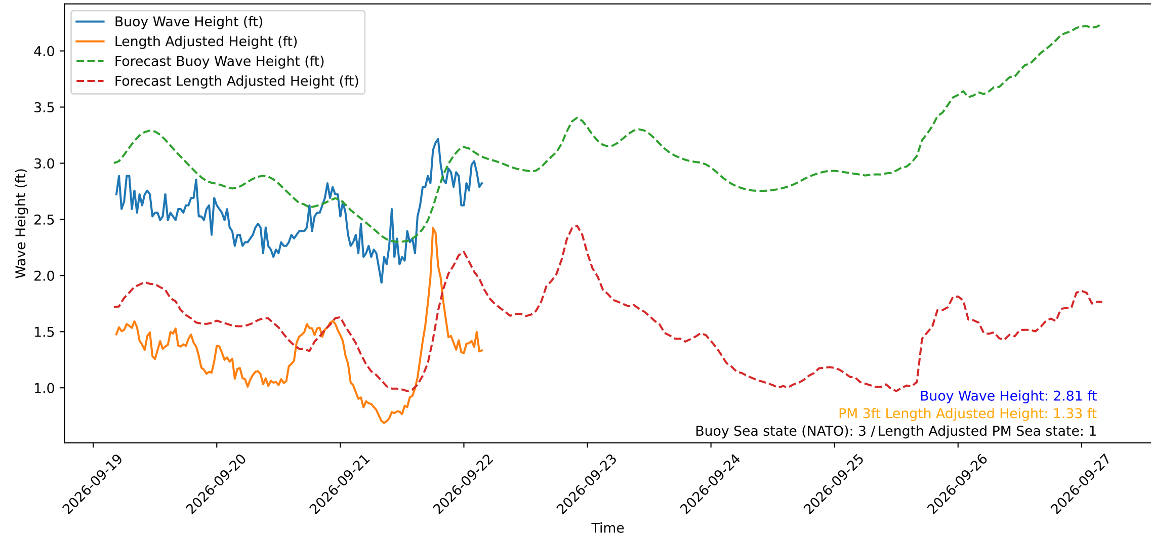
Wave Heights over Time for Green Beach at 2026-09-22 04:21:14
