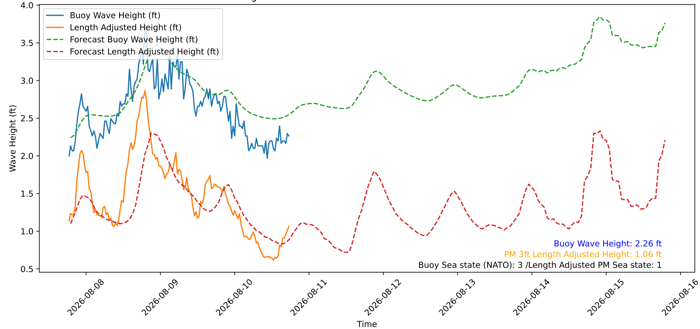
Wave Heights over Time for Green Beach at 2026-08-10 18:31:09
