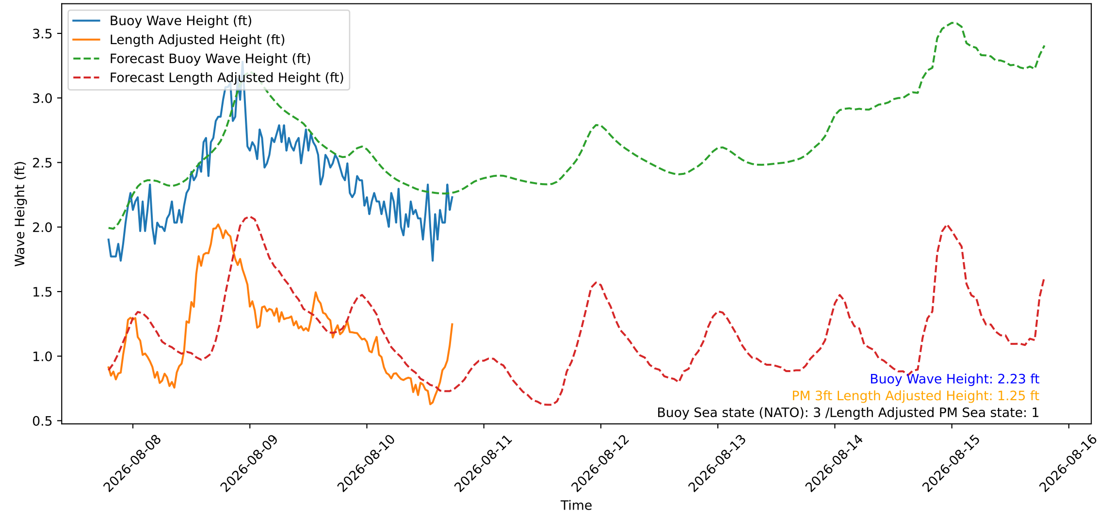
Wave Heights over Time for Red Beach at 2026-08-10 18:30:46
