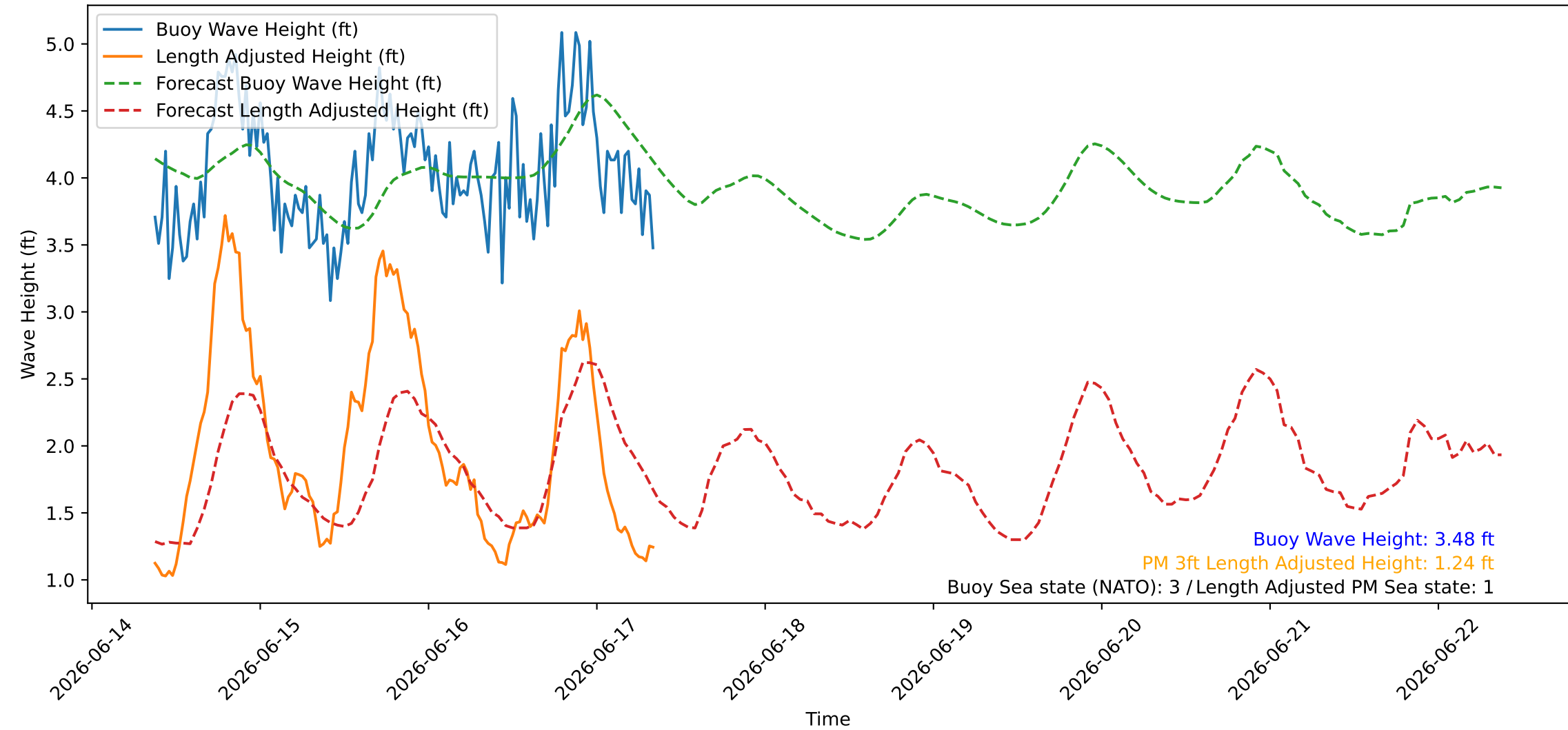
Wave Heights over Time for Green Beach at 2026-06-17 09:01:09
