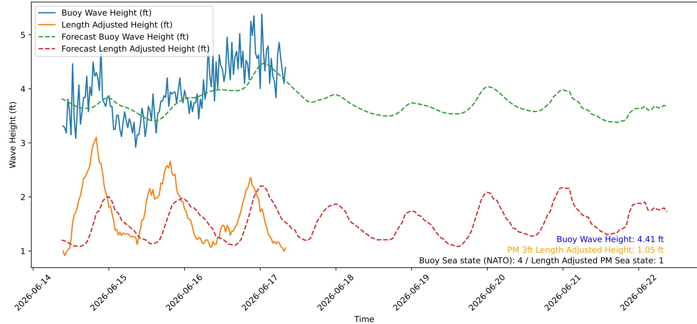
Wave Heights over Time for Red Beach at 2026-06-17 09:00:46
