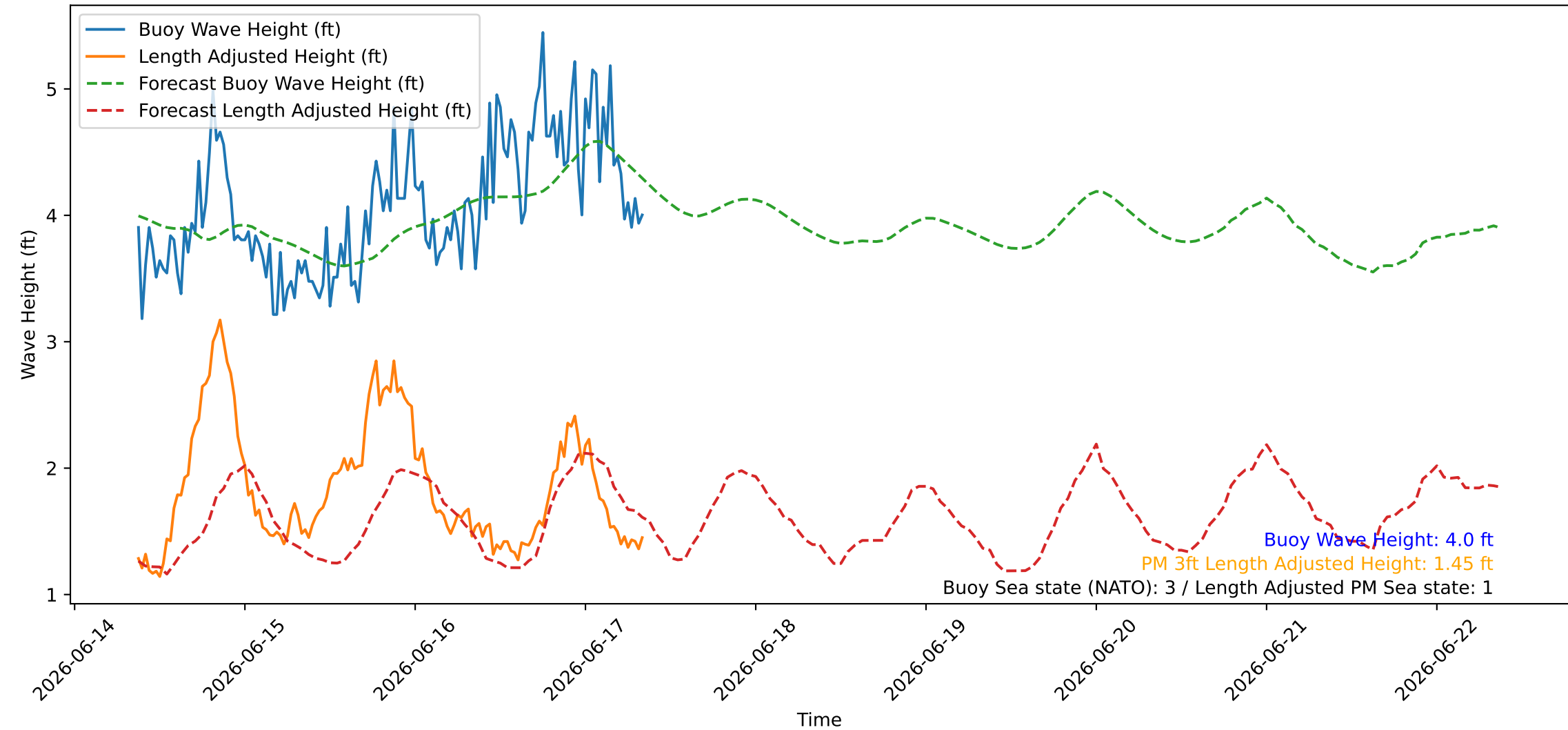
Wave Heights over Time for Oceanside Harbor at 2026-06-17 09:00:27
