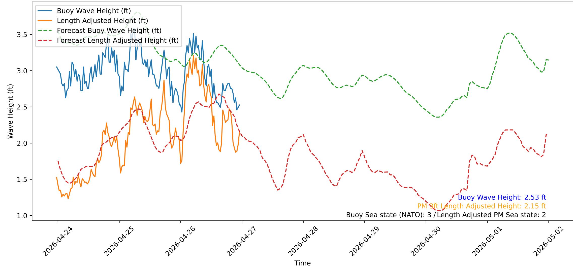
Wave Heights over Time for Green Beach at 2026-04-26 23:41:13
