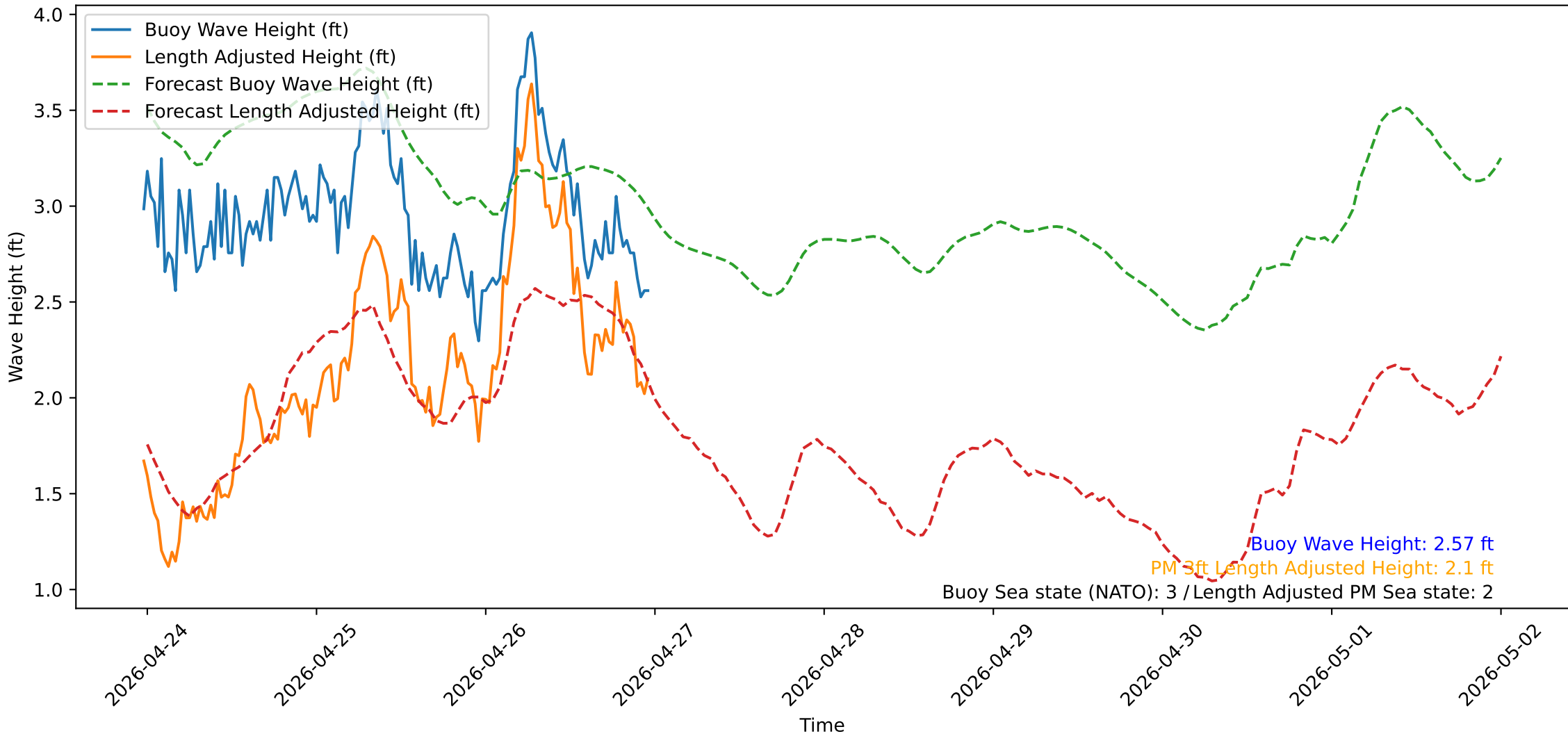
Wave Heights over Time for Oceanside Harbor at 2026-04-26 23:40:31
