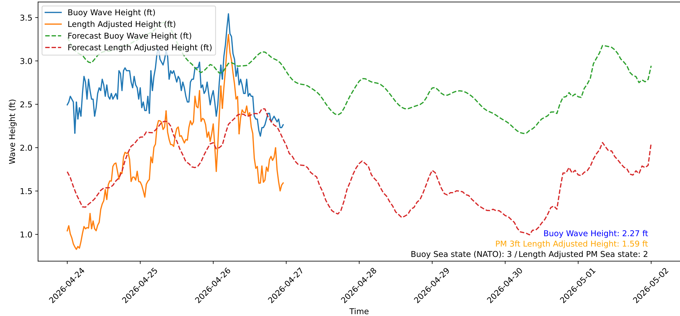
Wave Heights over Time for Red Beach at 2026-04-26 23:40:51
