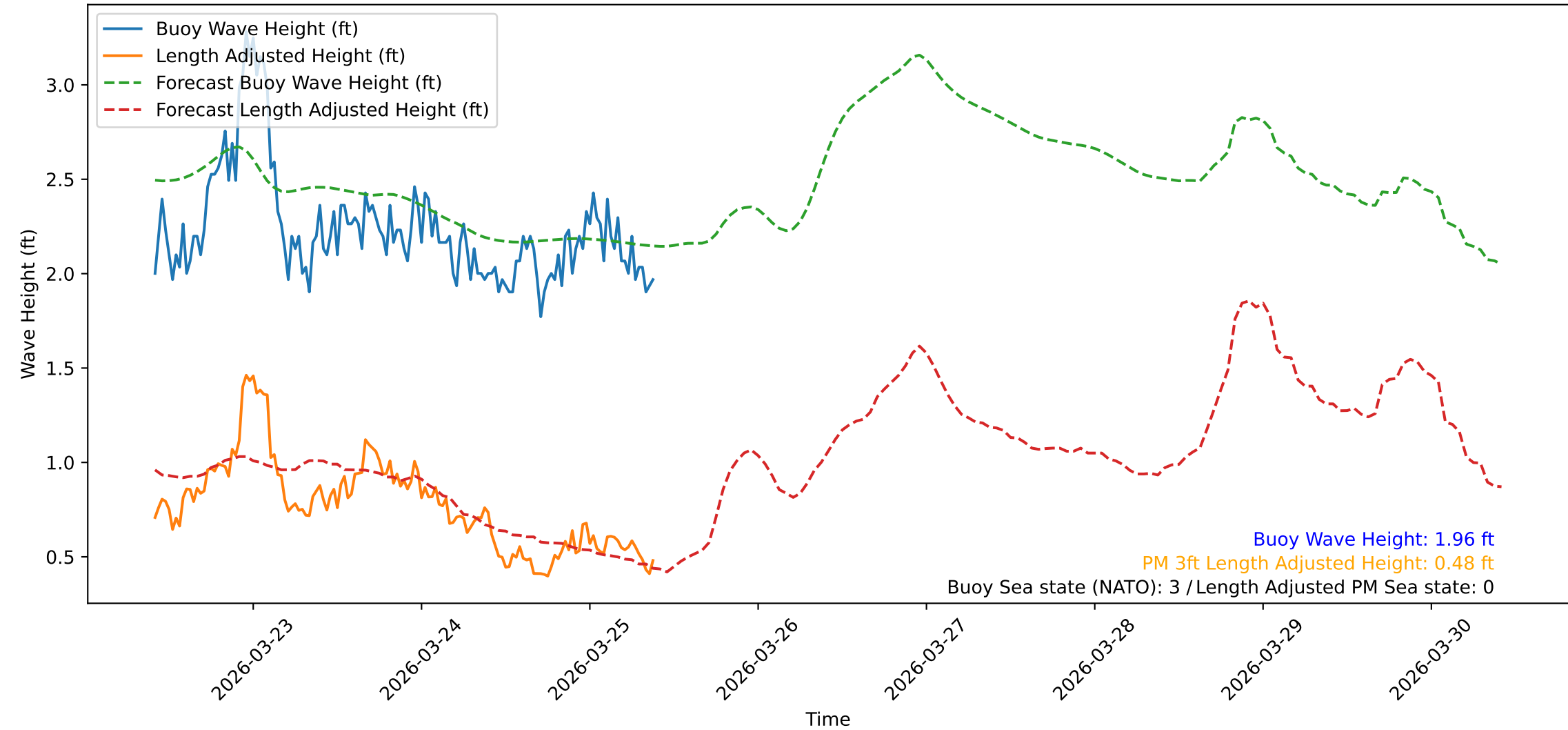
Wave Heights over Time for Green Beach at 2026-03-25 09:51:09
