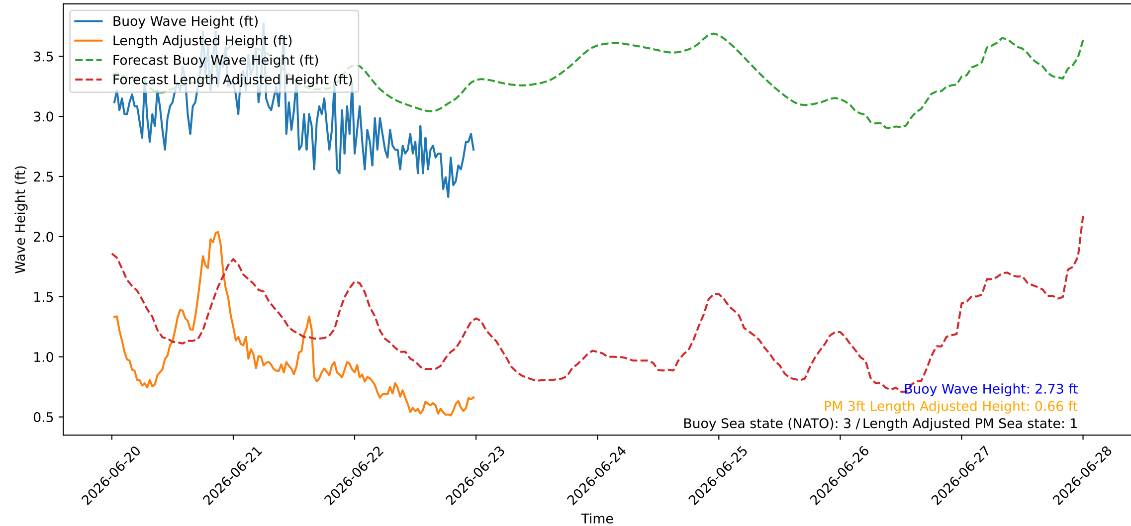
Wave Heights over Time for Red Beach at 2026-06-23 00:20:46
