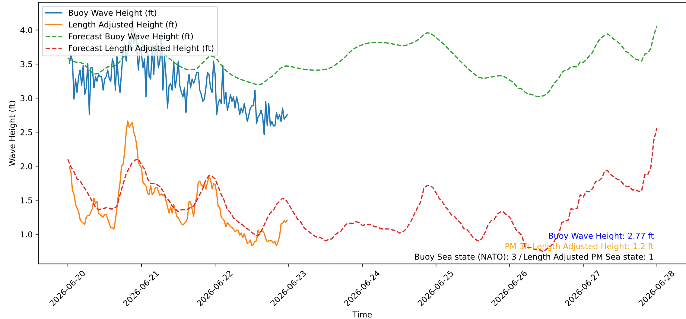
Wave Heights over Time for Green Beach at 2026-06-23 00:21:09
