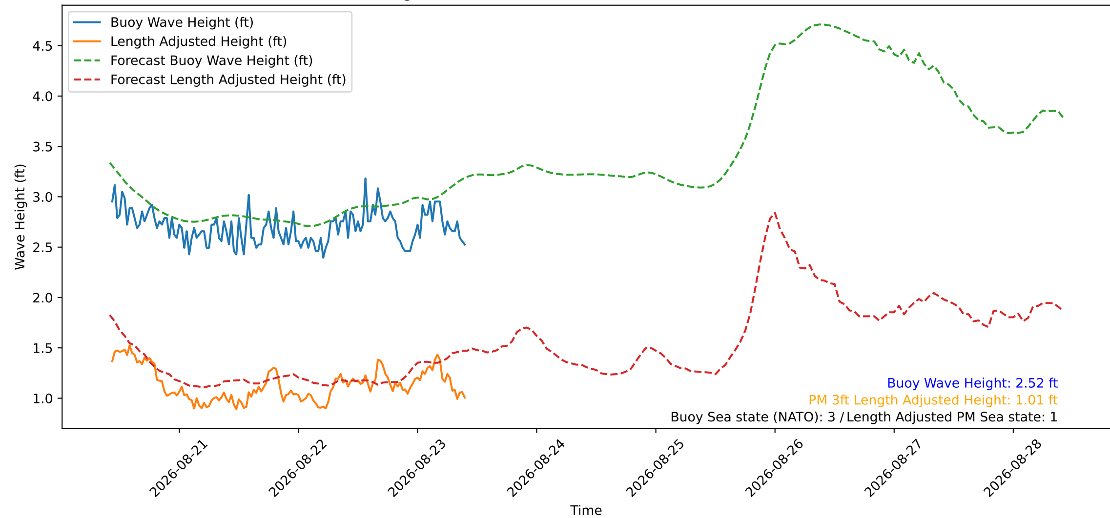
Wave Heights over Time for Green Beach at 2026-08-23 10:11:11
