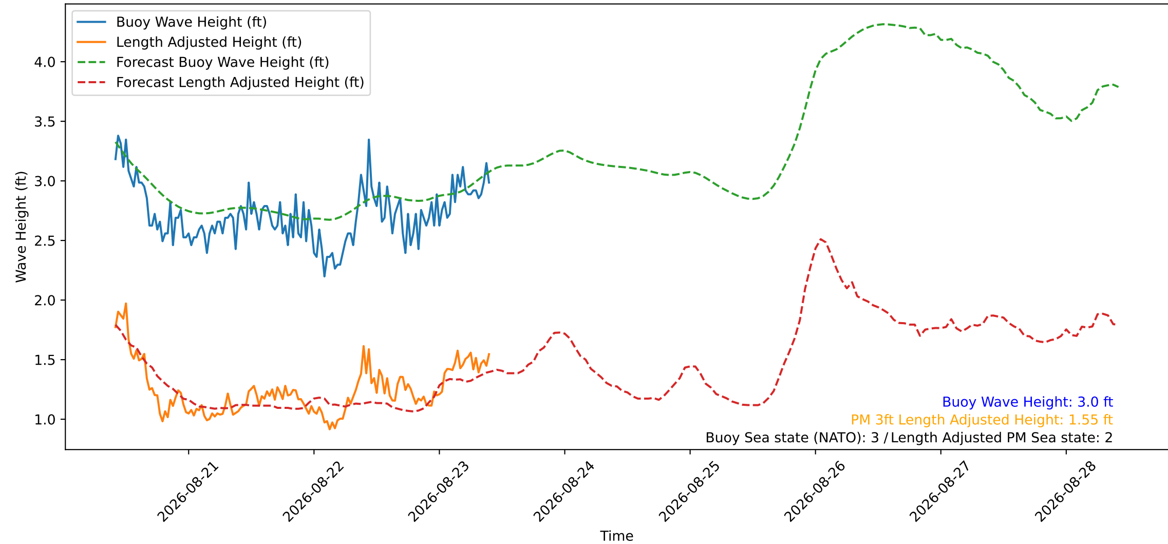
Wave Heights over Time for Oceanside Harbor at 2026-08-23 10:10:29
