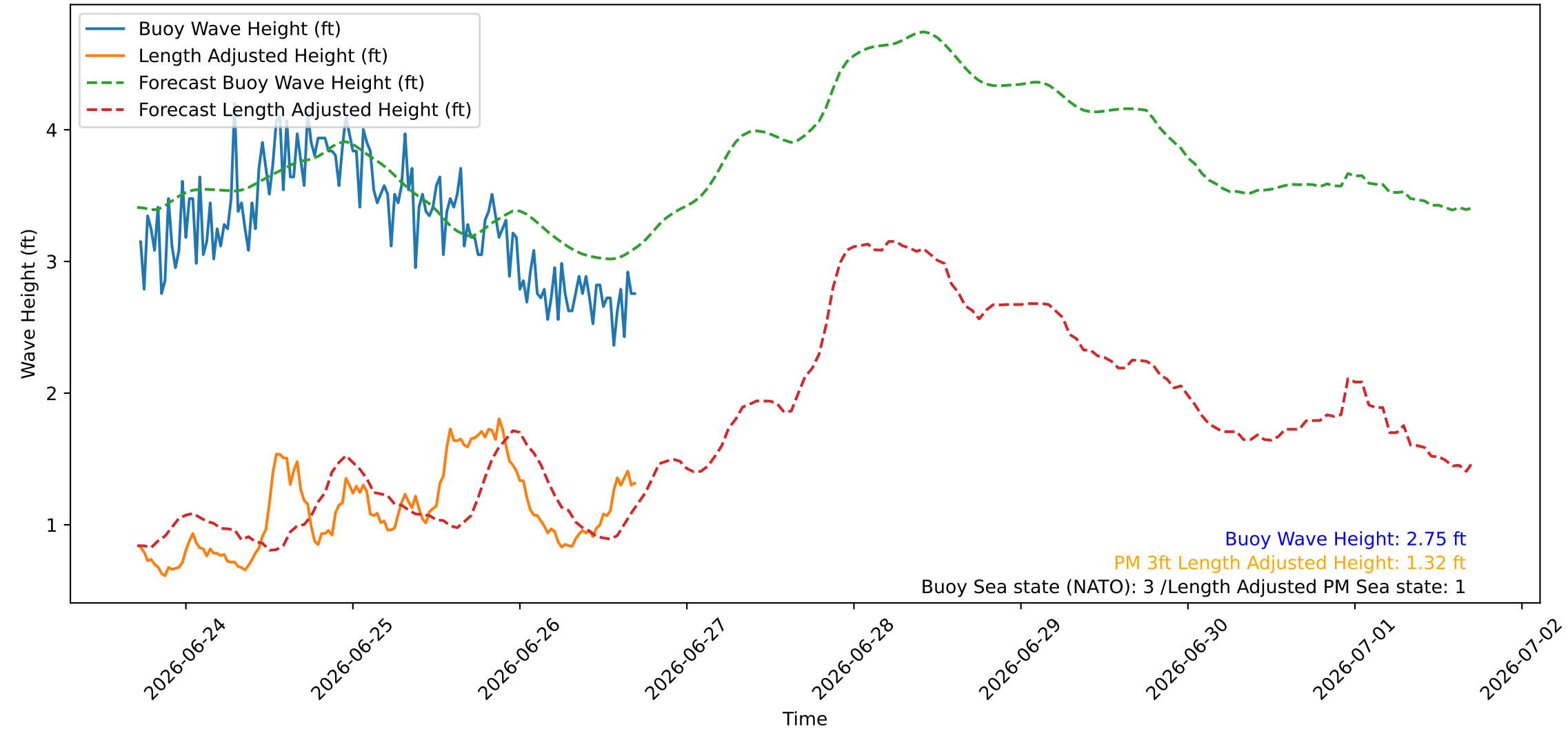
Wave Heights over Time for Green Beach at 2026-06-26 17:21:09
