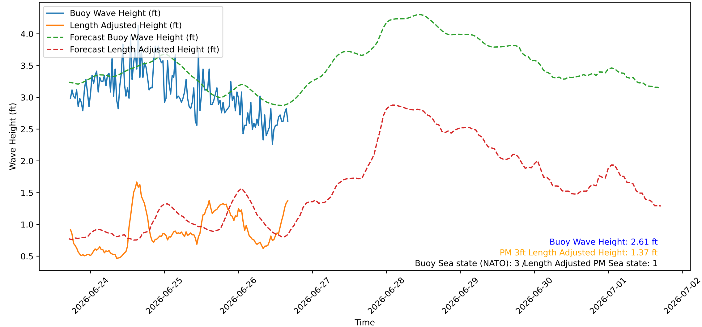
Wave Heights over Time for Red Beach at 2026-06-26 17:20:46
