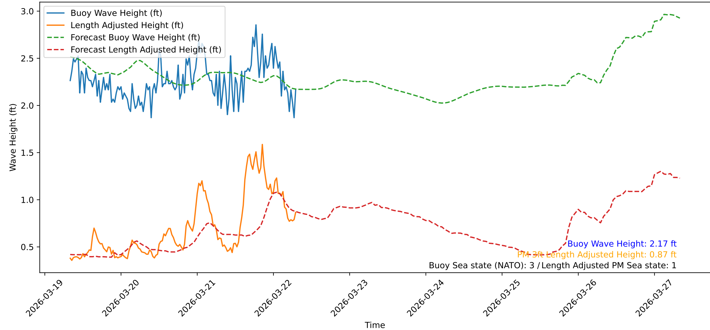
Wave Heights over Time for Red Beach at 2026-03-22 07:40:46
