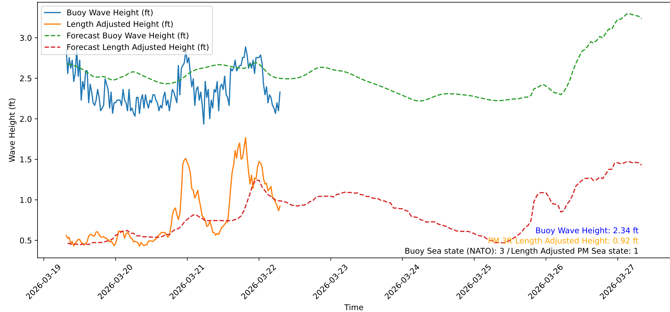
Wave Heights over Time for Green Beach at 2026-03-22 07:41:09
