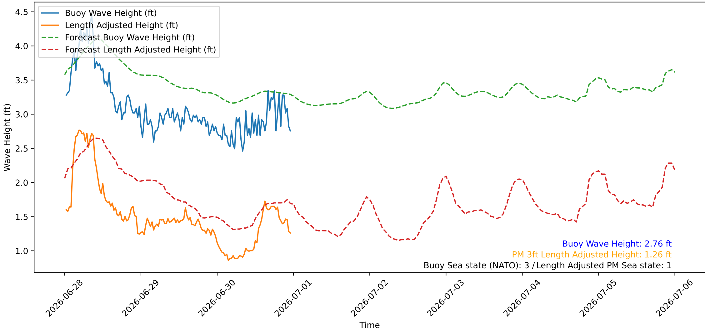
Wave Heights over Time for Red Beach at 2026-07-01 00:00:46
