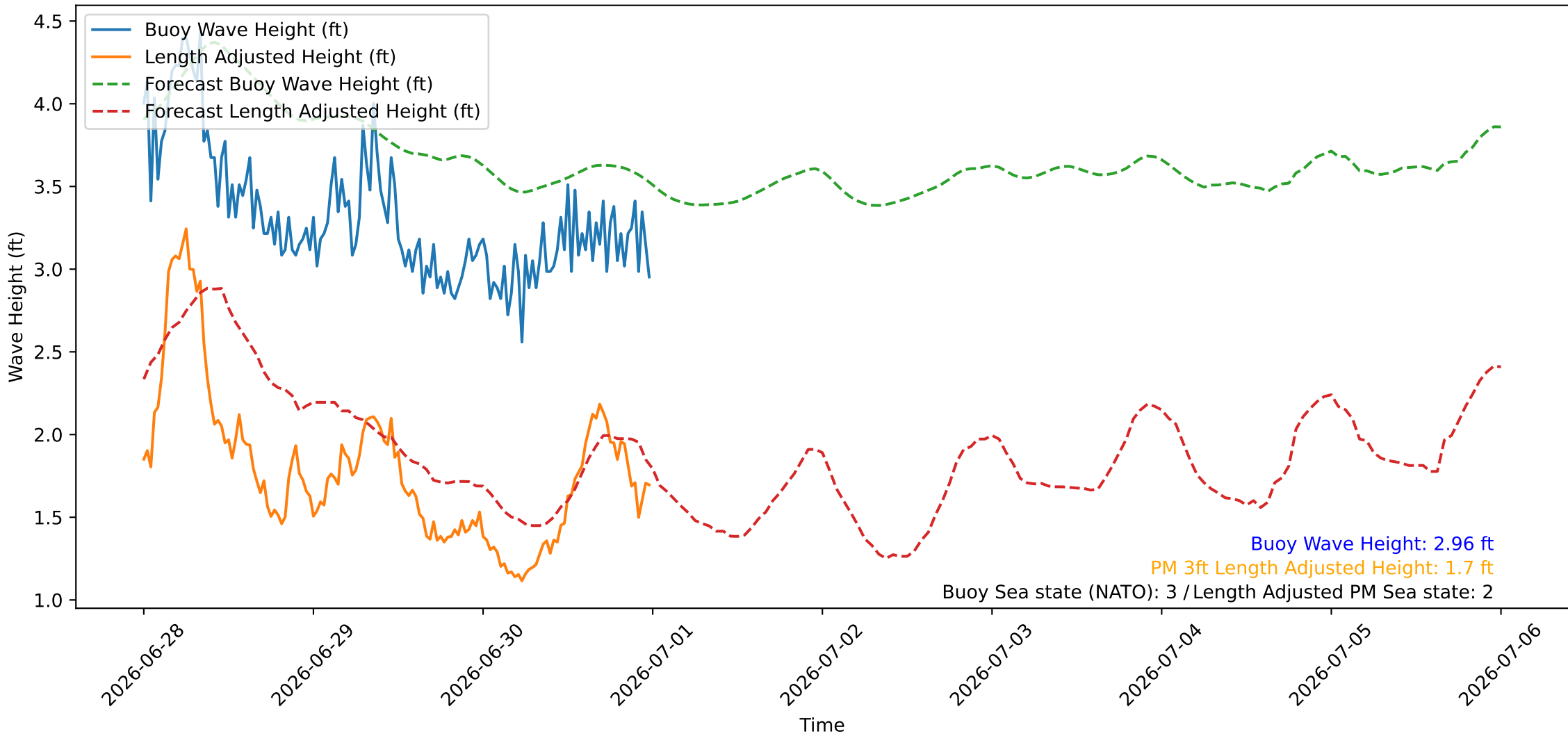
Wave Heights over Time for Oceanside Harbor at 2026-07-01 00:00:26
