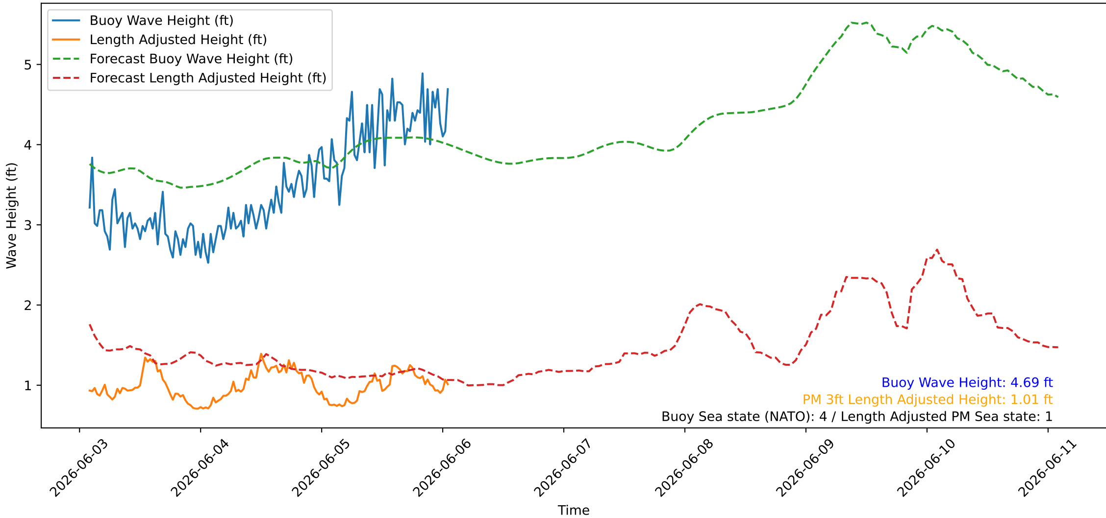
Wave Heights over Time for Red Beach at 2026-06-06 01:40:46
