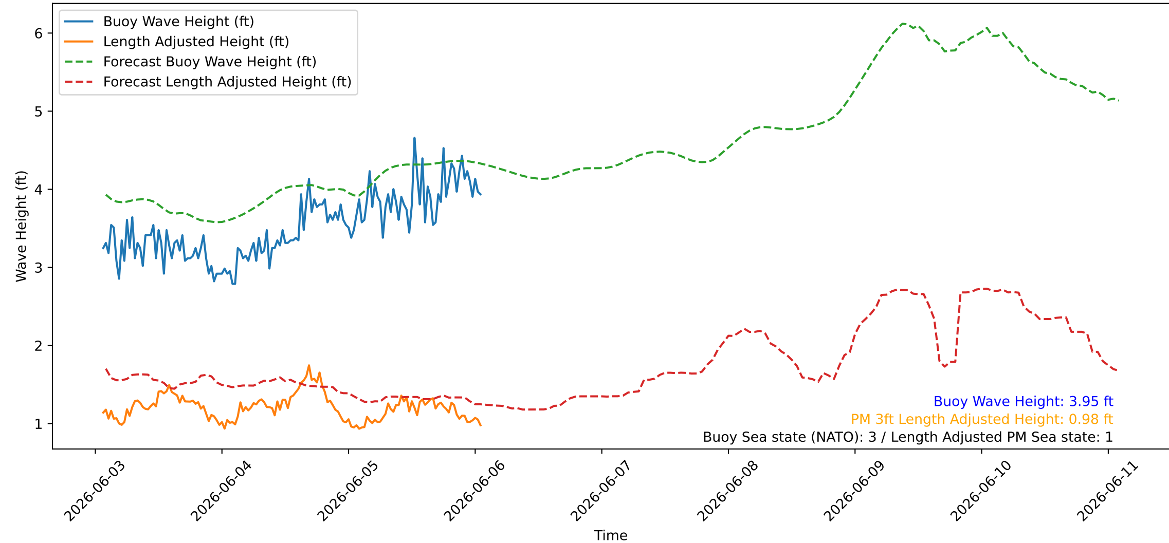
Wave Heights over Time for Green Beach at 2026-06-06 01:41:09
