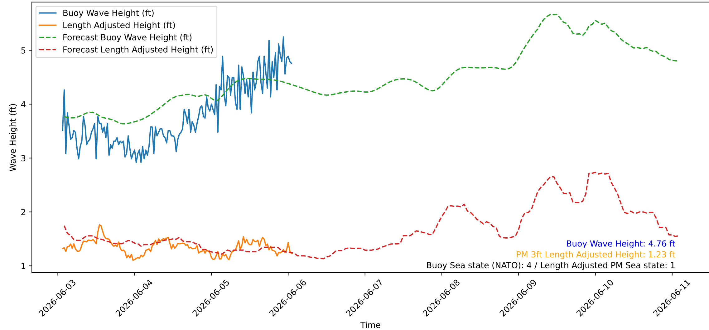
Wave Heights over Time for Oceanside Harbor at 2026-06-06 01:40:27
