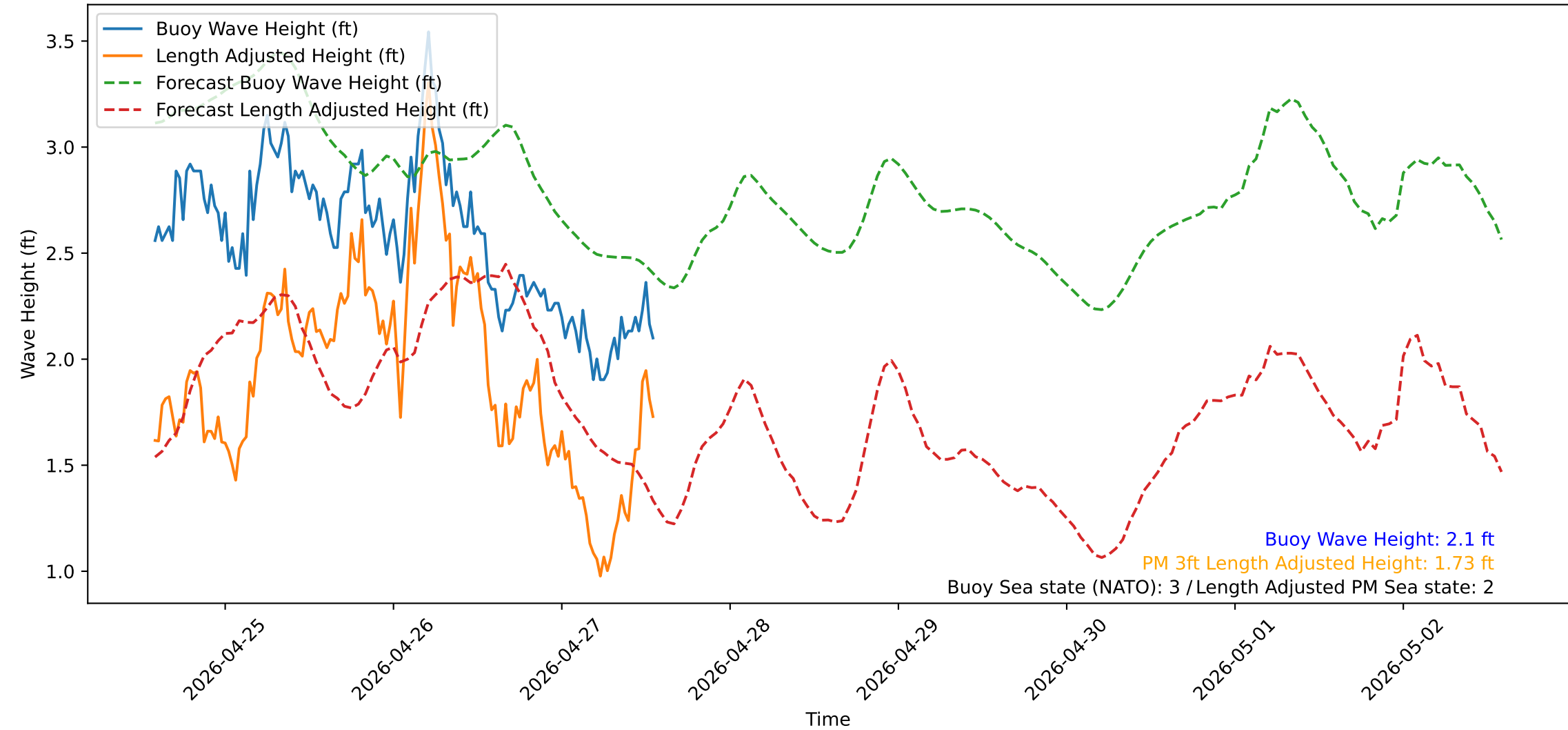
Wave Heights over Time for Red Beach at 2026-04-27 13:40:50
