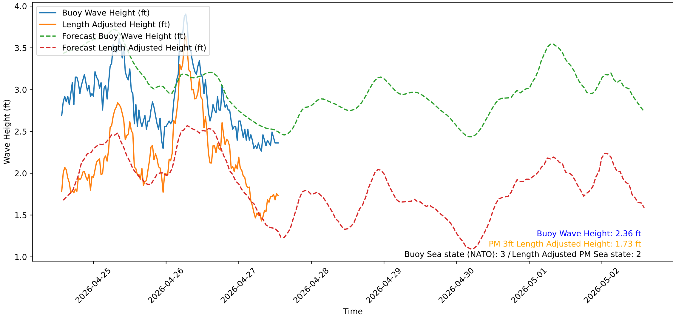
Wave Heights over Time for Oceanside Harbor at 2026-04-27 13:40:31
