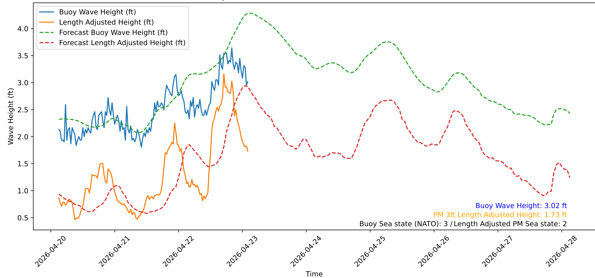
Wave Heights over Time for Red Beach at 2026-04-23 02:50:51
