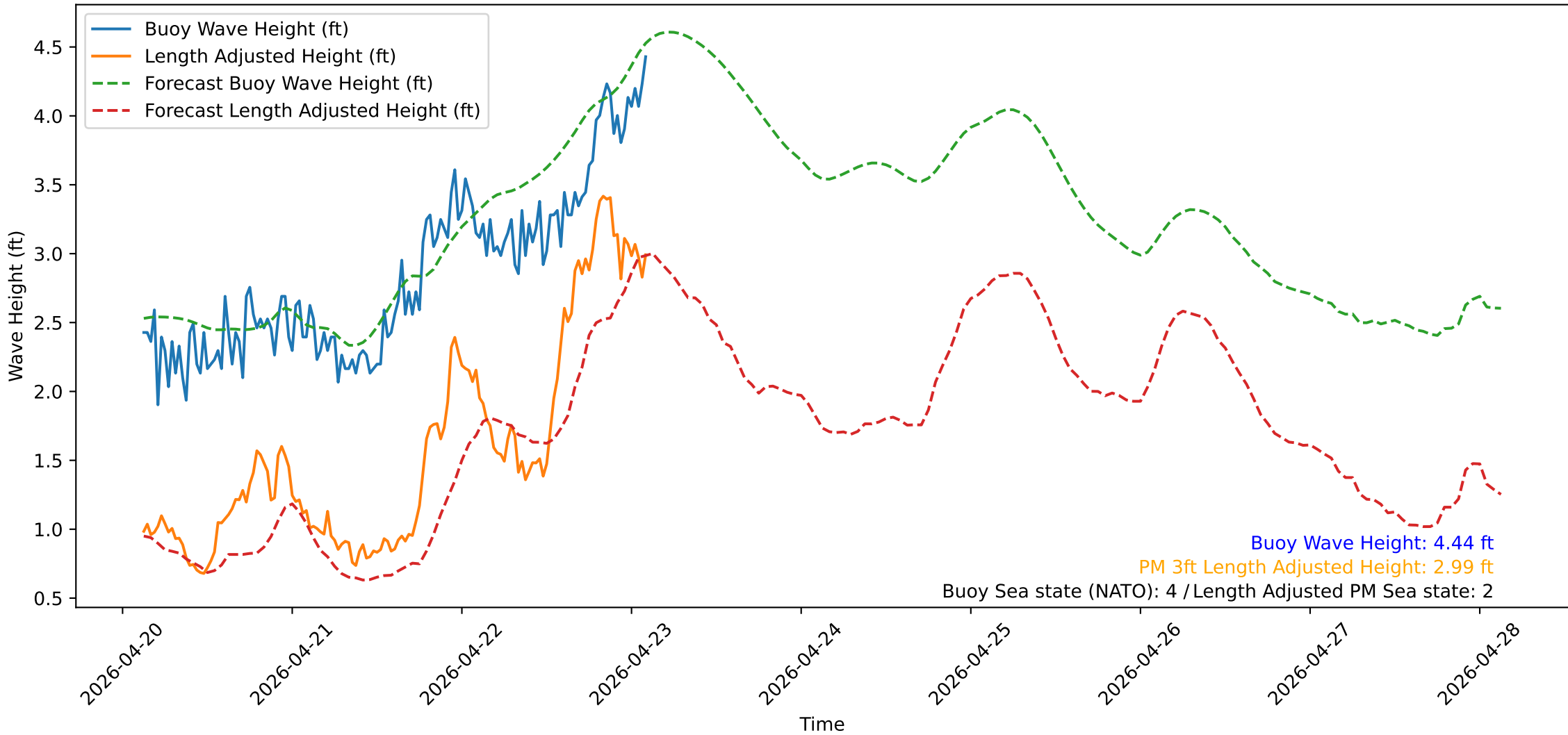
Wave Heights over Time for Oceanside Harbor at 2026-04-23 02:50:30
